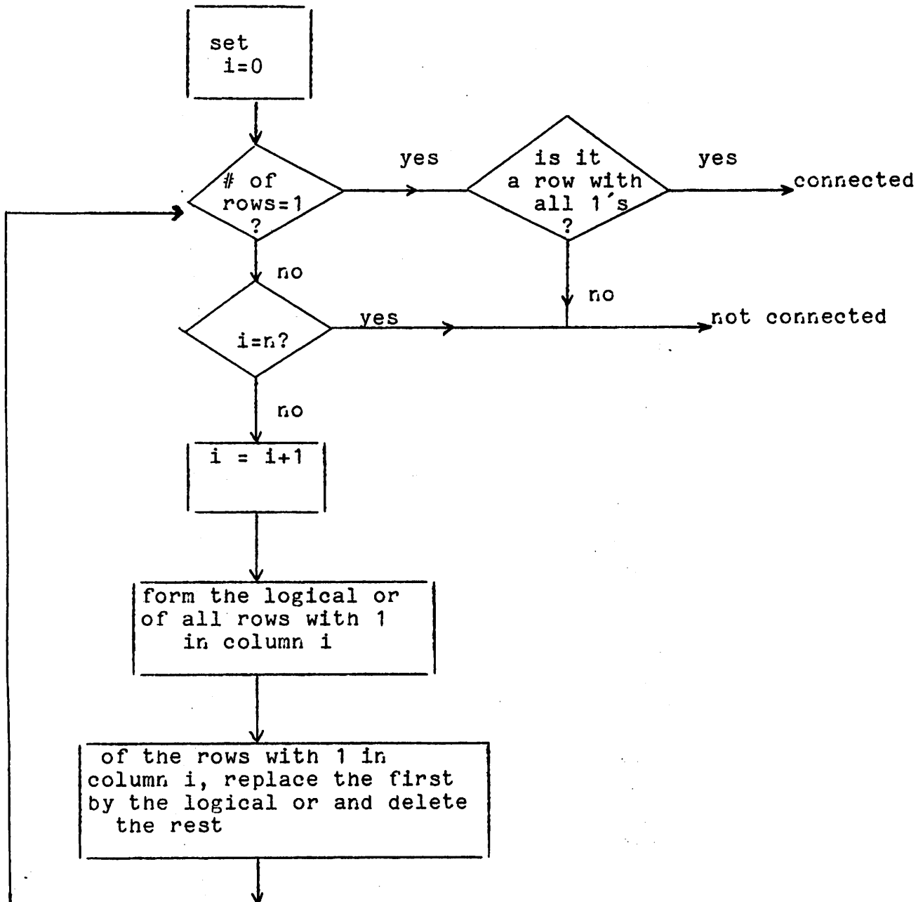
Figure 4.2 Connectivity
