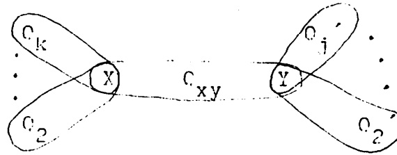
Figure 4.3 Joining-Variables
