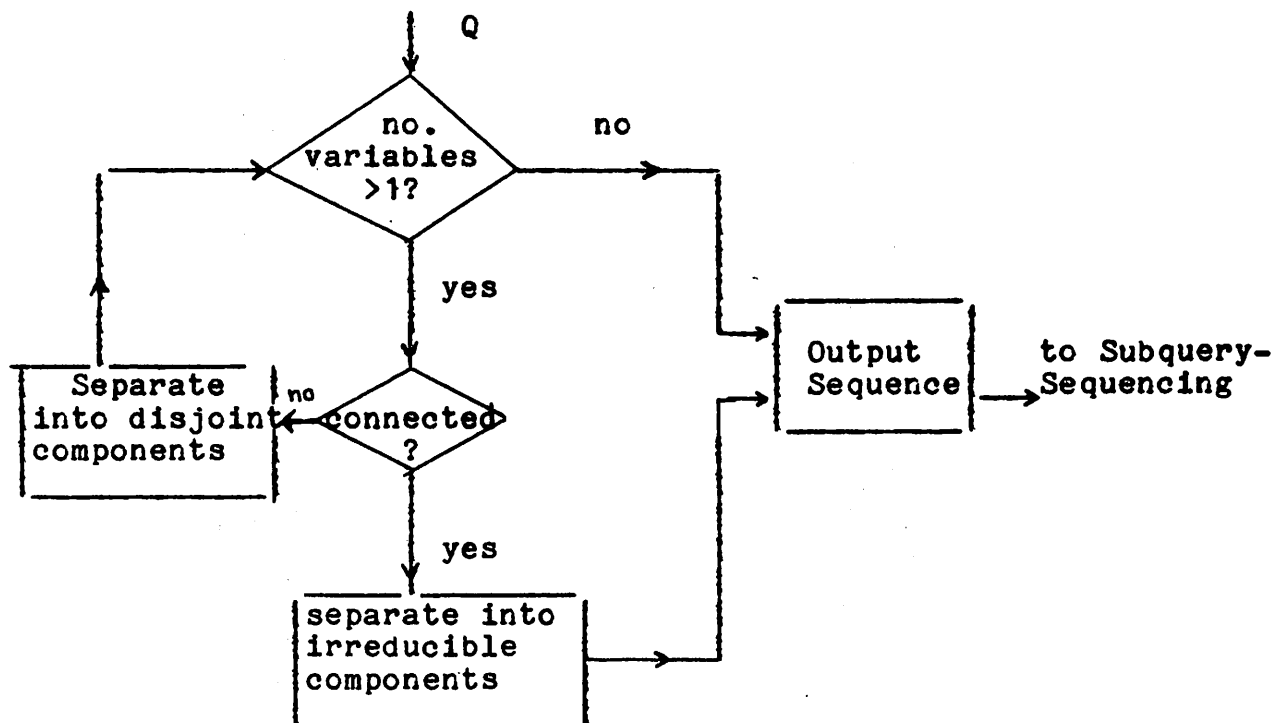
Figure 4.1 Reduction Algorithm
