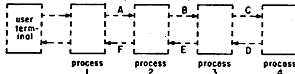
Fig. 1. INGRES process structure
