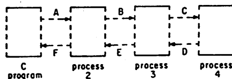
Fig. 2. The forked process structure
