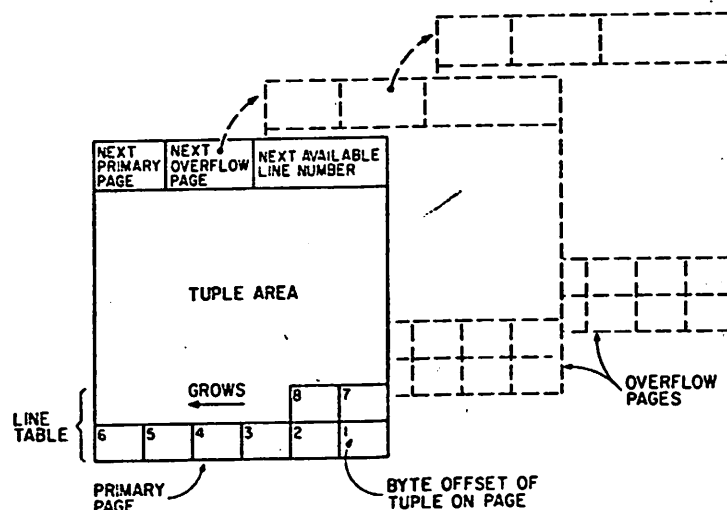
Fig. 4. Page layout for keyed storage structures
