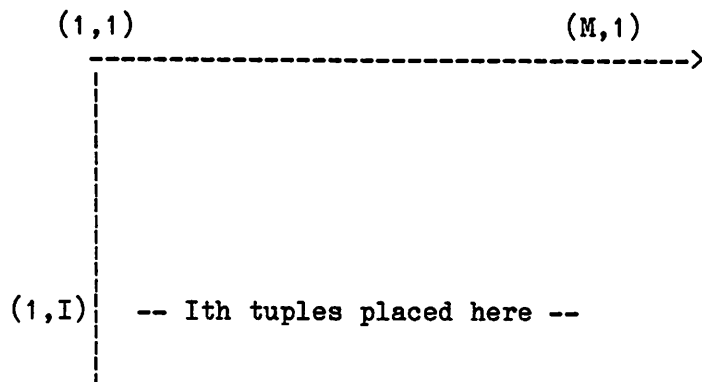
Relation Space for Fixed Format Relations
