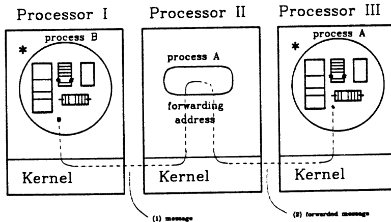
Message sent through a forwarding address Figure 4-1
