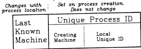
Structure of a process address Figure 2-1
