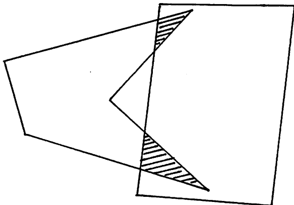
Fig. 1.1: The intersection of two simple polyhedra is not necessarily a simple polyhedron.
