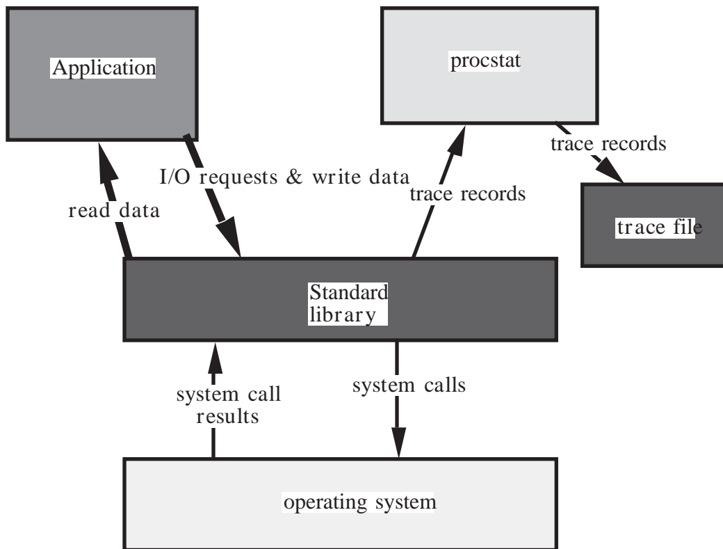
Figure 2. Trace information flow between software modules.
