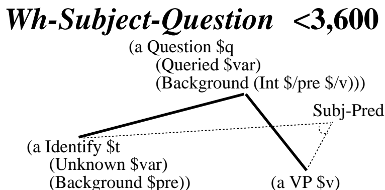
Figure 6.19: The Wh-Subject-Question Construction
