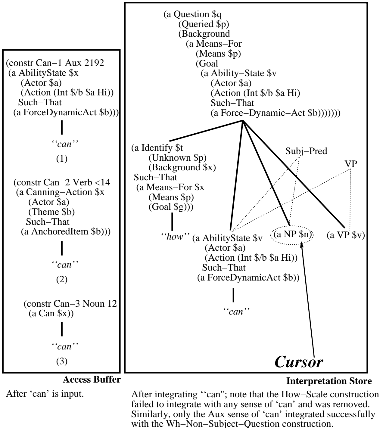
Figure 4.9: Accessing and Integrating "can"
