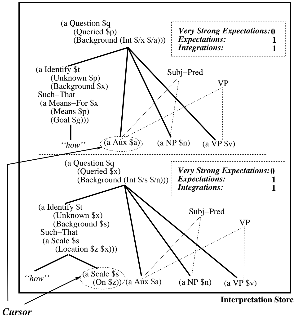
Figure 4.8: After Integrating "how" with the Wh-Non-Subject-Question Construction. Two more interpretations are not shown (see text).
