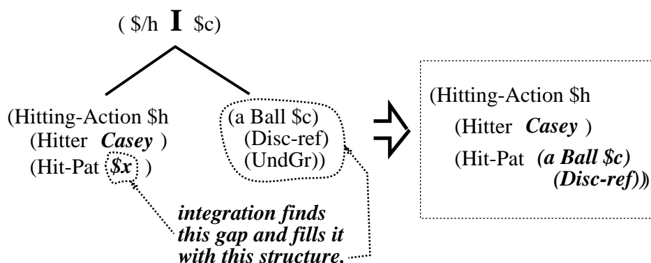
Figure 6.12: Interpreting "Casey hit the ball (2)"
