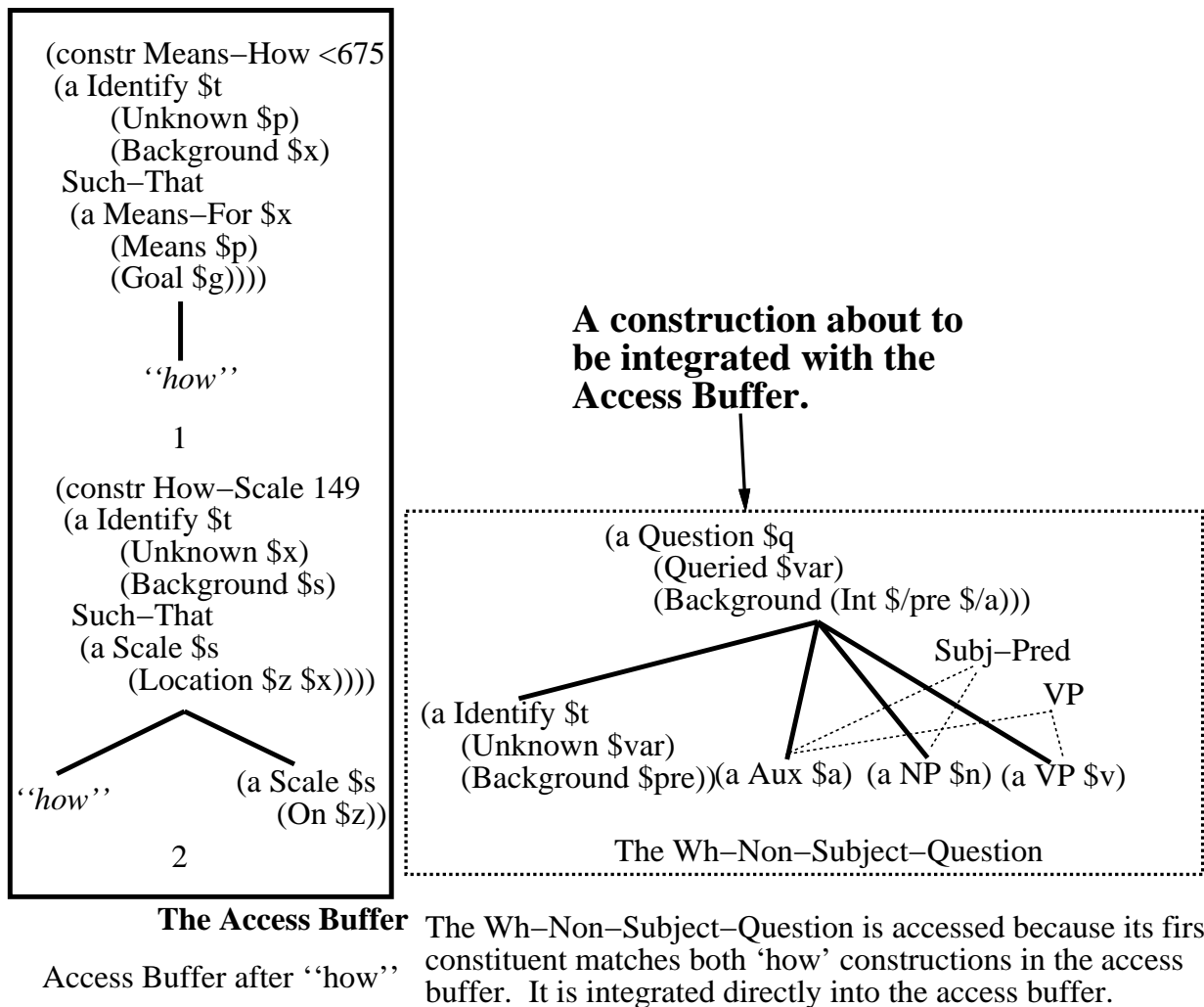
Figure 4.7: The access buffer after "how"
