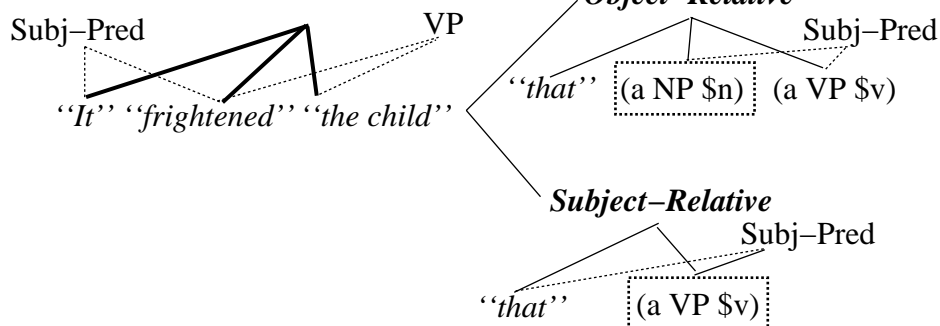
Figure 7.8: Processing an Extrapolation (2): The Interpretation Store after that
