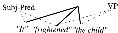
Figure 7.7: Processing an Extrapolation (1): The Interpretation Store after child
