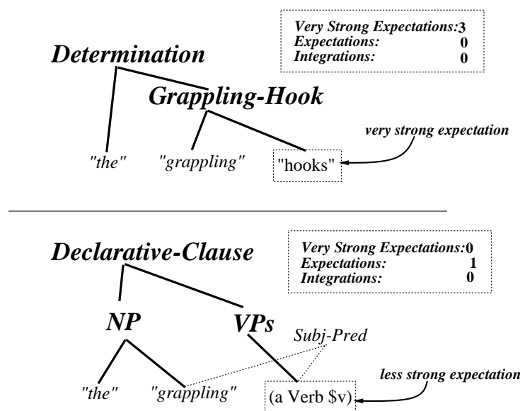
Figure 7.3: Two Interpretations before seeing “hooks”
