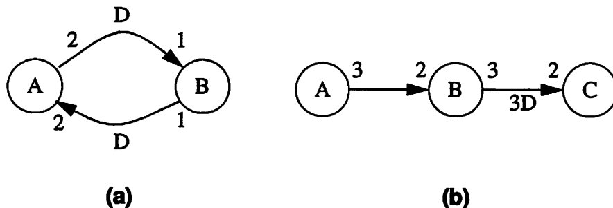
Fig 3. Examples that illustrate distinctions between iteration and looping in SDF.
