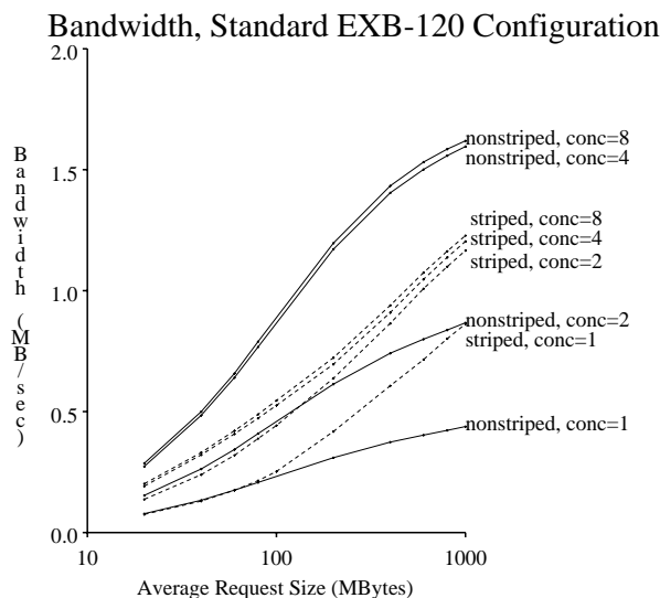
Figure 6: Bandwidth comparison of striped system with interleave unit of 100 MBytes to a non-striped system, for concurrencies of 1, 2, 4 and 8. Standard Exabyte configuration.
