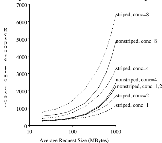
Response time, Standard EXB-120 Configuration
