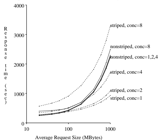
Response Time, EXB-120 with Eight Readers
