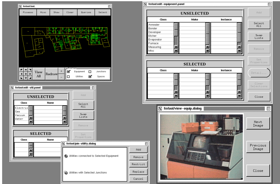
Figure 1: CIMTOOL screendump
