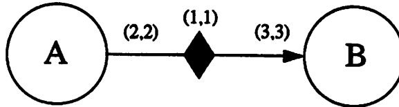
FIGURE 30. A MDSDF system with a two-dimensional delay.
