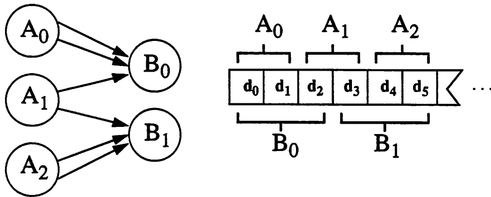
FIGURE 9. Precedence graph and data distribution for system of Figure 8.
