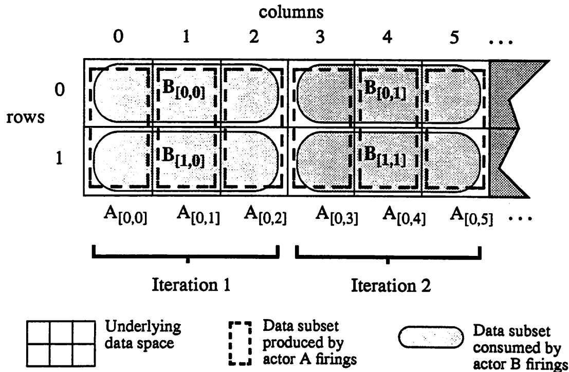
FIGURE 5. The data space for the system of Figure 4
