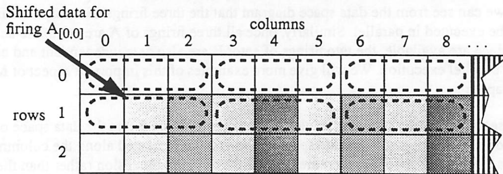
FIGURE 7. A MDSDF system with a two-dimensional delay.
