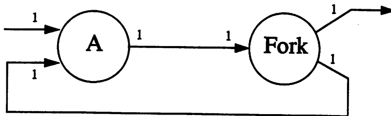
FIGURE 25. A SDF system with a deadlock condition.
