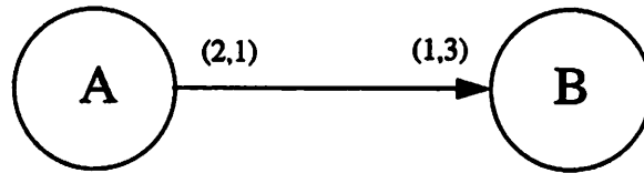
FIGURE 4. A MDSDF extension of the universe in Figure 1.
