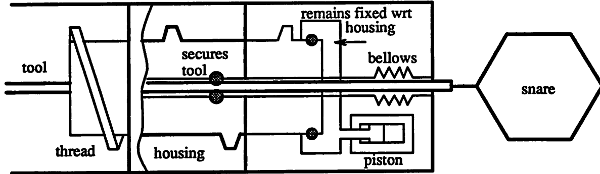
Figure 9: Rotary Screw Actuator
