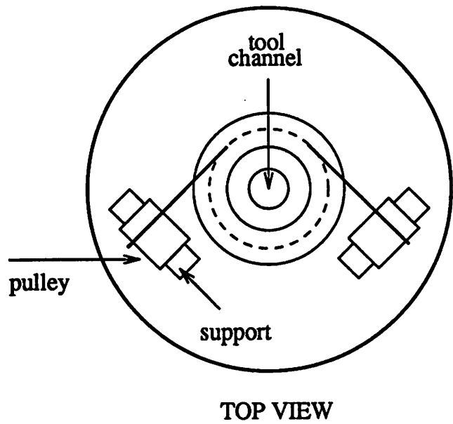
Figure 10: Rotary Pulley Actuator
