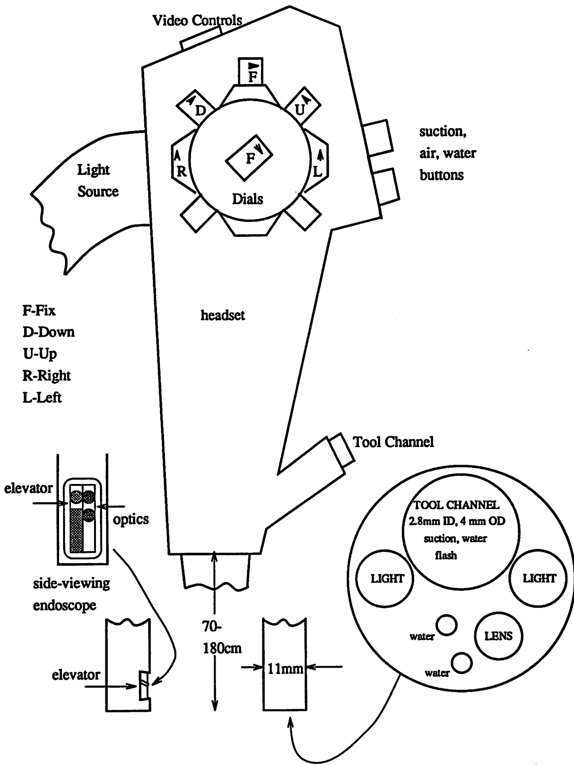
Figure 1: Design of Typical Flexible Endoscopes
