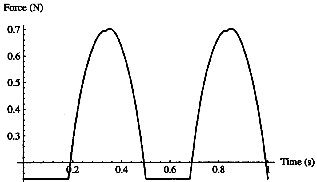
Figure 30: Force in Tendon C for Circle Trajectory
