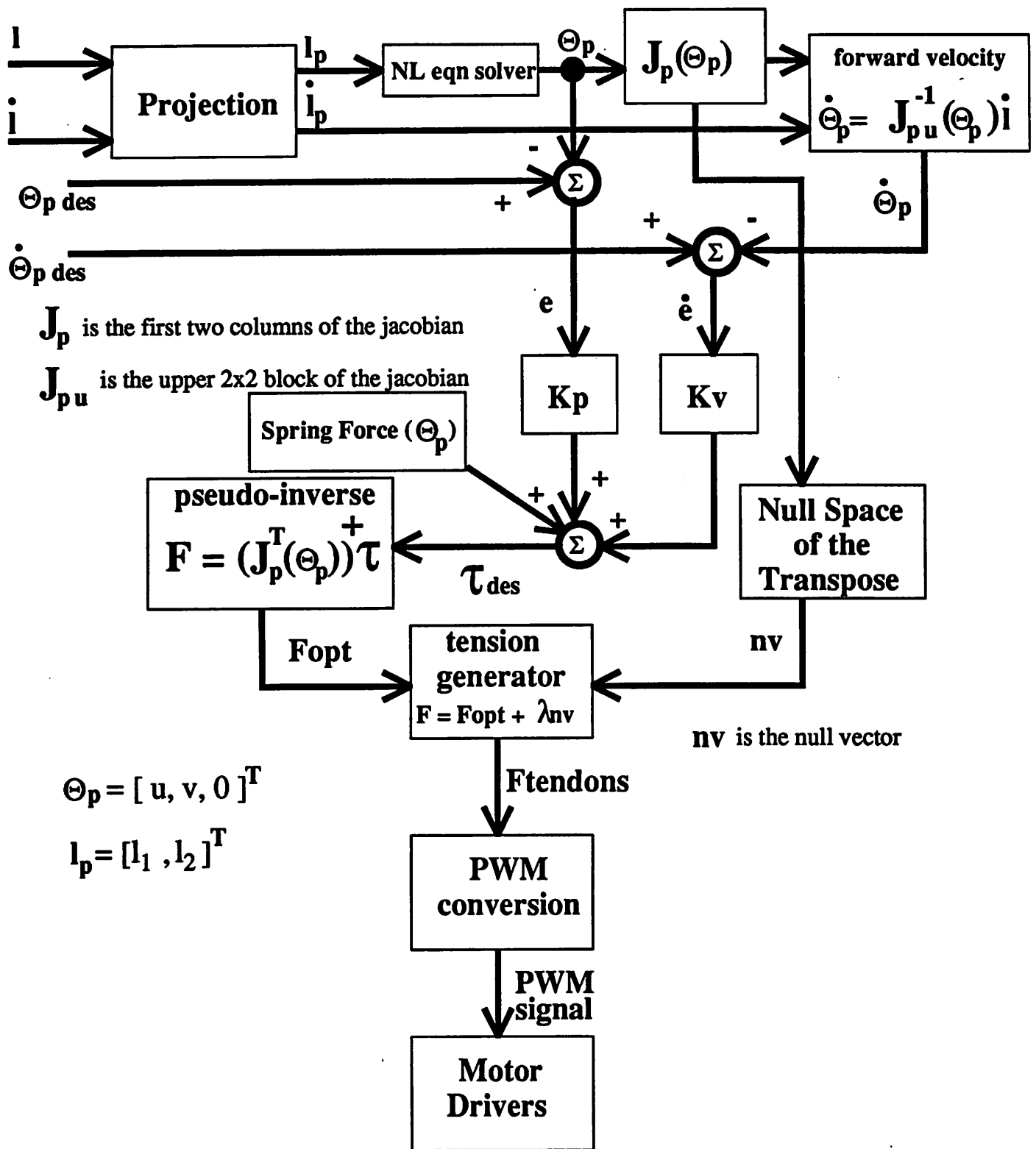
Figure 17: Control Algorithm Diagram
