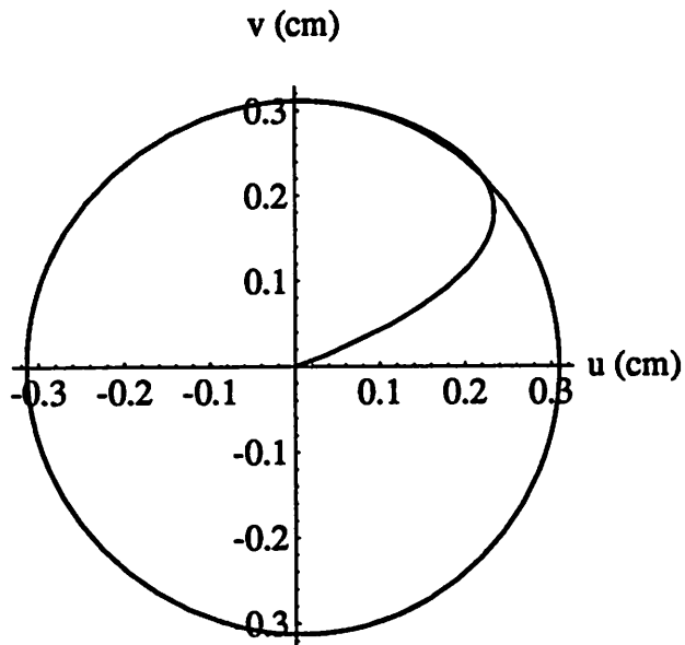
Figure 24: Circle Trajectory
