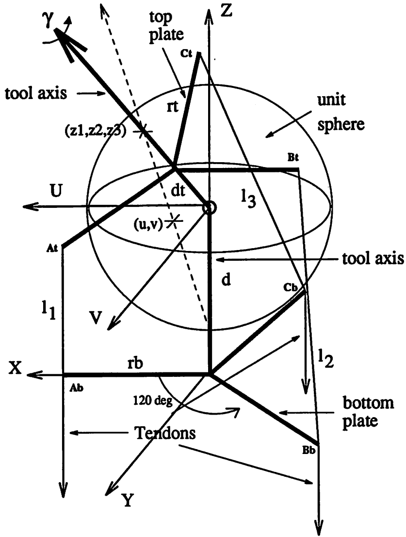
Figure 12: Kinematic Model
