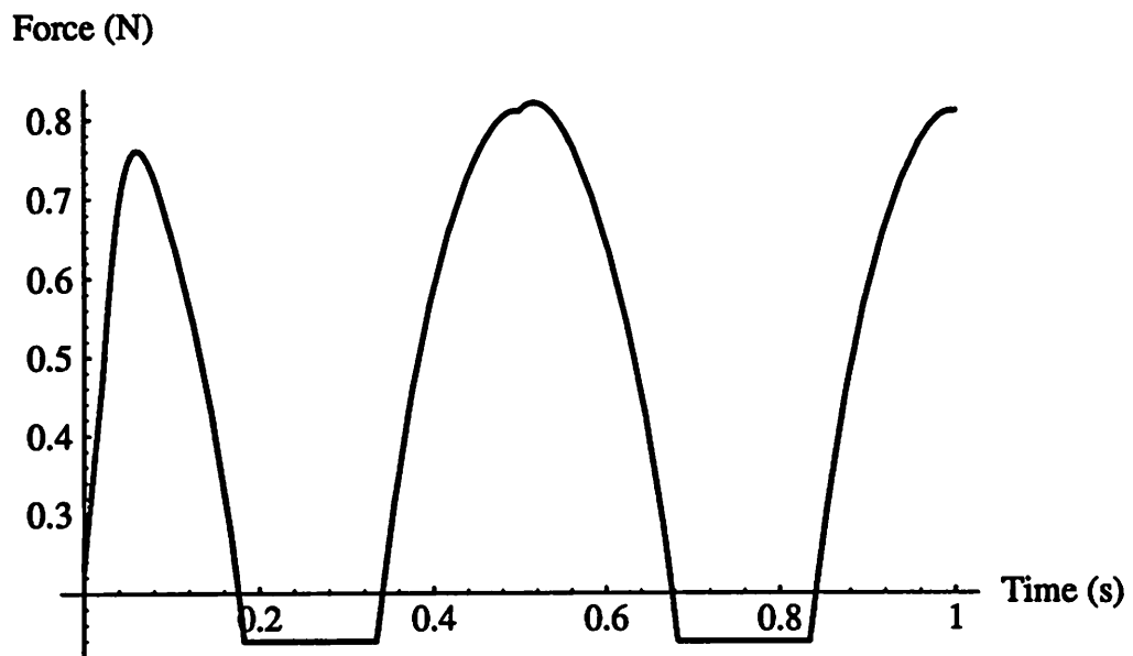
Figure 28: Force in Tendon A for Circle Trajectory
