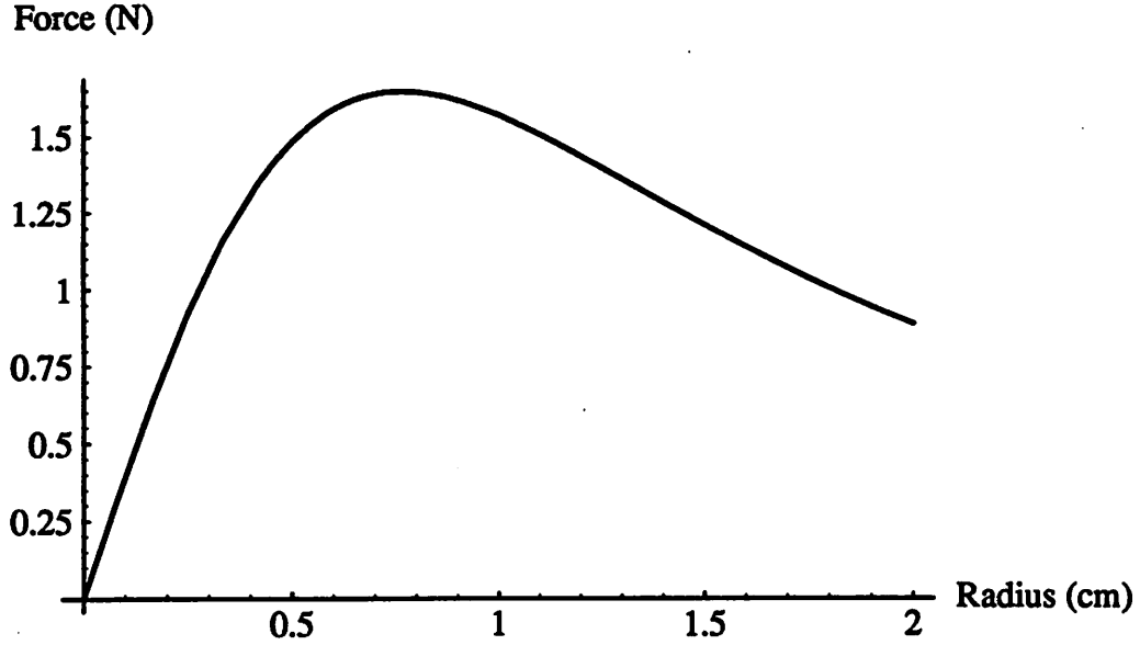
Figure 15: Radial Force
