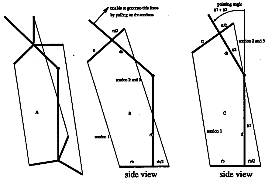
Figure 18: Null Space Geometry
