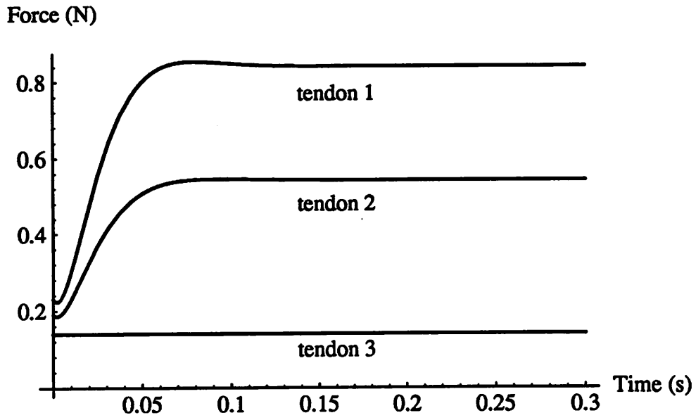
Figure 23: Tendon Force Step Response
