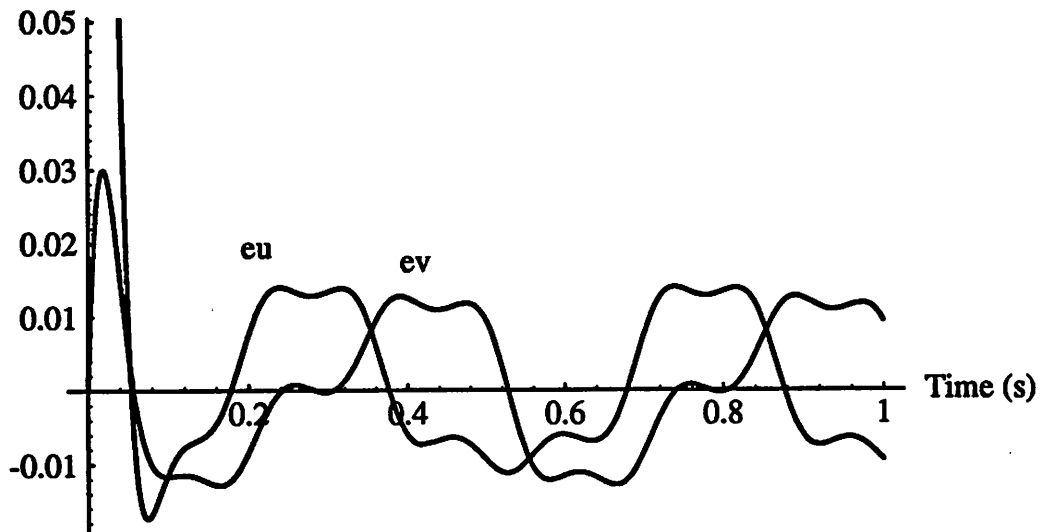
Figure 26: Error Response to Circle Trajectory
