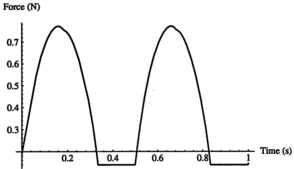
Figure 29: Force in Tendon B for Circle Trajectory
