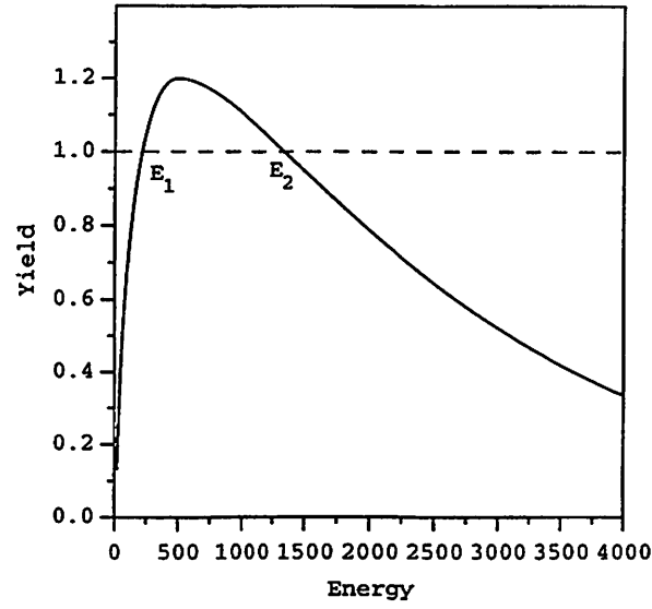
Figure 1: A Typical Metal Secondary Yield vs. Normal Incidence Energy Curve [1]
