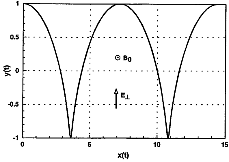
Figure 1.3: E \times B drift
