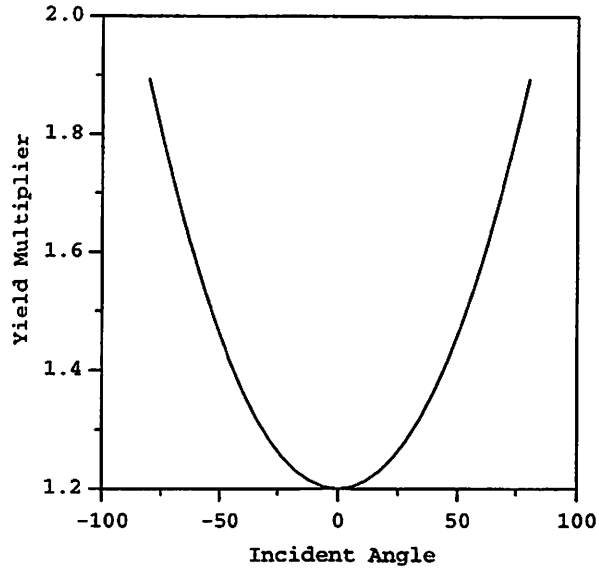
Figure 2: Equation (4) with k' = 0.55
