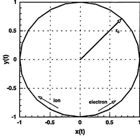
Figure 1.1: Cyclotron motion
