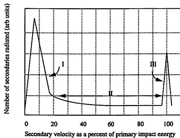
Figure 4: Relative velocity distribution of electrons, adapted from Spangenberg ( [1] fig. 4.17, pg 52).
