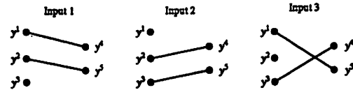
Figure 4. An implementation of F .
