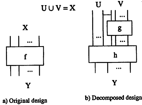
Figure 6. Multi-valued decomposition
