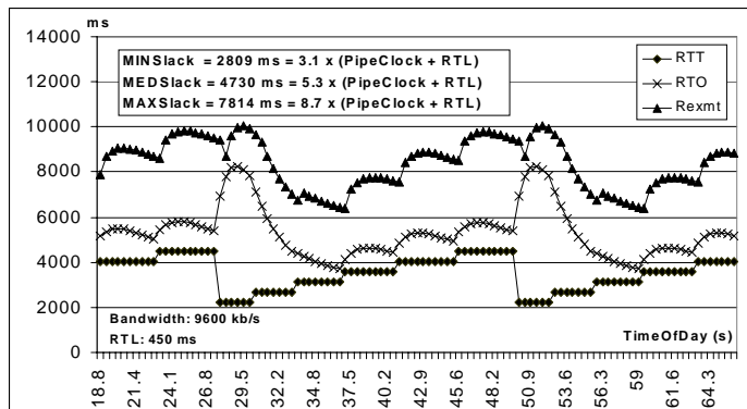
Figure 5: The retransmission timer in steady state.
