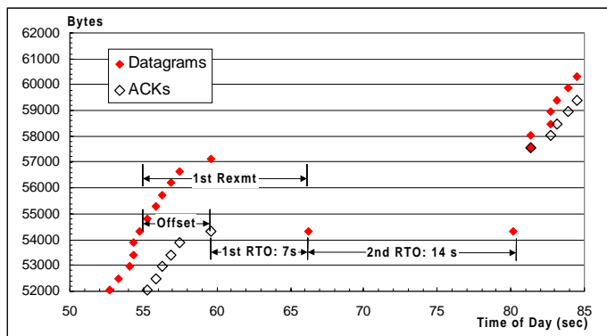
Figure 3: The RTO is not the retransmission timer.
