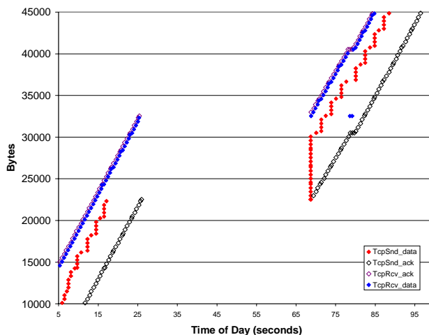
Figure 8: Spurious timeout detection (TCP-Eifel) at work.
