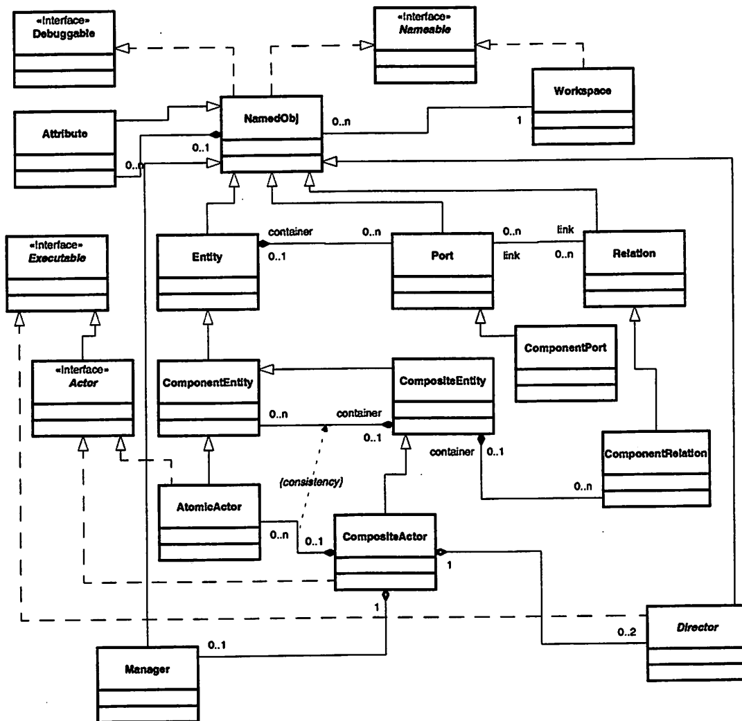
FIGURE 5. Some of the key classes in Ptolemy II. These are defined in the kernel , kernel.util , and actor packages. They define the Ptolemy II abstract syntax and abstract semantics.
