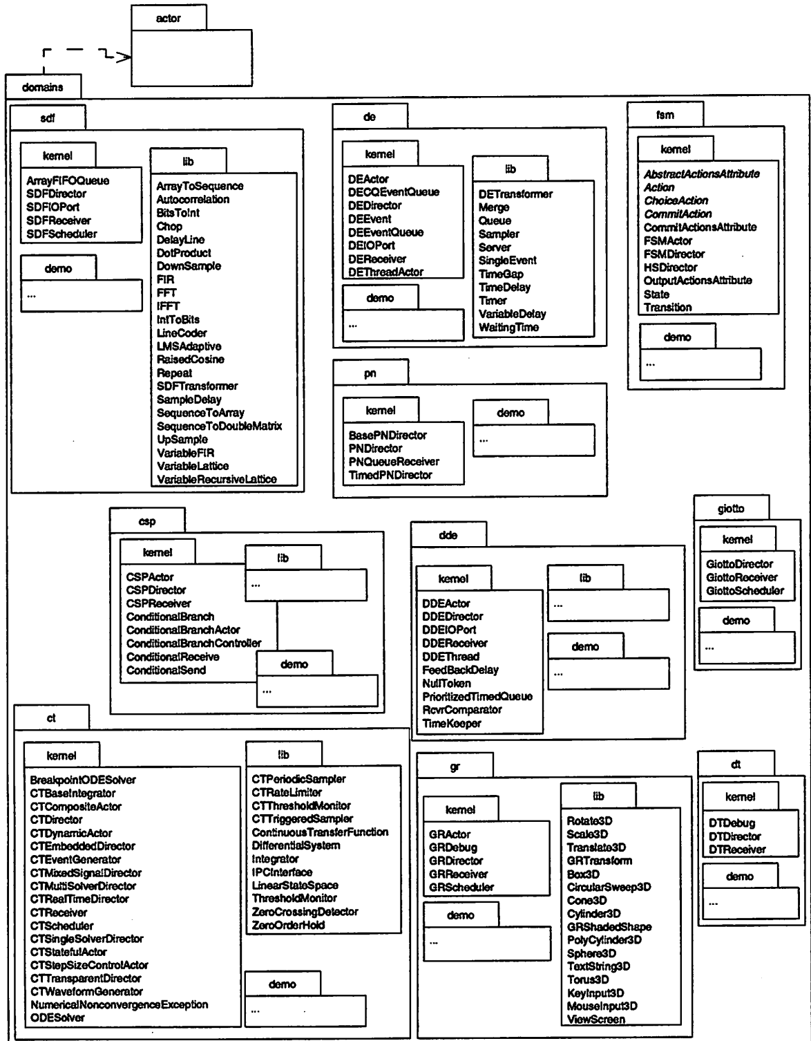
FIGURE 6. Package structure of Ptolemy II domains.
