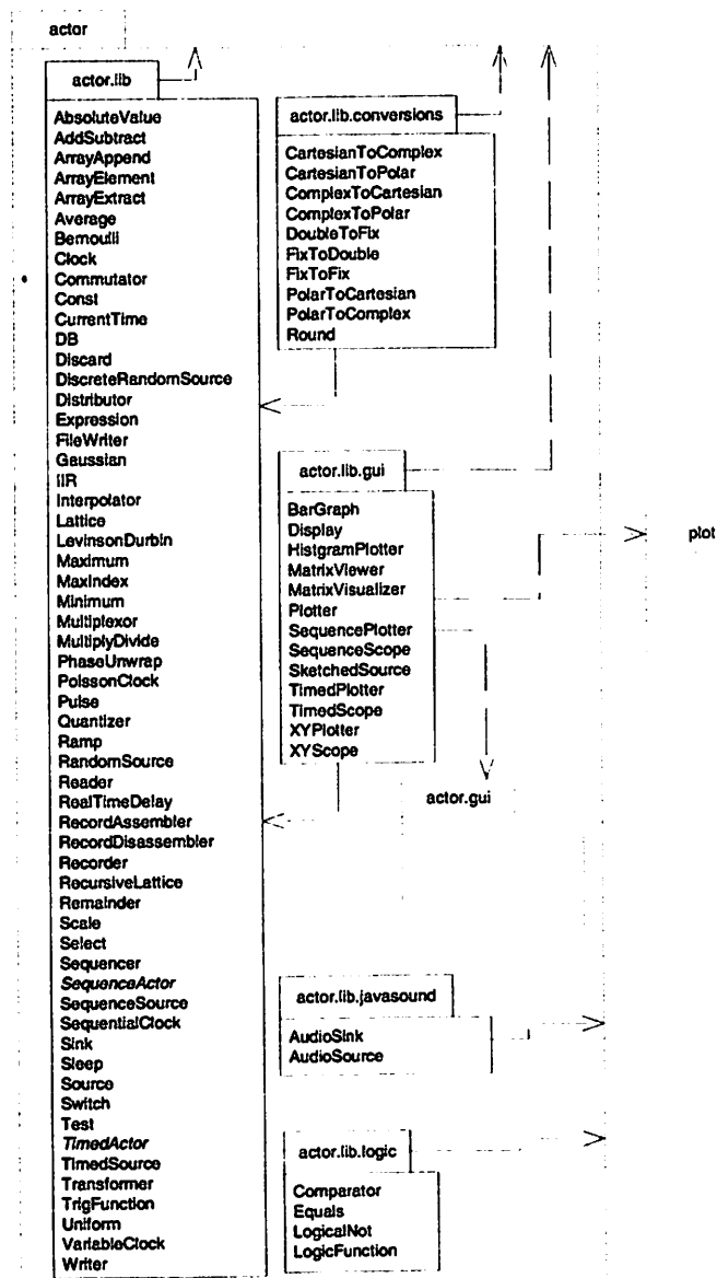
FIGURE 1.7. Packages containing domain-polymorphic actors.
