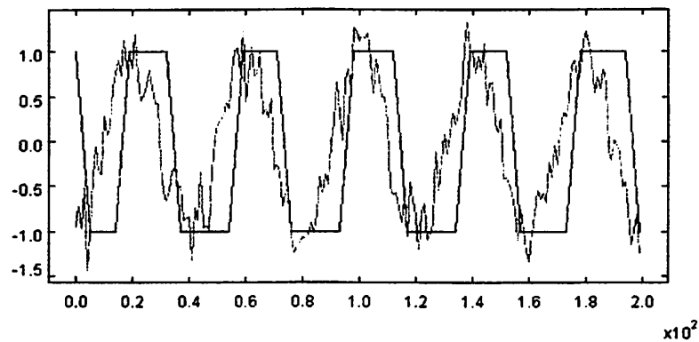
FIGURE 17.10. Sample result of the model shown in figure 17.9.
