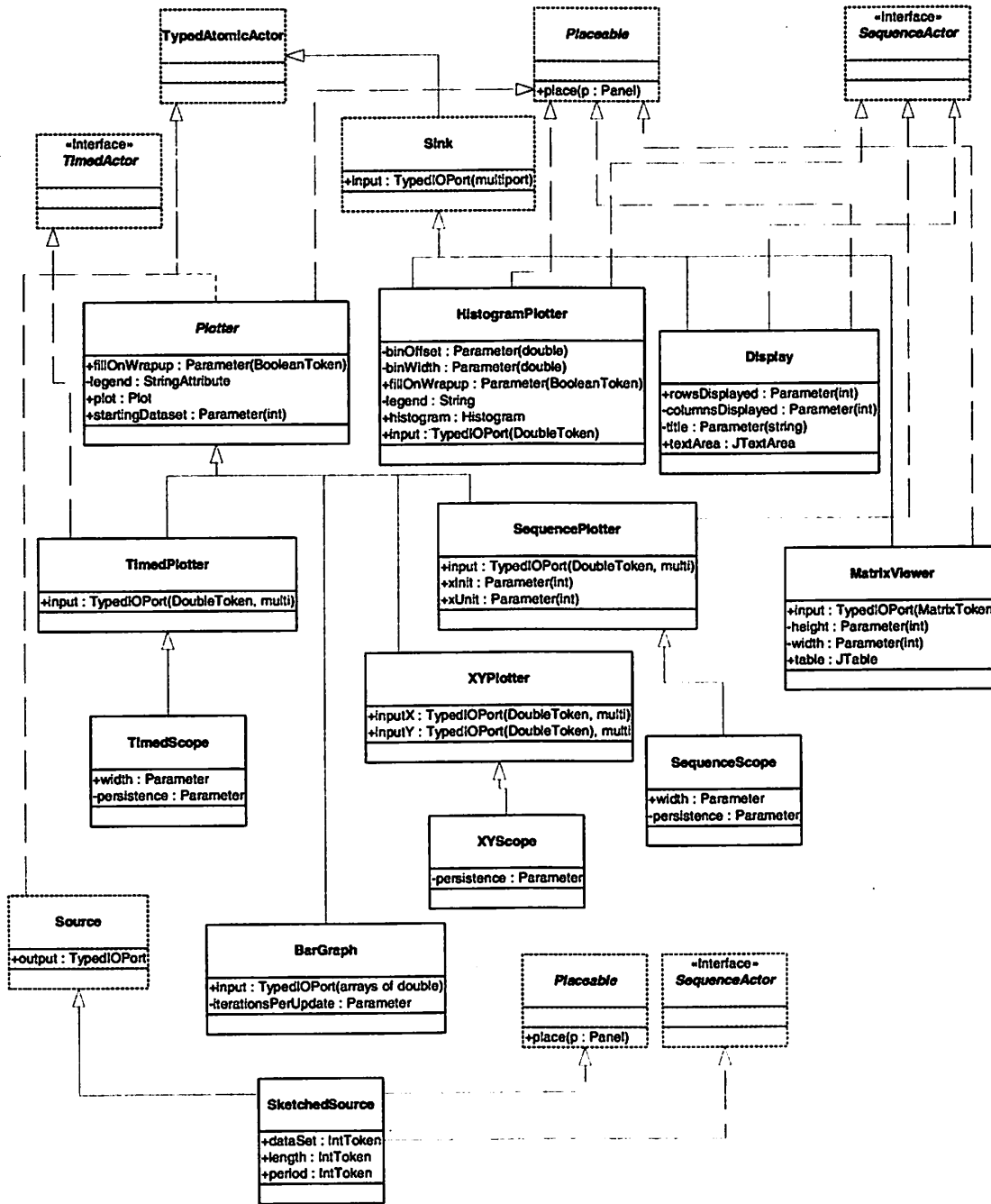
FIGURE 3.3. Organization of actors in the ptolemy.actor.lib.gui package.
