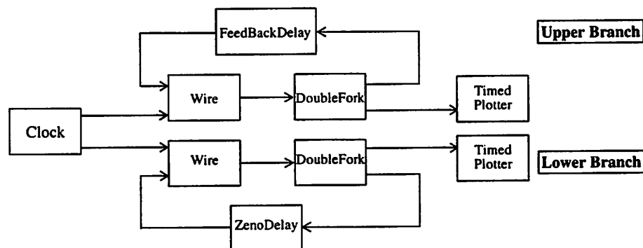
FIGURE 19.7. Localized Zeno condition topology.
