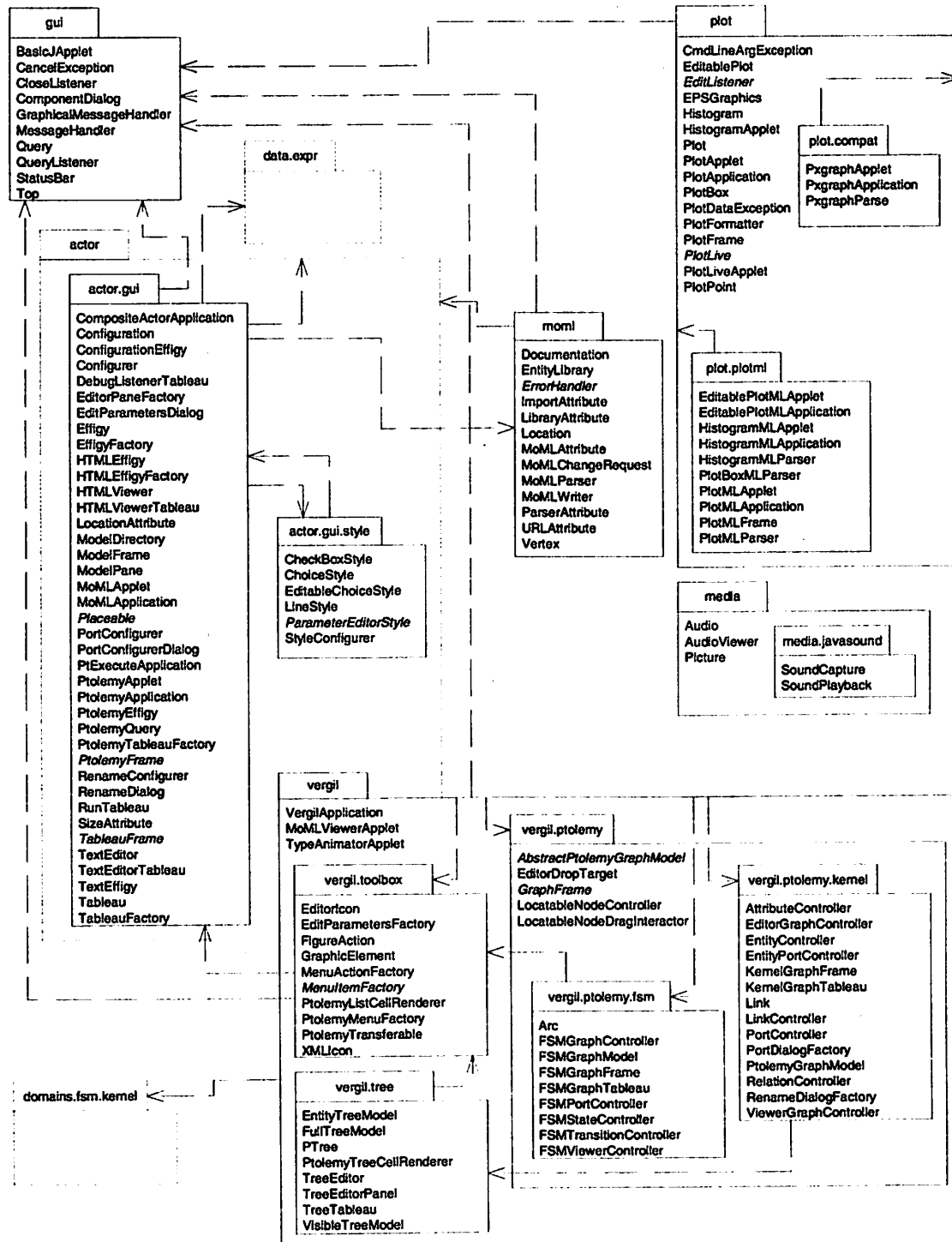
FIGURE 1.8. Packages in Ptolemy II that support user interfaces, including the MoML XML schema and the Vergil visual editor.
