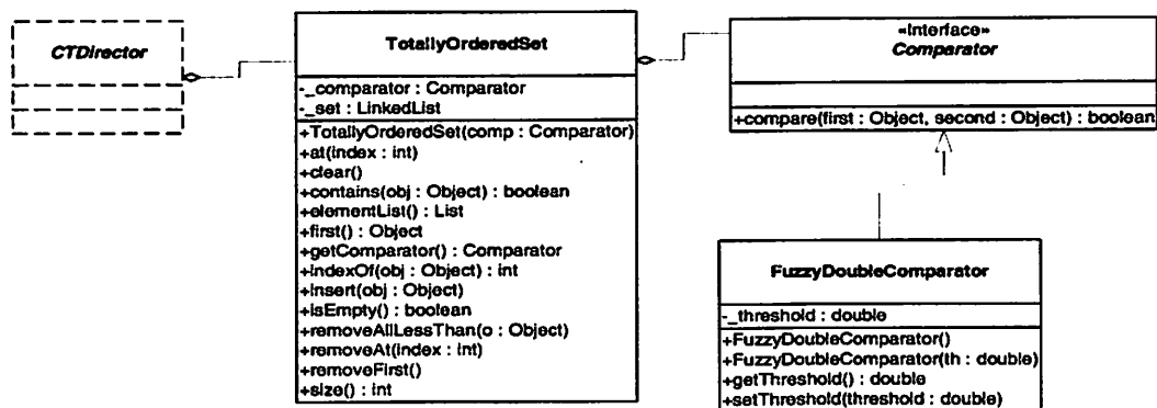
FIGURE 14.16. UML for ct.kernel.util package.
