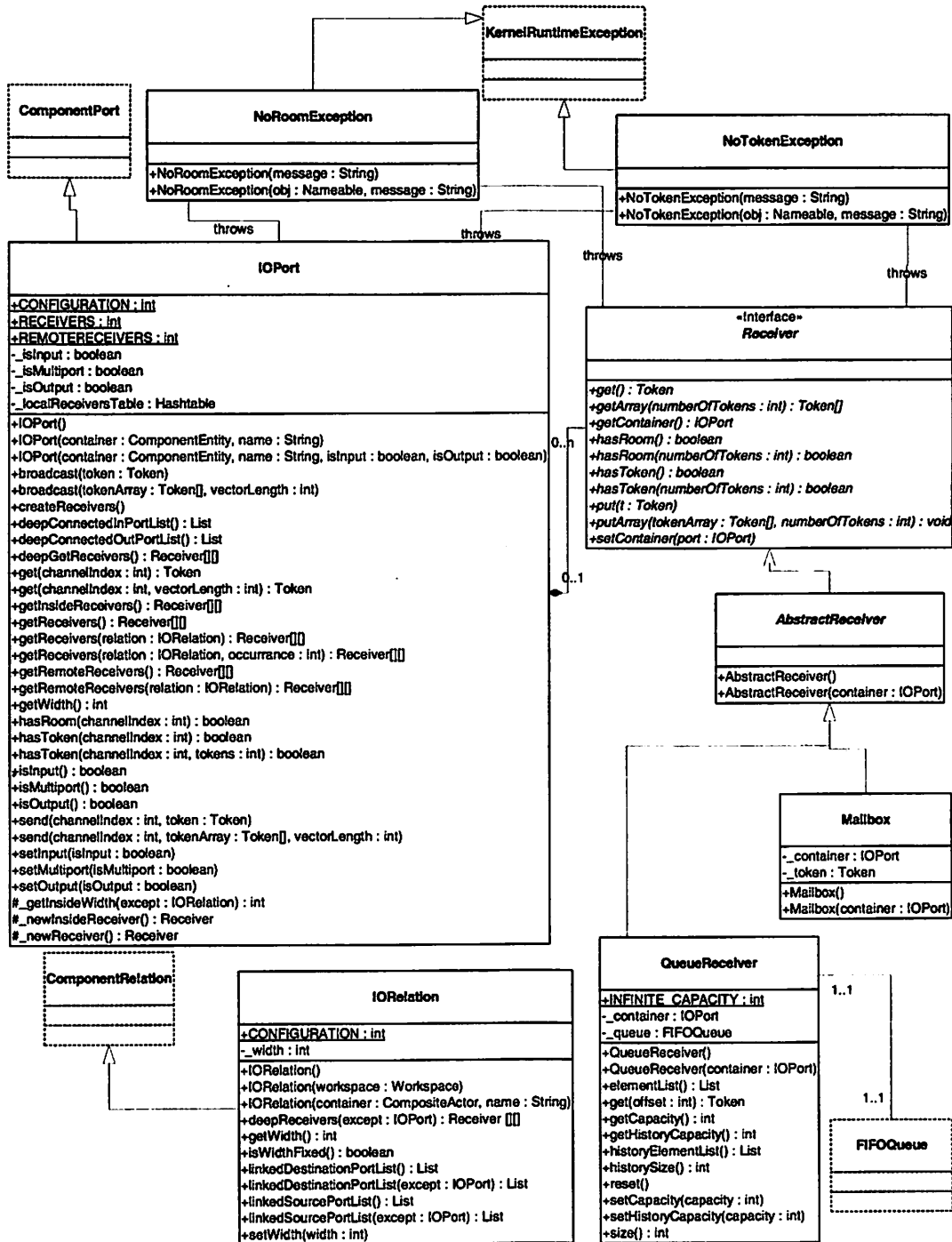
FIGURE 8.2. Port and receiver classes that provide infrastructure for message passing under various communication protocols.
