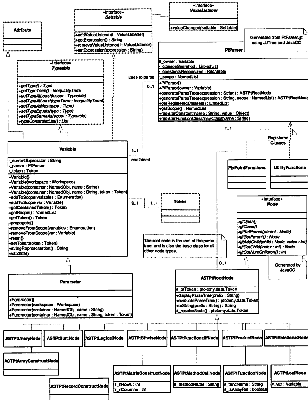
FIGURE 9.3. Static structure diagram for the data.expr package.
