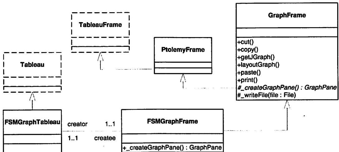
Figure 13.14 Static structure of the Ptolemy FSM graph editor.
