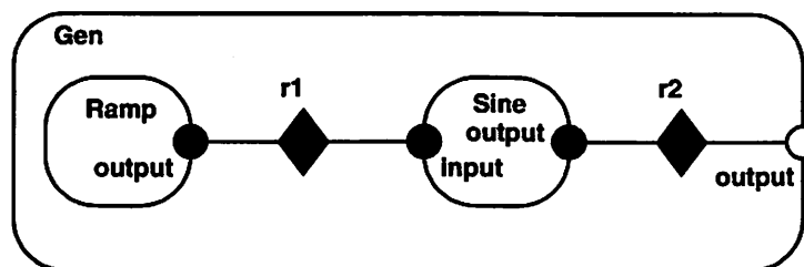
FIGURE 5.7. Sine wave generator topology.
