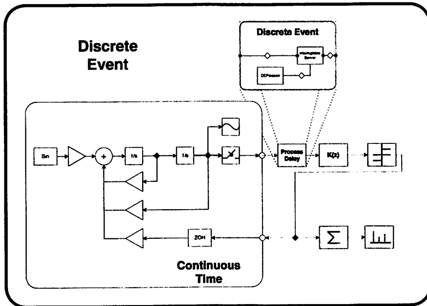
FIGURE 15.12. An example of heterogeneous and hierarchical composition. The CT subsystem and DE subsystem are inside an outermost DE system. This example is developed by Jie Liu [57].
