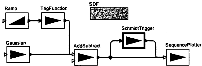
FIGURE 17.9. The top-level model with the SchmittTrigger.
