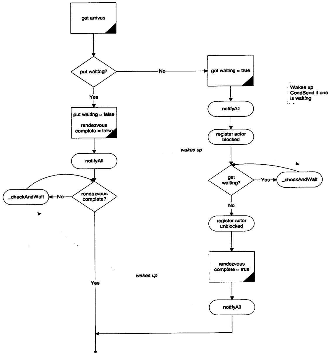
FIGURE 18.10. Rendezvous algorithm.
