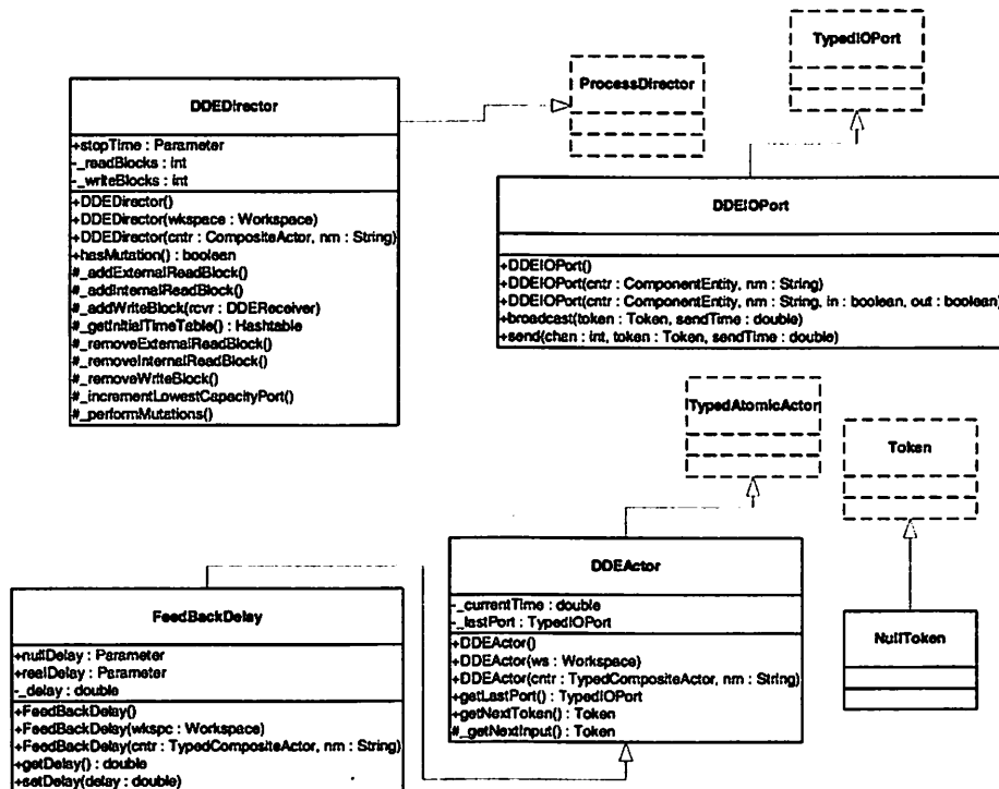
FIGURE 19.6. Additional Classes in the DDE Kernel.
