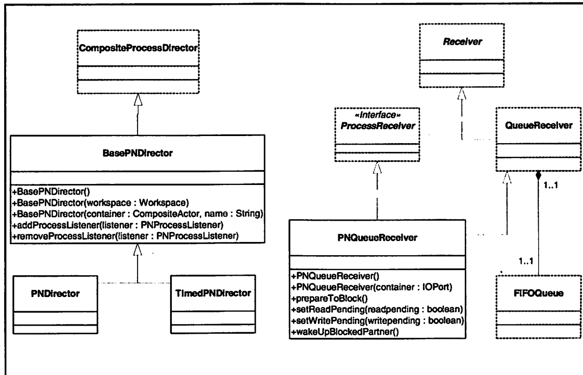
FIGURE 20.1. Static structure of the PN kernel.
