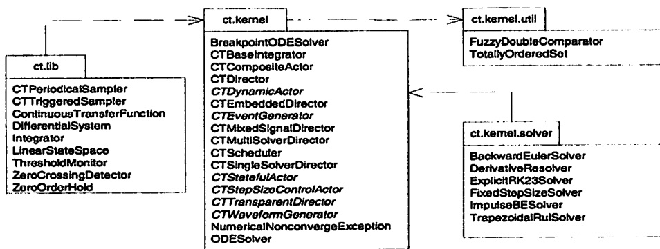
FIGURE 14.15. The packages in the CT domain.
