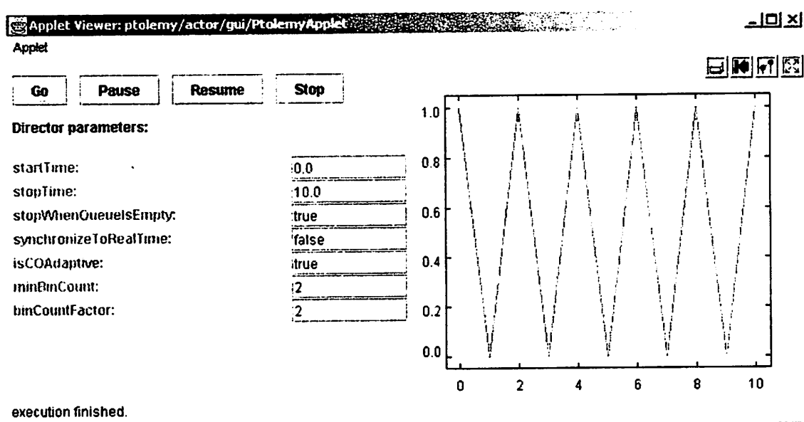
FIGURE 6.5. Result of running the applet of figure 6.3 with horizontal layout, and including the director parameters.
