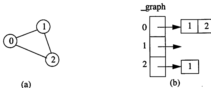
FIGURE 10.2. An undirected graph
