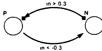
FIGURE 17.6. The mode controller for SchmidtTrigger.
