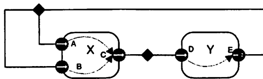
FIGURE 15.2. An example of a directed zero-delay loop.
