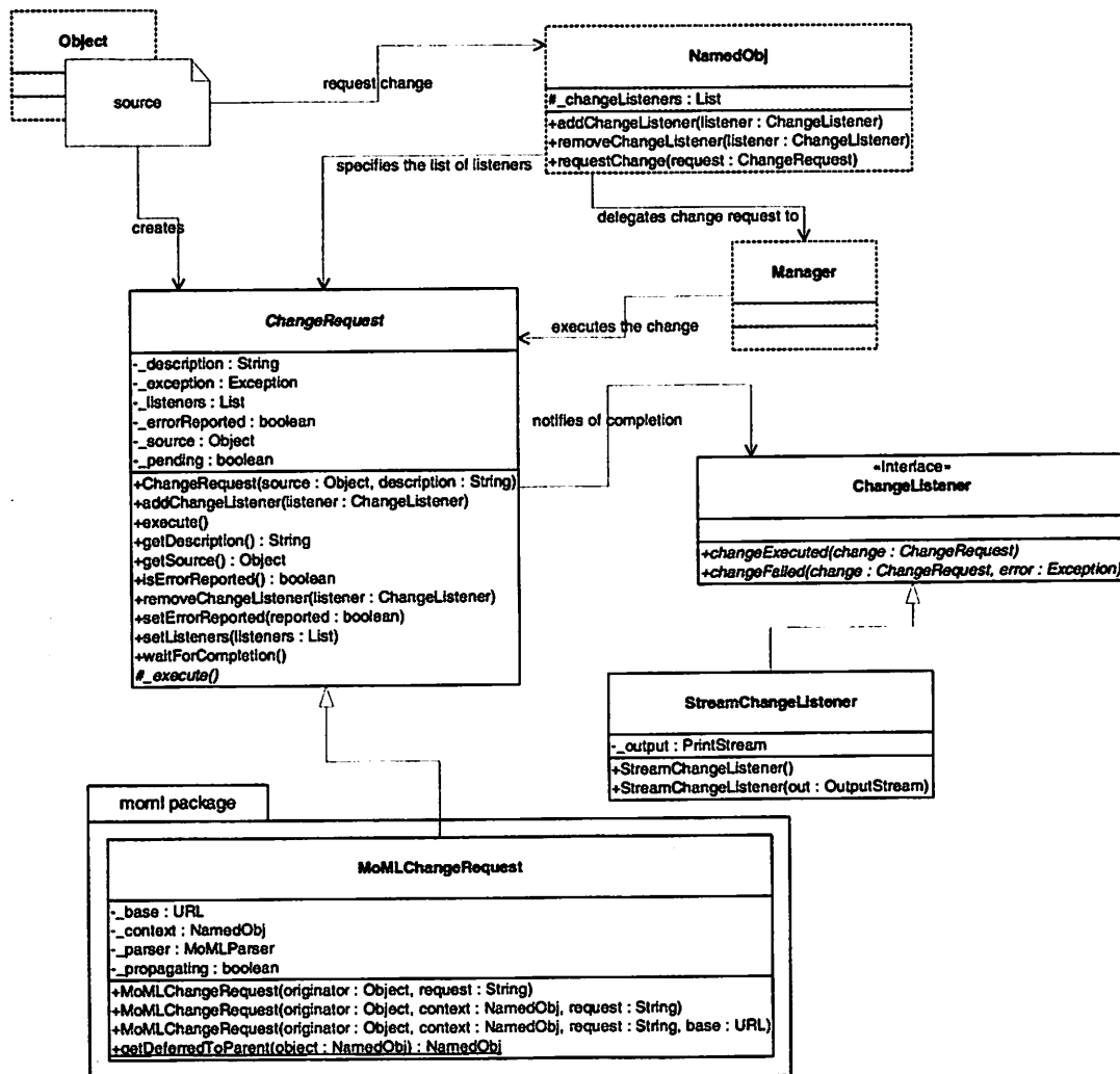
FIGURE 7.13. Classes and interfaces that support controlled topology mutations. A source requests topology changes and a manager performs them at a safe time.
