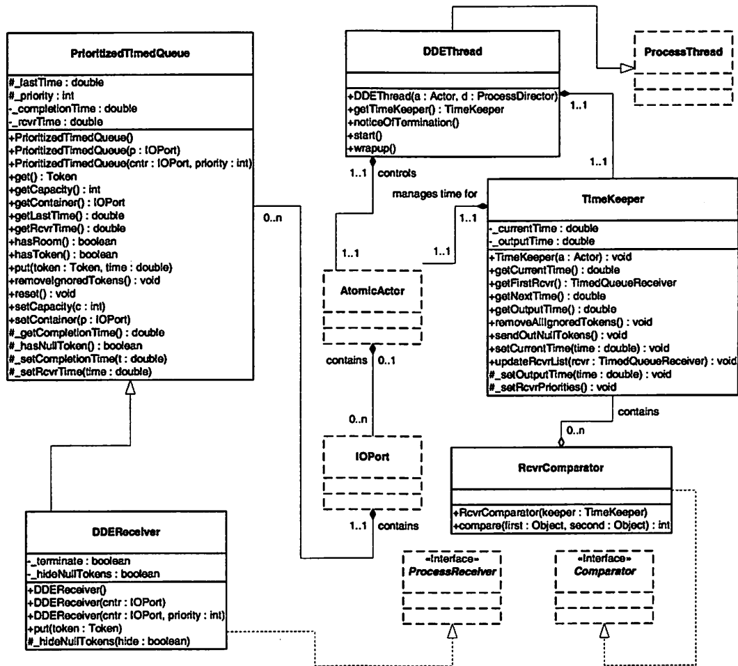
FIGURE 19.5. Key Classes for Locally Managing Time.
