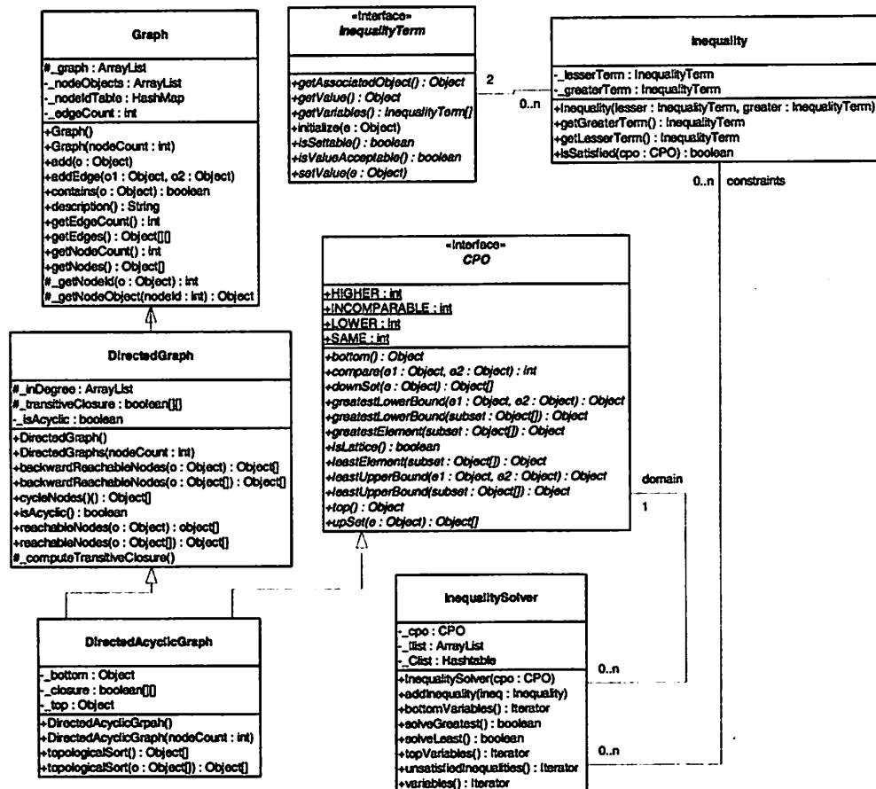
FIGURE 10.1. Classes in the graph package
