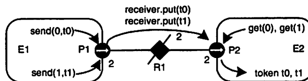
FIGURE 8.4. A bus is an IORelation that represents multiple channels. It is indicated by a relation with a slash through it, and the number adjacent to the bus is the width of the bus.
