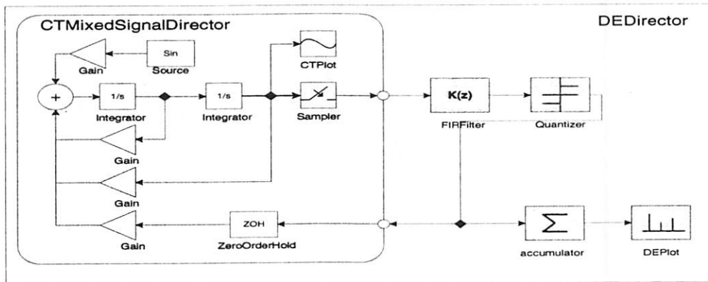
FIGURE 14.10. Block diagram for the micro-accelerator system.
