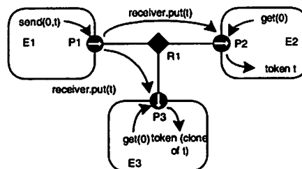
FIGURE 8.5. Channels may reach multiple destinations. This is represented by relations linking multiple input ports to an output port.
