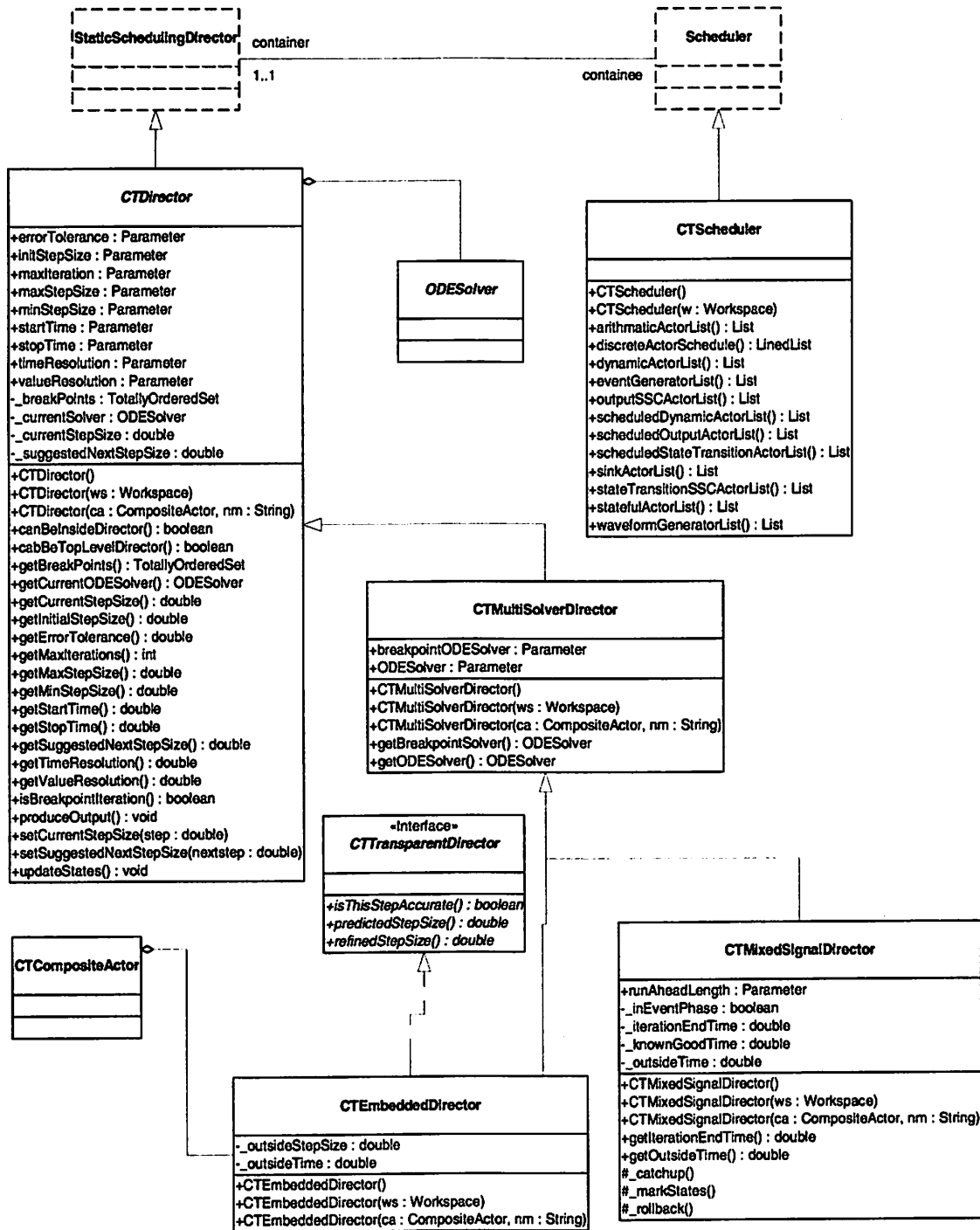
FIGURE 14.18. UML for ct.kernel package, director related classes.
