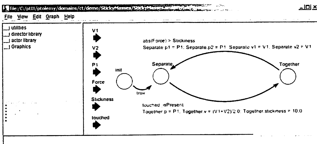
FIGURE 1.3. Visual rendition of a Ptolemy II model as a state transition diagram in Vergil (FSM domain).
