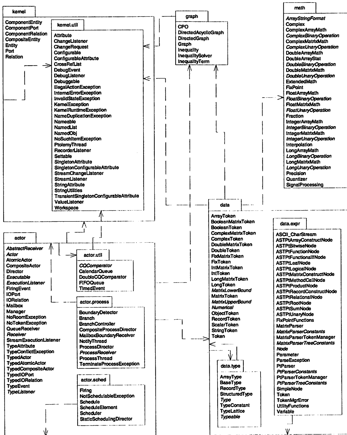
FIGURE 1.4. The core packages shown here support the data model, or abstract syntax, of Ptolemy II designs. They also provide the abstract semantics that allows domains to interoperate with maximum information hiding.
