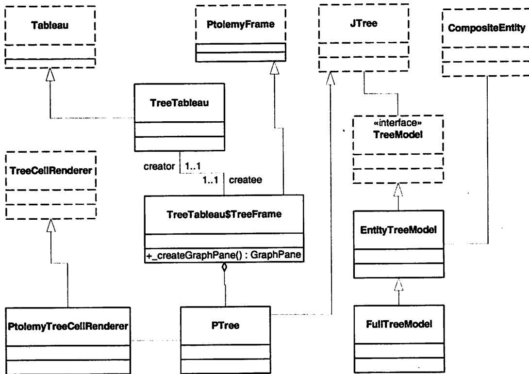
Figure 13.15 Static structure of the ptolemy.vergil.tree package.
