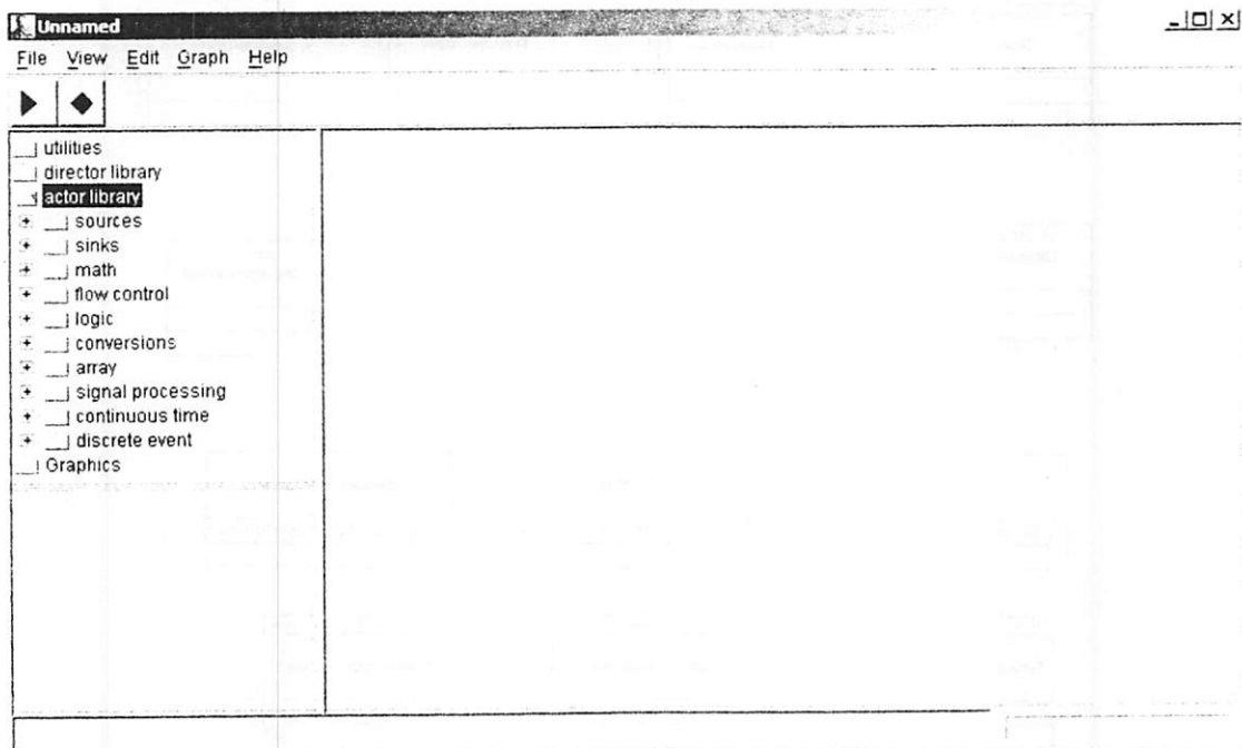
FIGURE 3.2. The default Vergil actor library is shown at the left, expanded to the first level.
