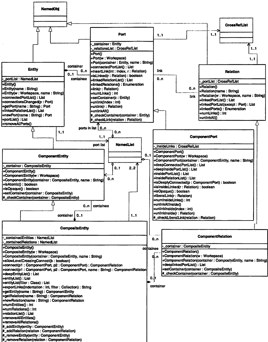
FIGURE 7.4. Key classes supporting clustered graphs.
