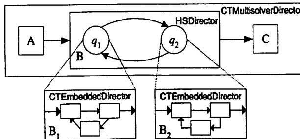
FIGURE 14.6. Hybrid system modeling.
