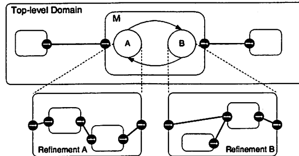
FIGURE 17.5. A modal model example.
