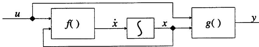
FIGURE 14.2. A conceptual block diagram for continuous time systems.
