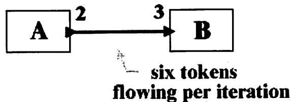
Figure 8. A simple SDF graph with possible schedule (3A)(2B).
