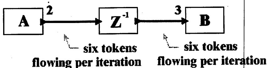
Figure 10. An SDF graph with a delay actor
