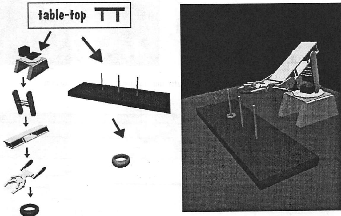
Figure 30. Scene graphs may change over time
