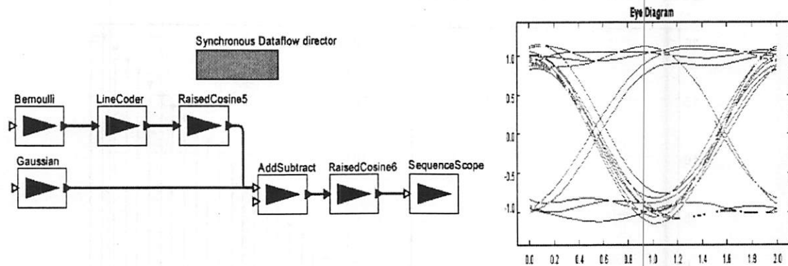
Figure 6. An SDF model (left) for simulating the eye-diagram (right) in communication systems.
