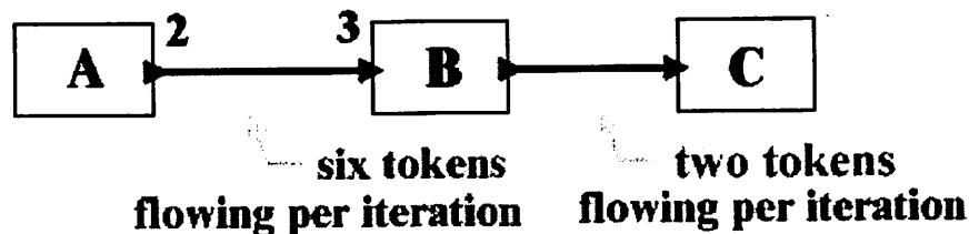
Figure 15. Another DT dataflow graph
