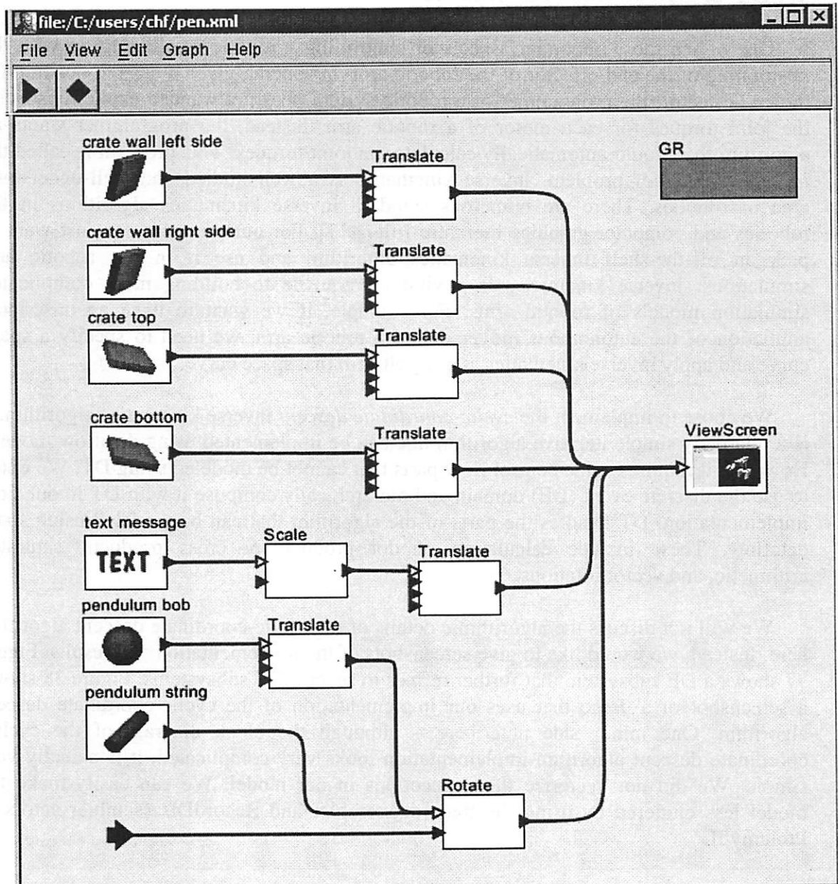
Figure 36. The GR scene graph for pendulum model
