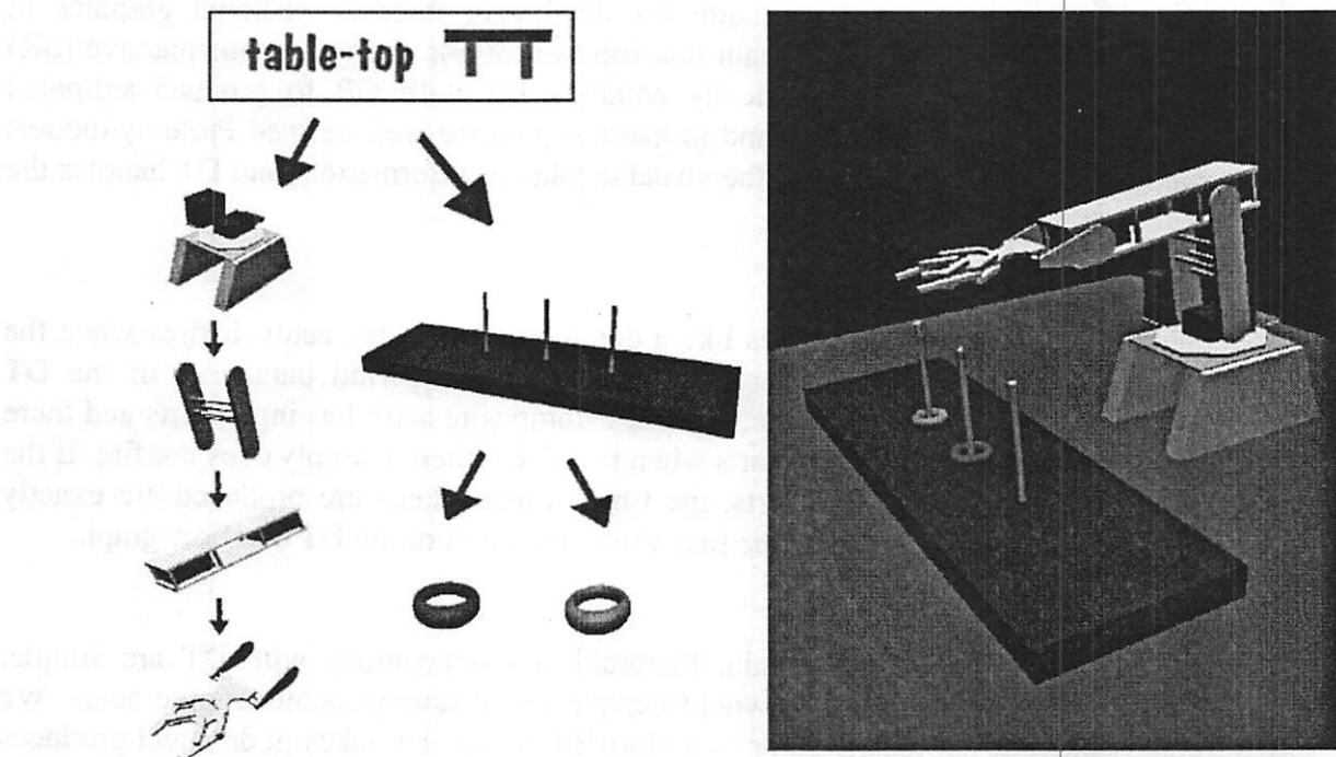
Figure 29. An example scene graph
