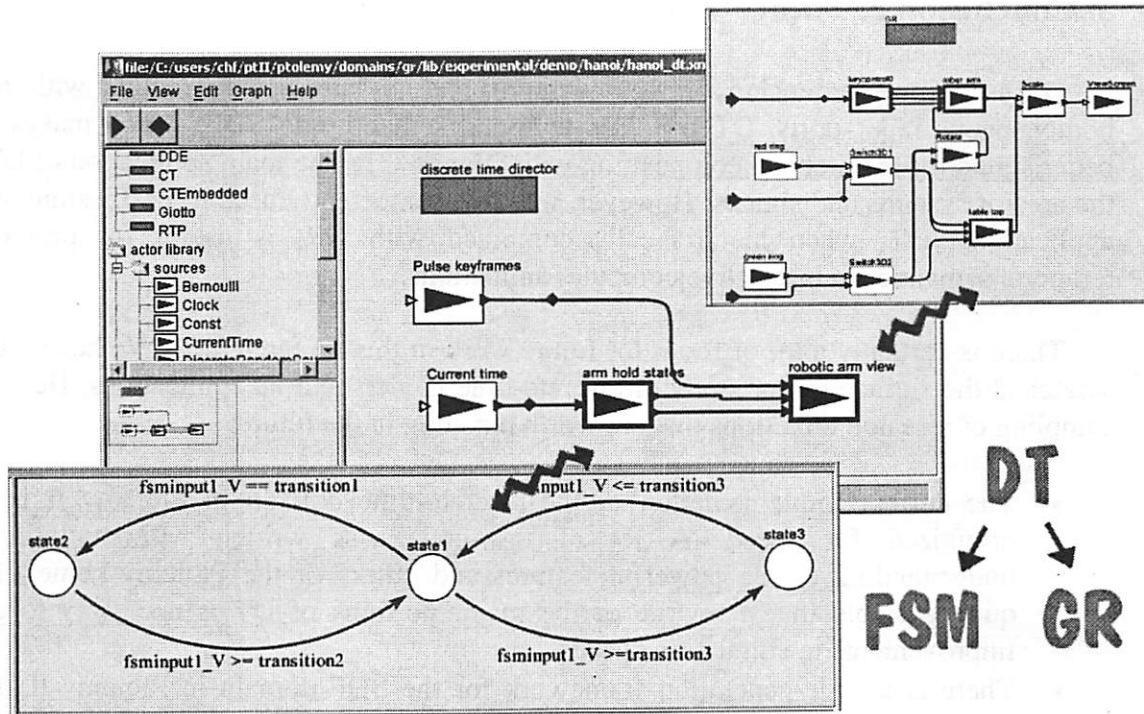
Figure 40. Nested hierarchies: DT refining to FSM and GR
