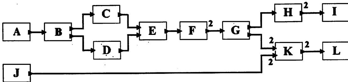
Figure 7. An abstract SDF graph
