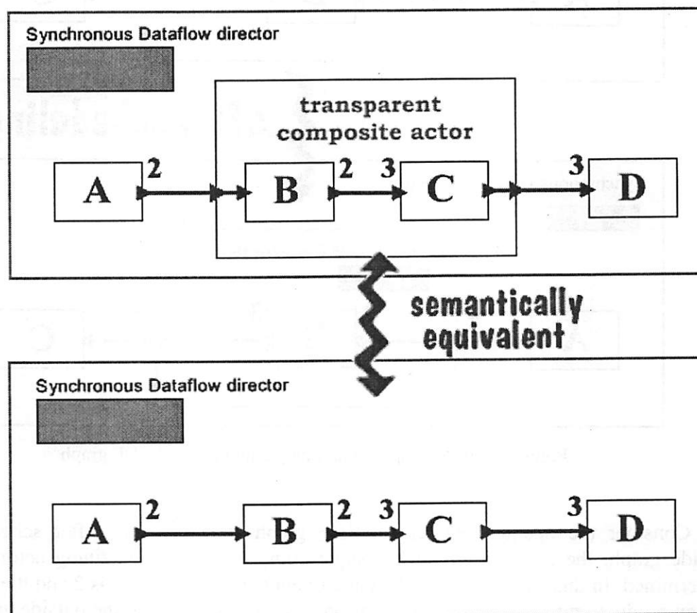
Figure 24. Two semantically equivalent SDF graphs. The top graph shows a hierarchical SDF graph with a transparent composite actor. The bottom graph shows a semantically equivalent non-hierarchical SDF graph.
