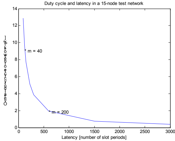
Fig. 8. Overall duty cycle versus latency for varying values of cycle length ( m )
