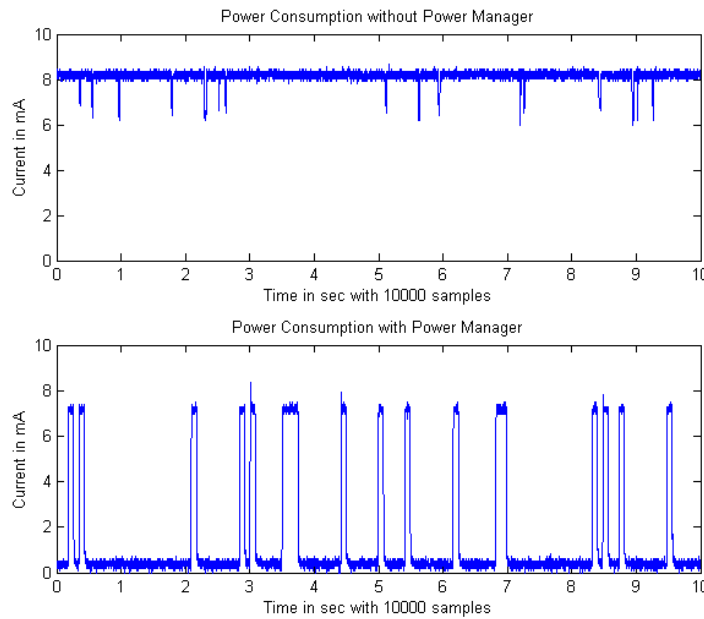
Fig. 5. Measured current at node 1 with and without power management over 10 seconds
