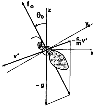
Figure 5.6: Cruising Configuration
