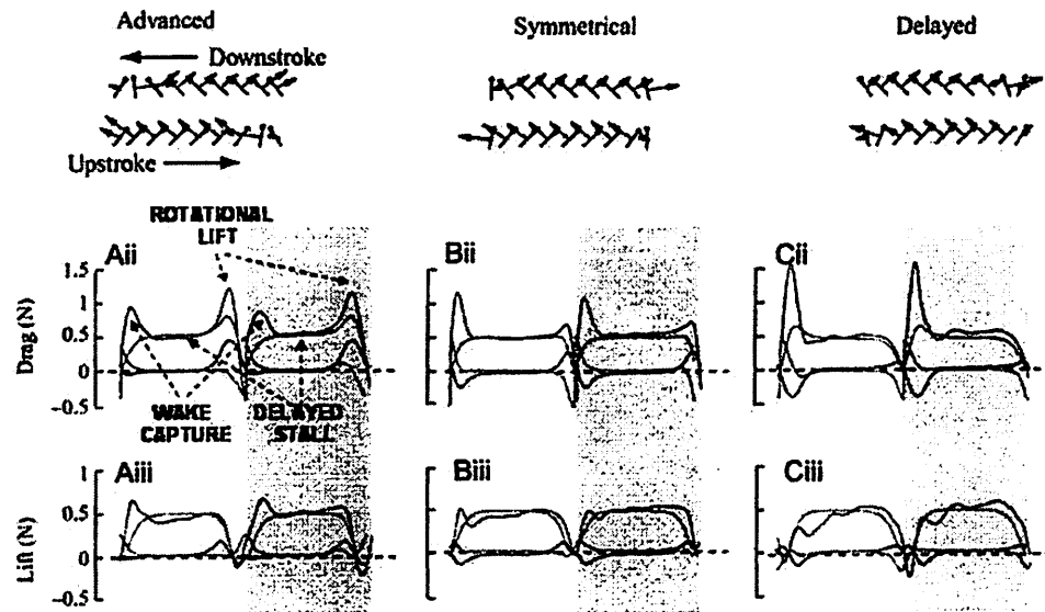
Figure 2.4: (Top) Wing kinematics diagram for three different wing trajectories in which the rotation of the wing is advanced, symmetric or delayed relative to the inversion of wing motion. (Center and Bottom) Aerodynamic drag and lift forces as measured by Robofly, a dynamically scaled model of an insect wing, during the course of a full wingbeat. The gray area corresponds to the upstroke portion of the wingbeat. Arrows indicate how specific aerodynamic mechanisms act during flapping flight. Courtesy of [24].
