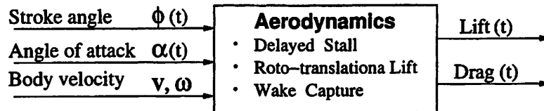
Figure 3.4: Block diagram of the Aerodynamical Module
