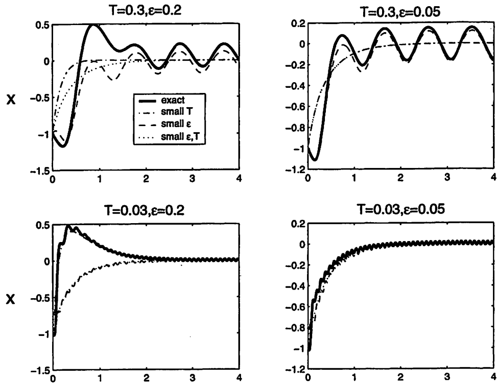
Figure 4.9: Solutions of state x for closed loop feedback of Example 4.4.1 for different value of parameter \epsilon and T . The different traces correspond to System (4.42) (exact), System (4.43) (small \epsilon ), System (4.44) (small T ), and System (4.45) (small \epsilon, T ).
