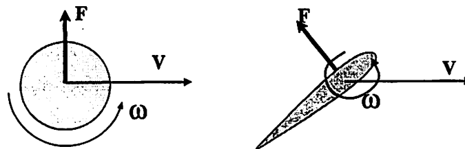
Figure 2.2: Rotational lift for a rotating ball and for a rotating wing
