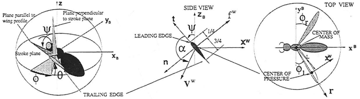
Figure 5.1: Definition of wing kinematic parameters: (left) 3D view of left wing, (center) side view of wing perpendicular to wing axis of rotation \vec{r} , (right) top view of insect stroke plane
