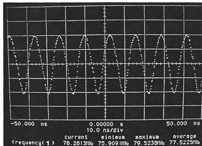
Fig. 21 – Snapshot of the oscilloscope screen showing 1\mu\text{m} gate ring oscillator frequency
