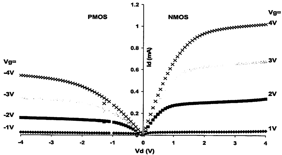
Fig. 17 - Drain current vs. drain voltage characteristics of PMOS and NMOS devices
