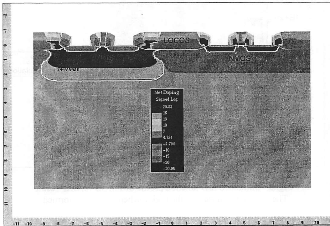
Fig. 5 - Final CMOS structure after process simulation in TSUPREM4
