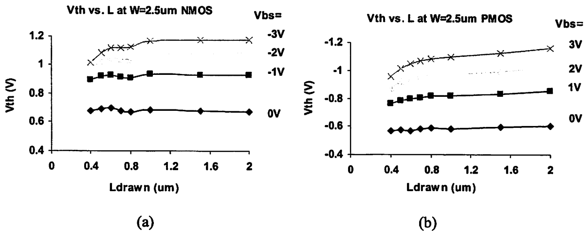
Fig. 18 - Threshold voltage roll-off vs. drawn channel length at W=2.5\mu\text{m}
