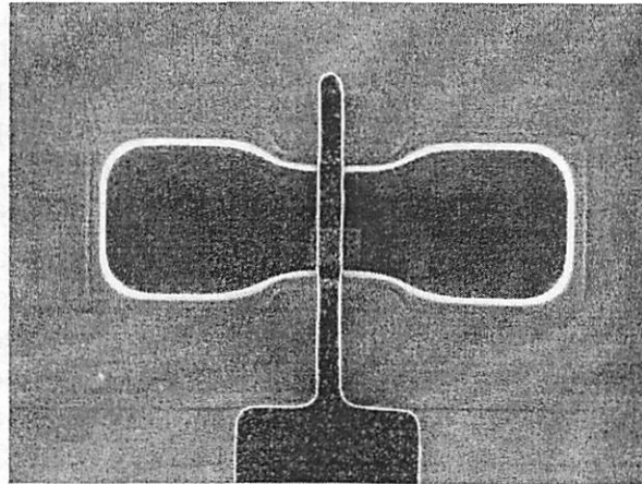
Fig. 3 - Top view SEM image of a 0.4\mu\text{m} transistor after poly gate patterning
