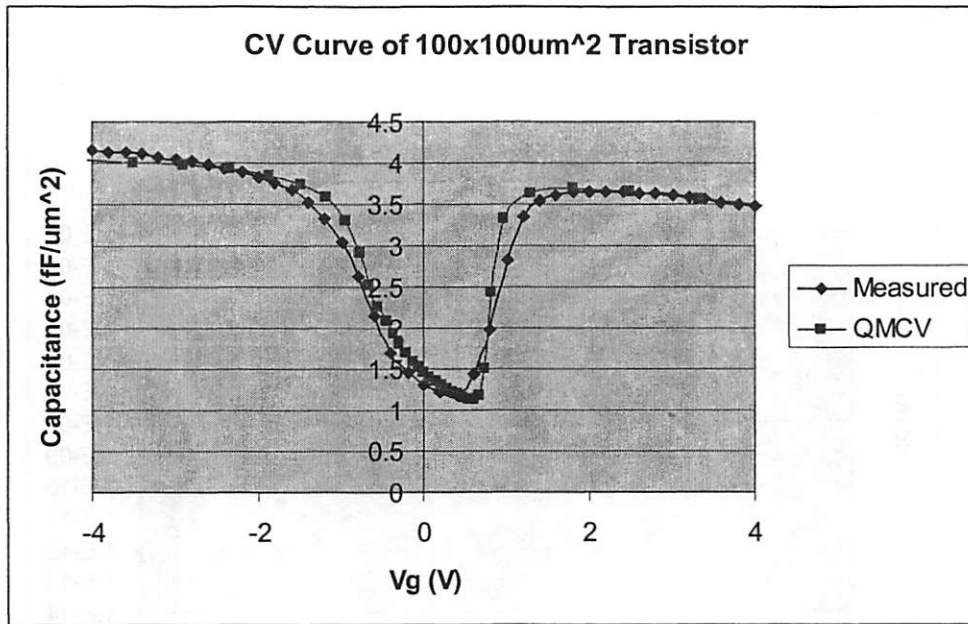
Fig. 10 - Measured and simulated CV curves of NMOS transistor (W/L=100/100) (Fitting parameters: t_{ox} = 8\text{nm} , N_{poly} = 2\text{E}19 , N_{sub} = 2.1\text{E}17 , V_{fb} = -0.75 )
