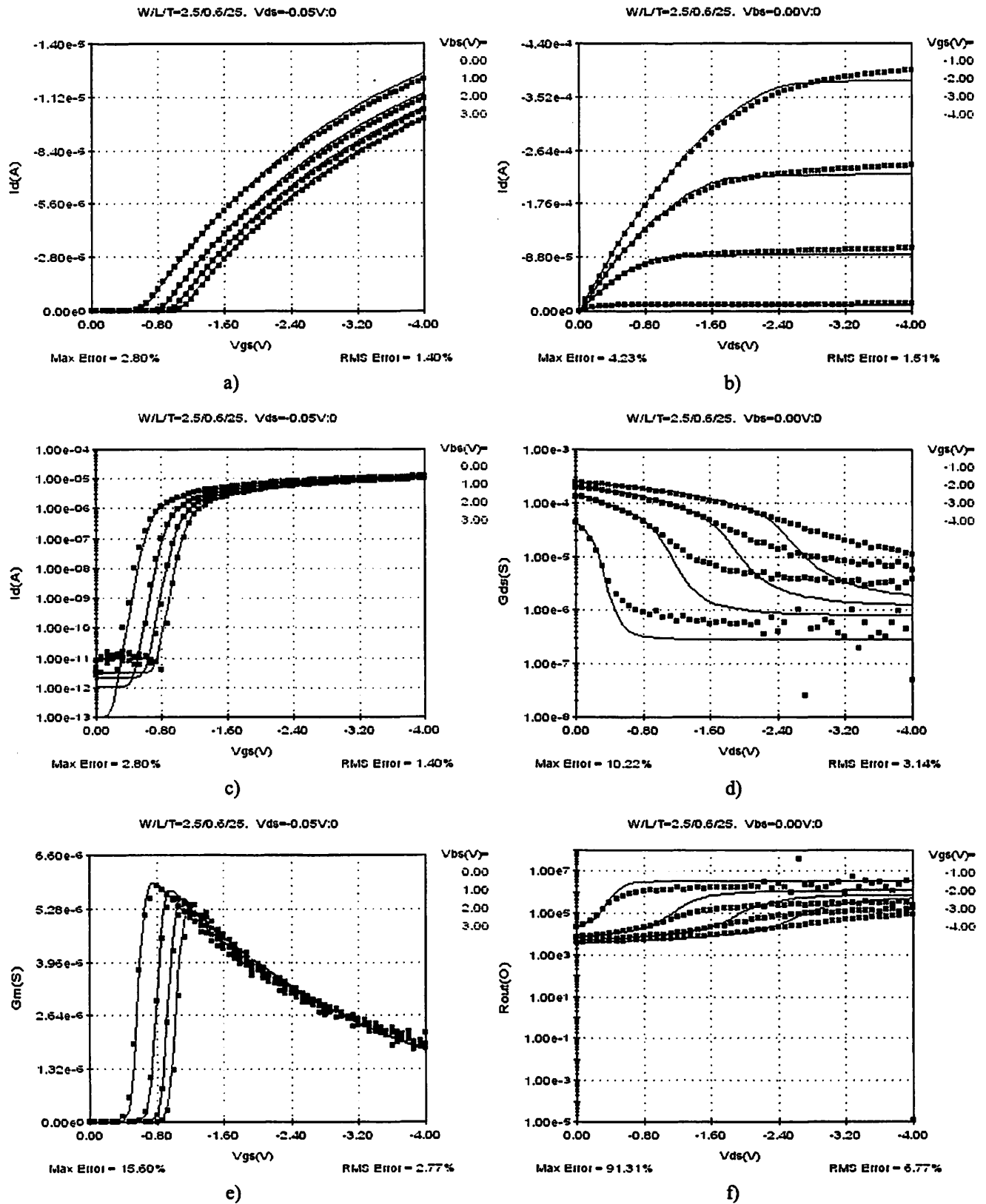
Fig 35 - L=0.6um W=2.5um PMOS
