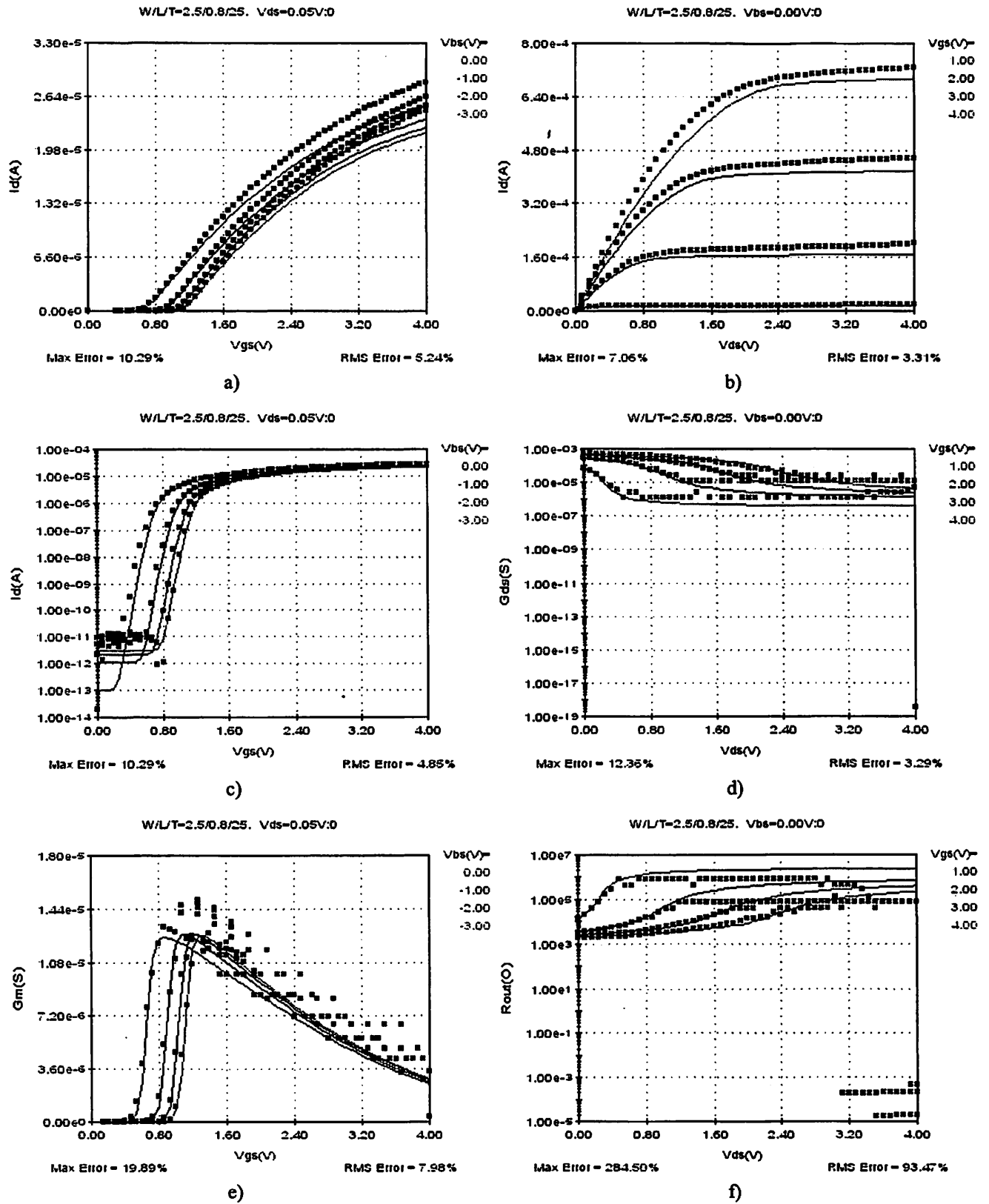
Fig 30 - L=0.8um W=2.5um NMOS
