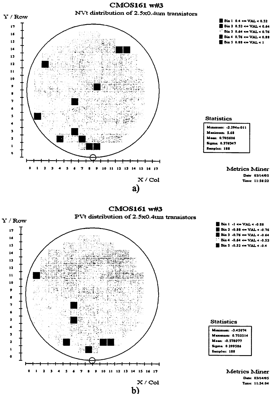
Fig. 22 - Wafer map of NVt (a) and PVt (b) distribution on wafer#3 CMOS161
