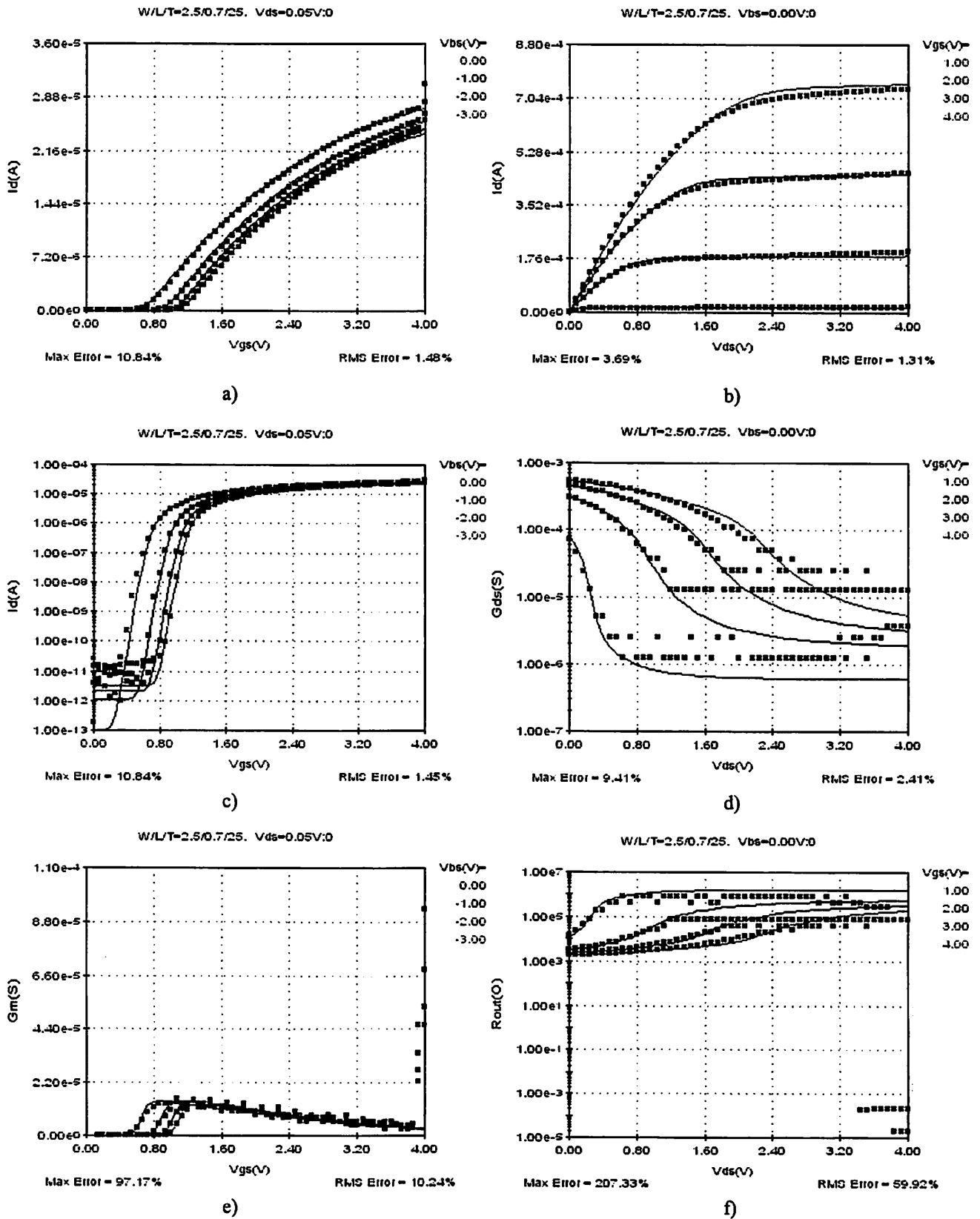
Fig 29 - L=0.7\mu\text{m} W=2.5\mu\text{m} NMOS
