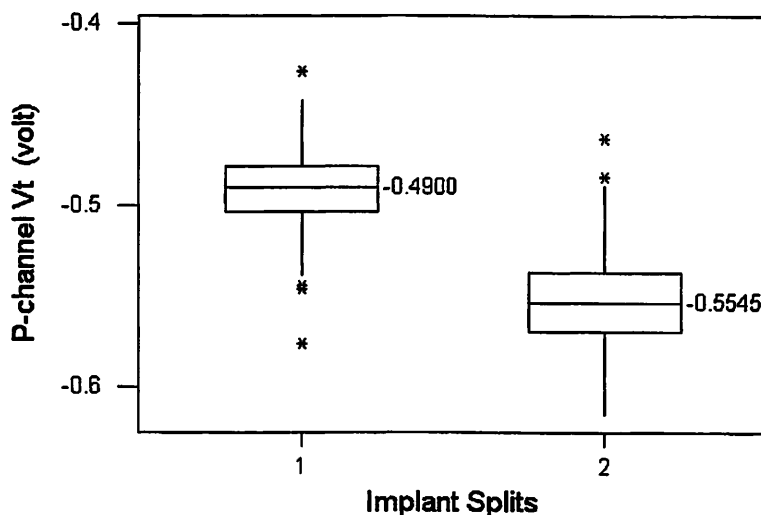
Fig. 20 - Threshold voltages in PMOS split groups: PMOS split group #1: Wafers #6, 7, 8, 9, 10 (N-Well imp. dose 2E13 and PVt imp. dose 1E12) PMOS split group #2: Wafers #1, 2, 3, 4, 5 (N-Well imp. dose 1E13 and PVt imp. dose 2E12)
