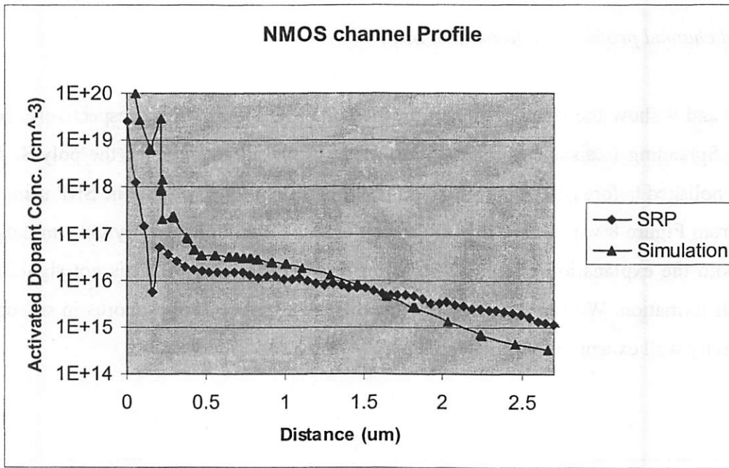
Fig. 9 - Simulated NMOS channel doping profile vs. SRP result Plot starts with poly-Si gate at 0 \mu m distance.
