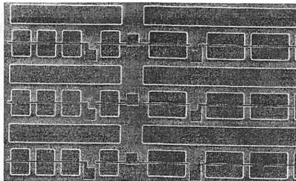
Fig. 4 - Top view SEM image of a 1\mu\text{m} gate ring oscillator section
