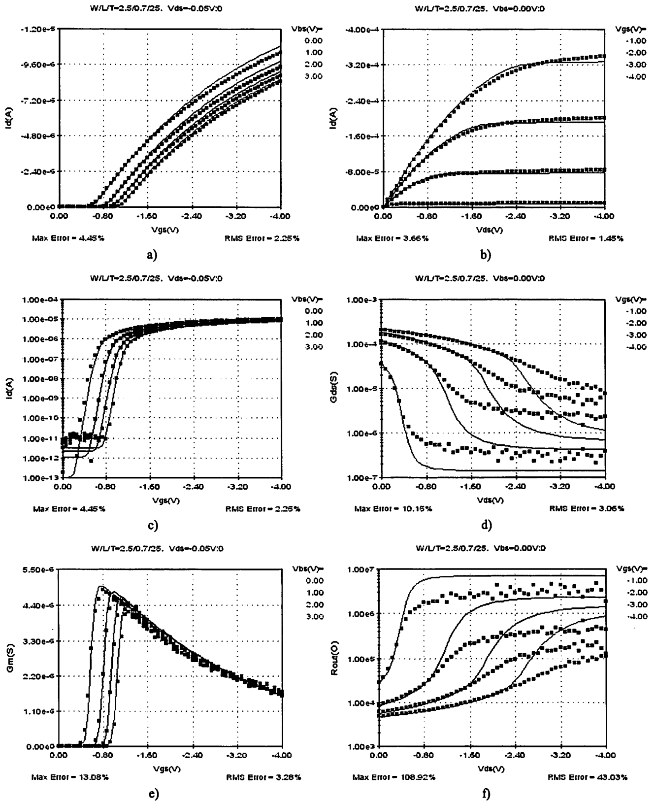
Fig 36 - L=0.7um W=2.5um PMOS
