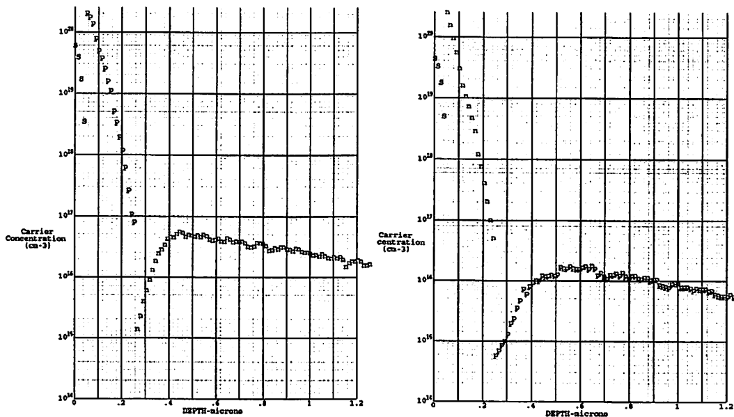
Fig.14 - P+ source-drain (left) and N+ source-drain doping profile
