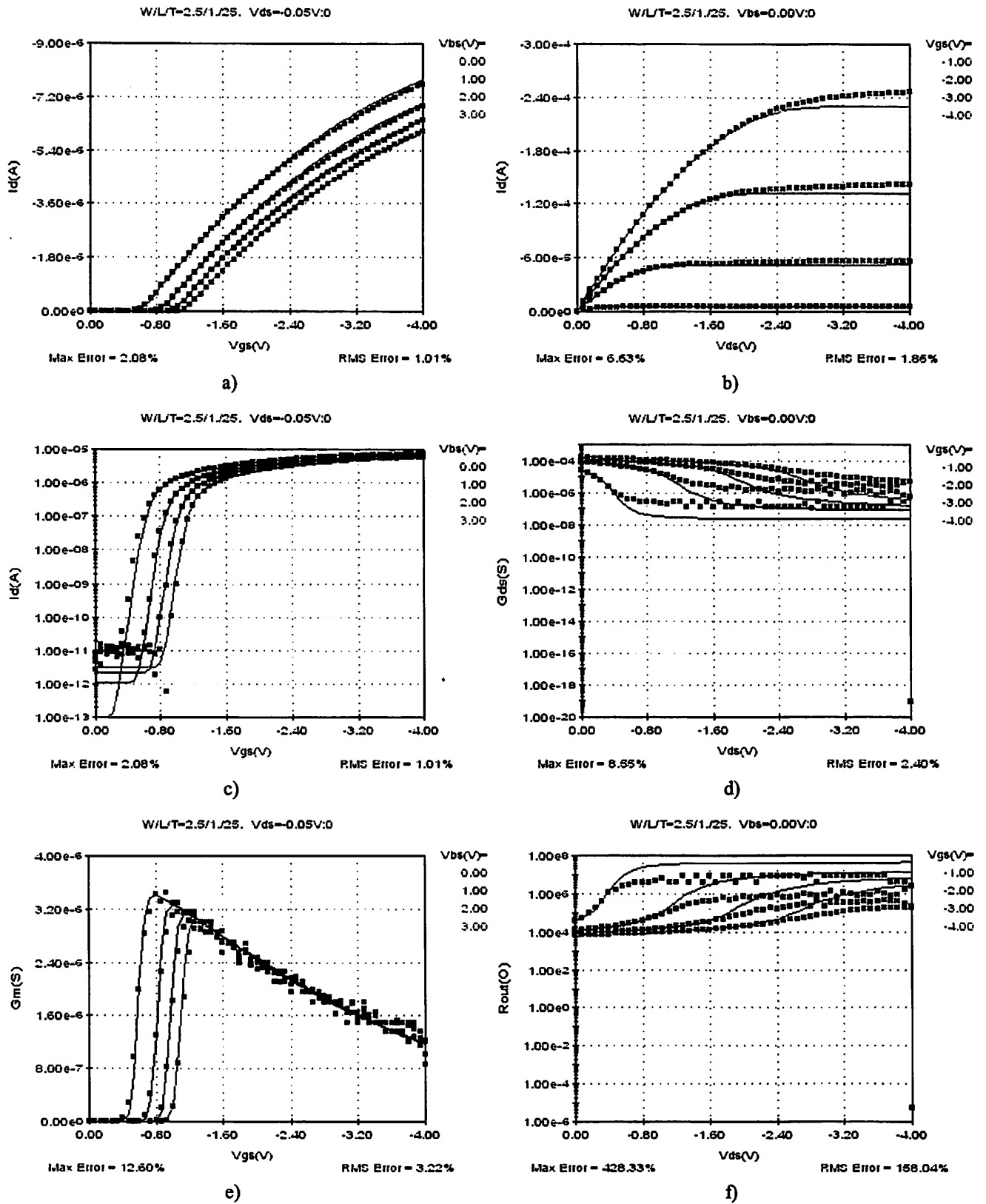
Fig 38 - L=1\mu\text{m} W=2.5\mu\text{m} PMOS
