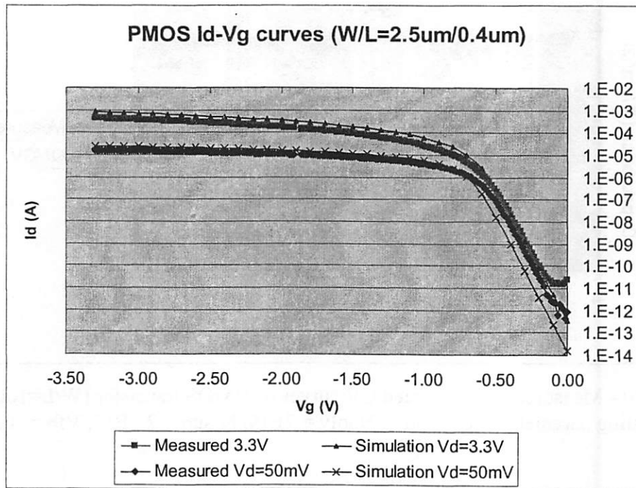
Fig. 11 - Measured and simulated I_d - V_g curves of PMOS transistor ( W/L=2.5/0.4 )
