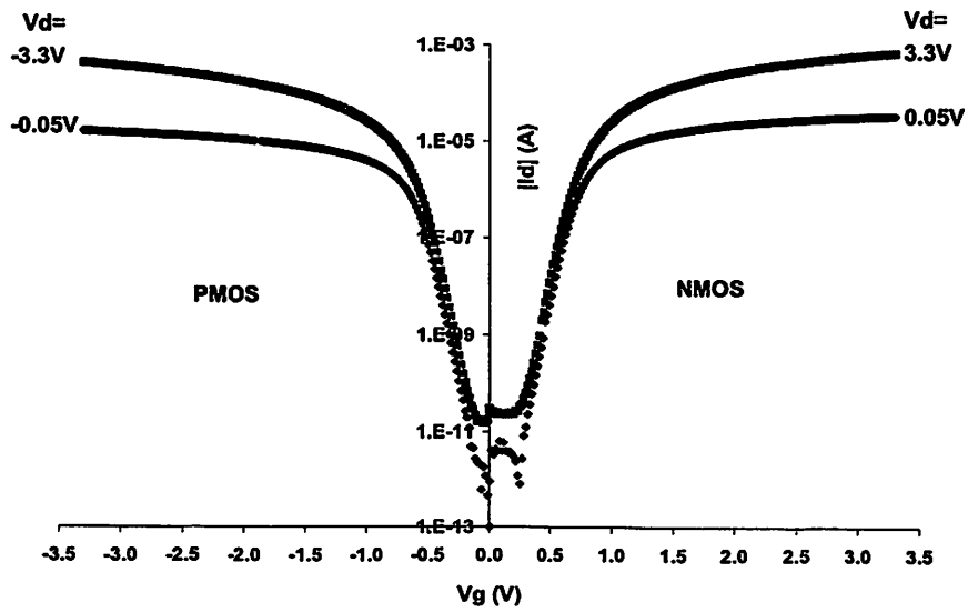
Fig. 16 - PMOS and NMOS sub-threshold characteristics
