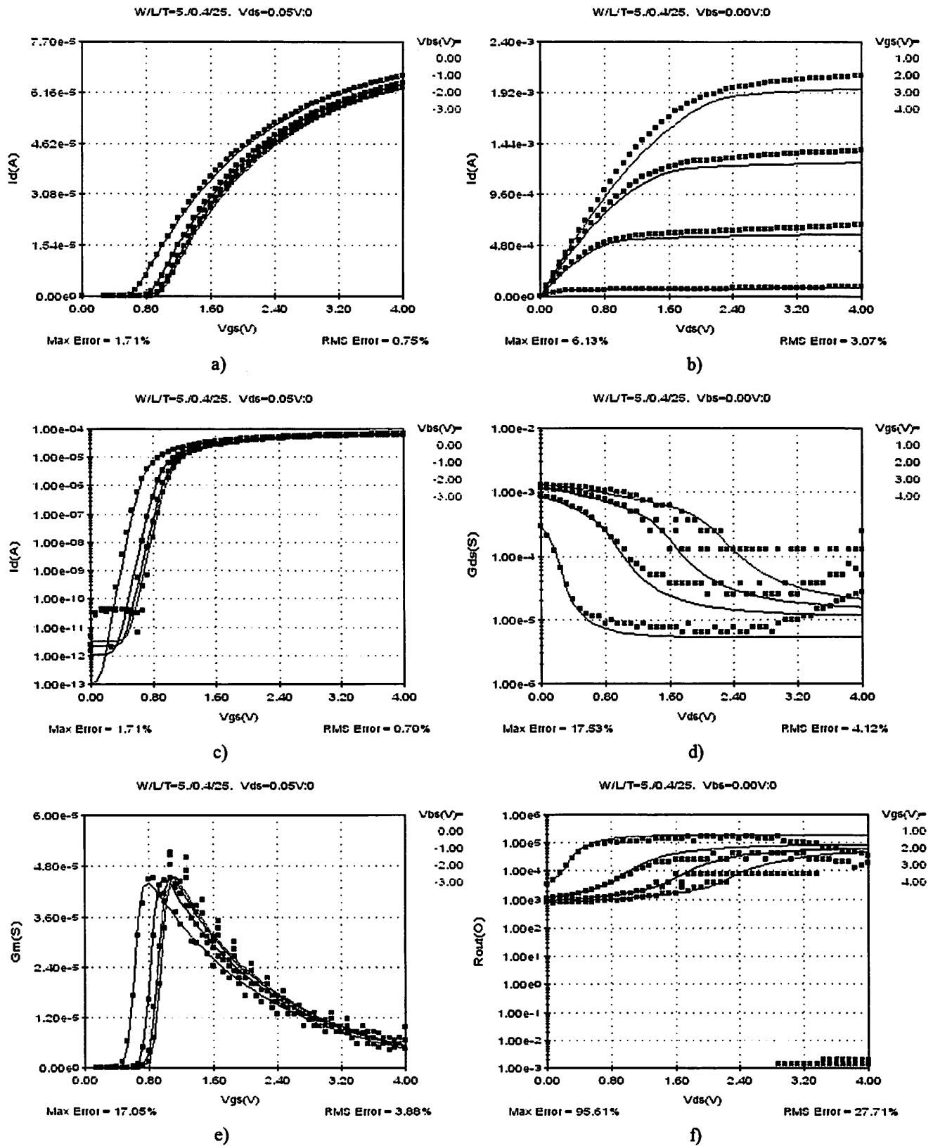
Fig 26 - L=0.4um W=5um NMOS
