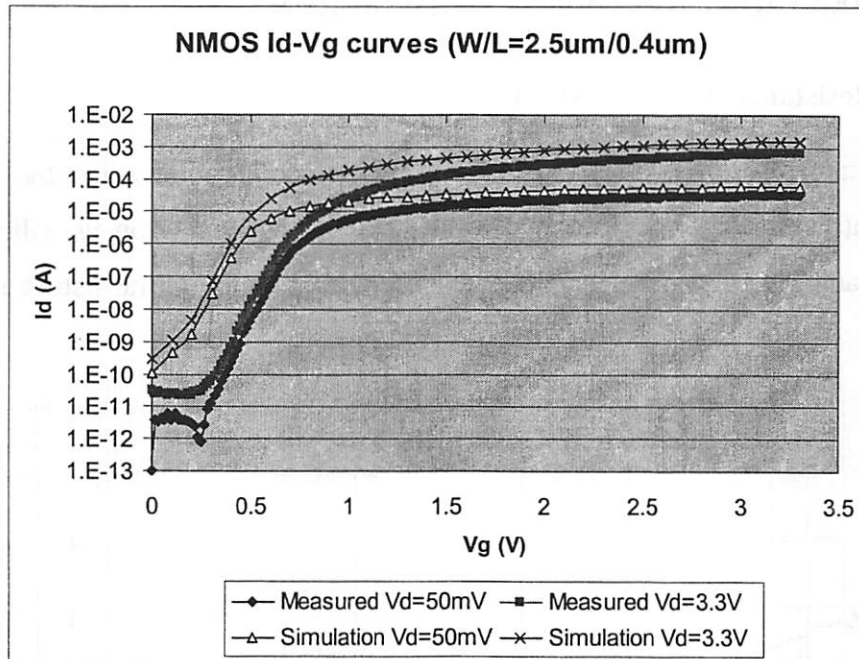
Fig. 12 – Measured and simulated Id-Vg curves of NMOS transistor (W/L=2.5/0.4)
