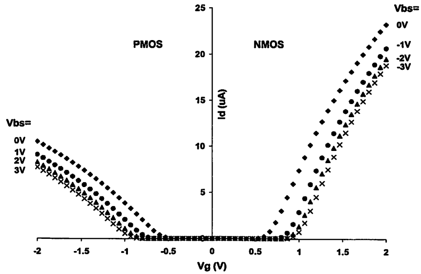
Fig. 15 - Drain current vs. gate voltage at varying substrate bias on PMOS and NMOS transistors in the linear region ( V_d=50\text{mV} )
