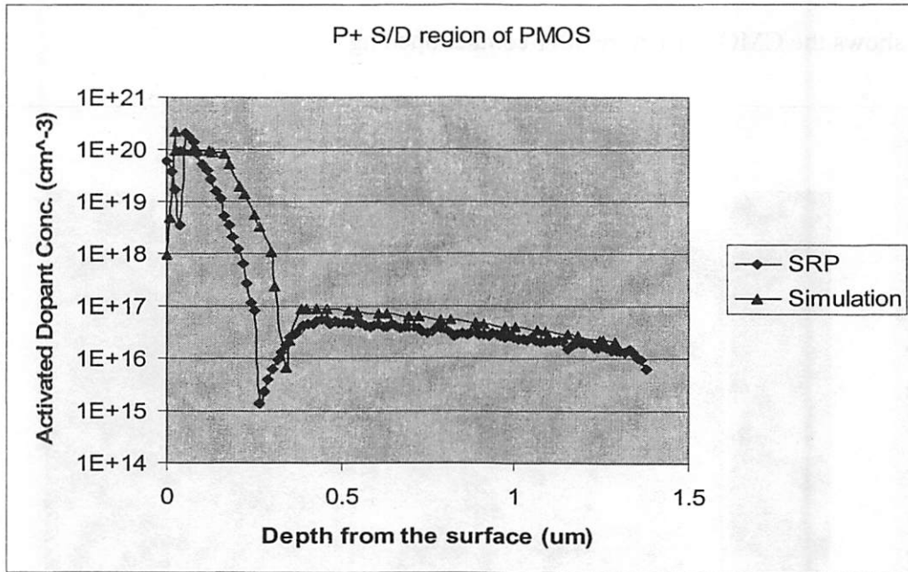
Fig. 6 - Simulated S/D junction profile of PMOS vs. SRP result The drop at the surface is the region where silicide is formed.
