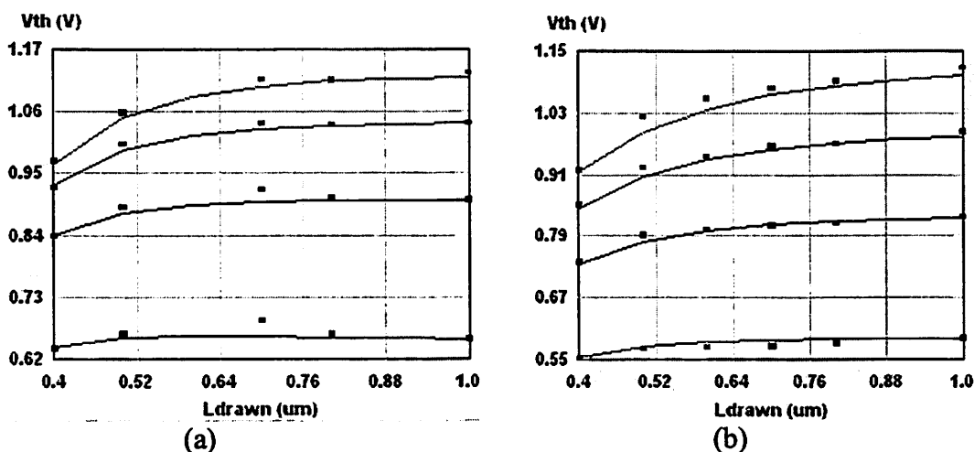
Fig. 23 - Threshold voltage vs. drawn channel length at W=2.5\mu\text{m} with substrate bias (a) 0 to -3V for NMOS; (b) 0 to 3V for PMOS
