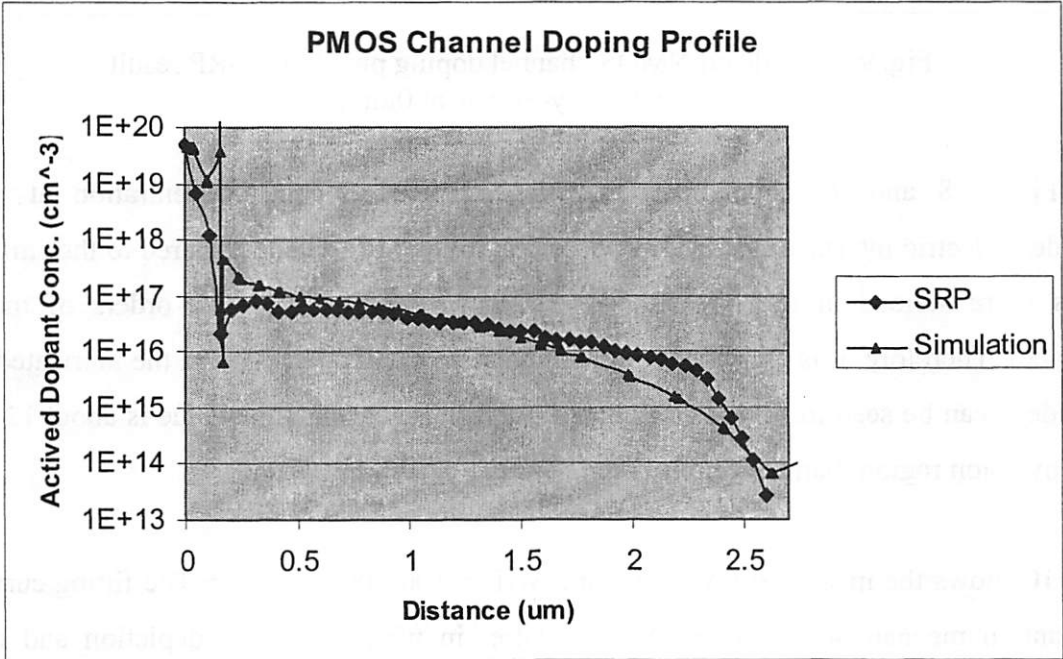
Fig. 8 - Simulated PMOS channel doping profile vs. SRP result Plot starts with poly-Si gate at 0μm distance.
