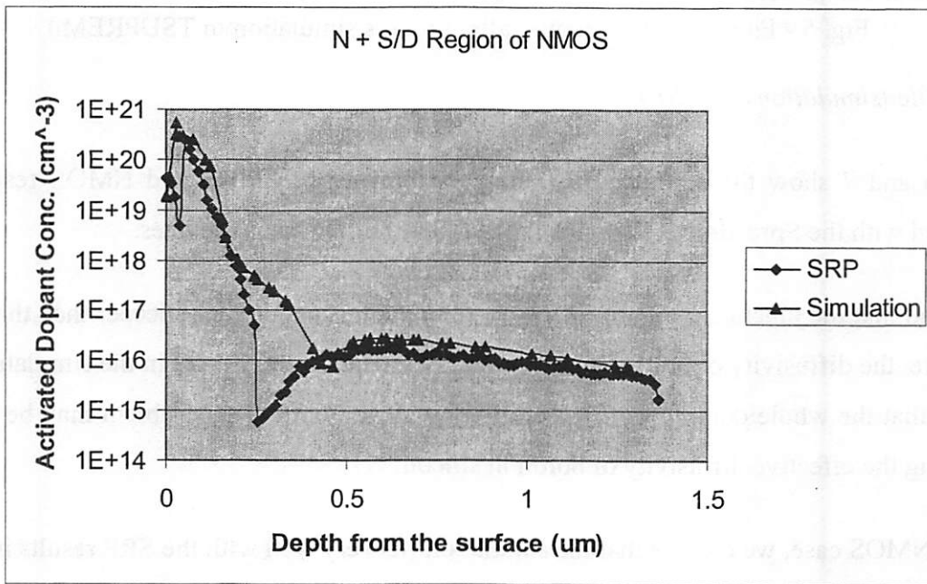
Fig. 7 - Simulated S/D junction profile of NMOS vs. SRP result The drop at the surface is the region where silicide is formed.
