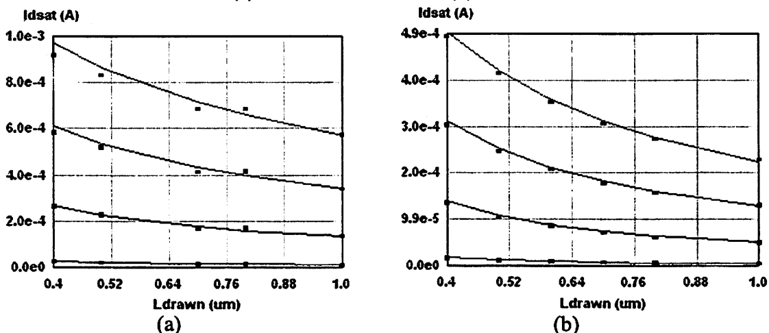
Fig. 24 - Saturation current vs. channel length at V_{bs}=0\text{V} with gate bias (a) 1 to 4V for NMOS; (b) -1 to -4V for PMOS
