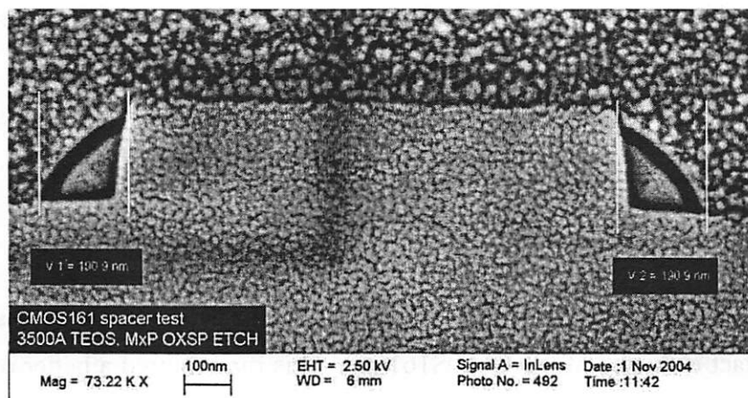
Fig. 1 – SEM cross-section of a sample prepared for sidewall spacer analysis
