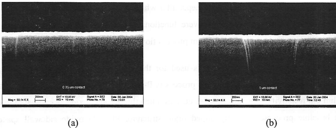
Fig. 2 - SEM cross section of 0.35µm (a) and 1µm (b) contact holes etched in 1.5µm thick LTO Lithography was done on ASML 5500/90, and etch was done in Centura MxP+
