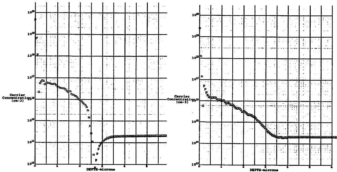
Fig.13 - P-channel (left) and N-channel (right) doping profile under the gate oxide
