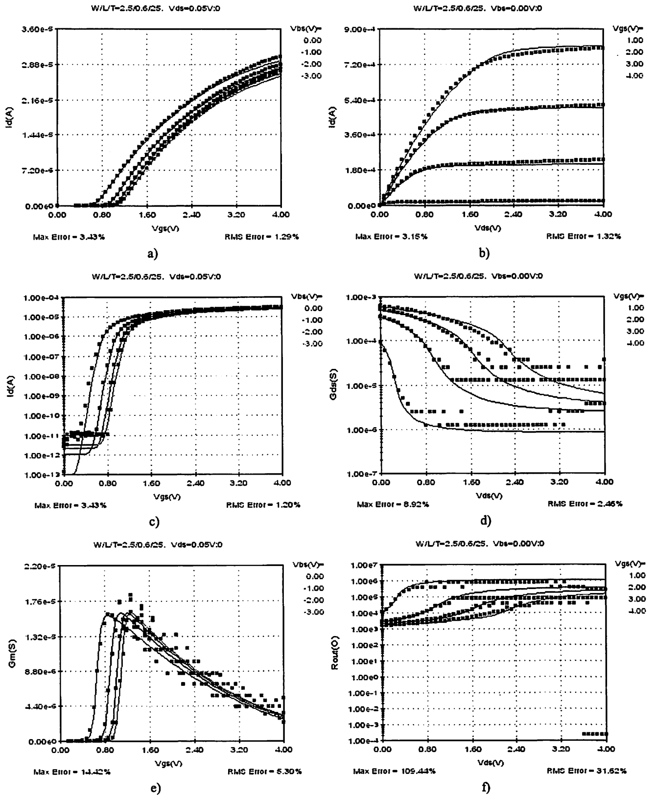
Fig 28 - L=0.6um W=2.5um NMOS
