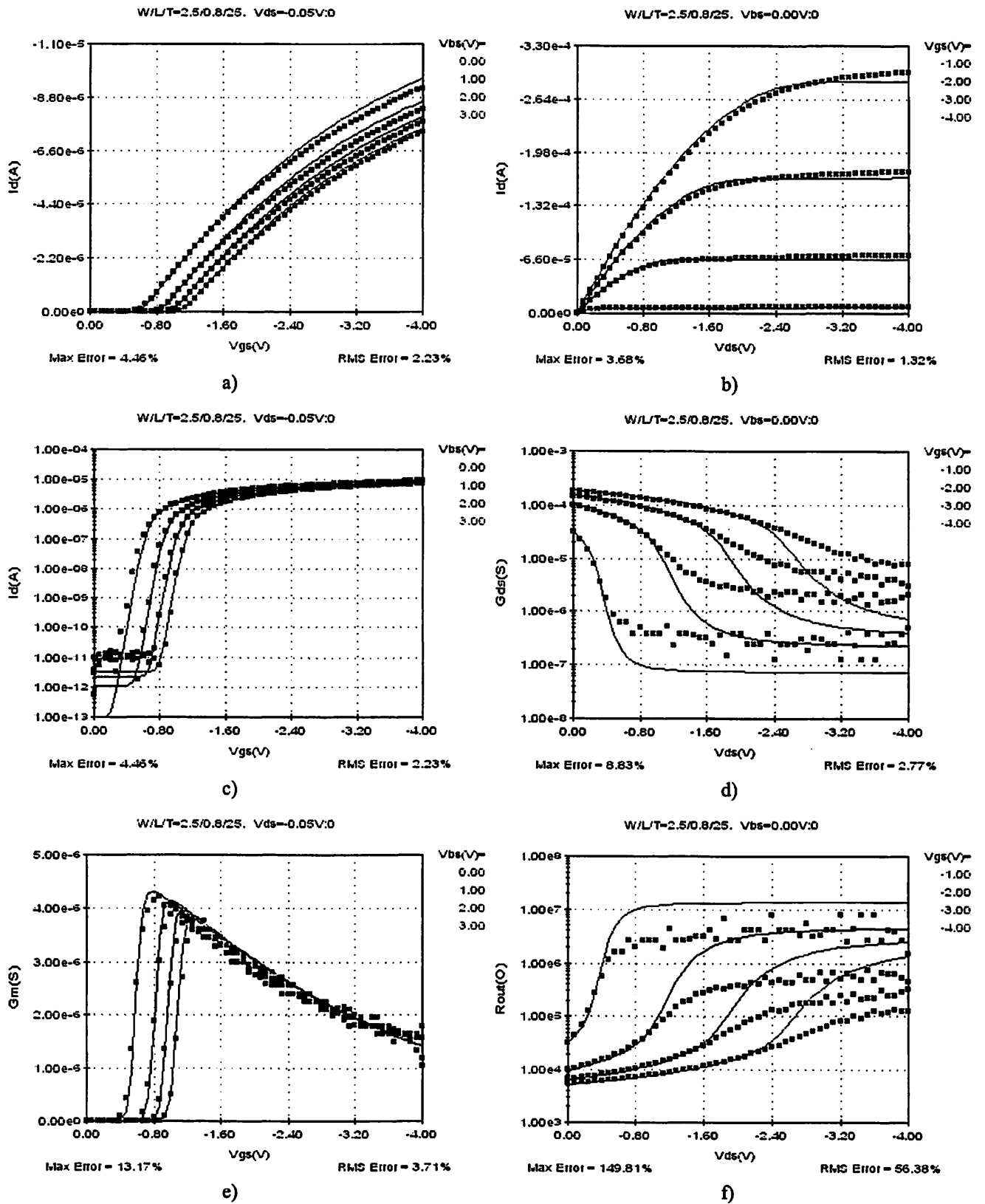
Fig 37 - L=0.8um W=2.5um PMOS
