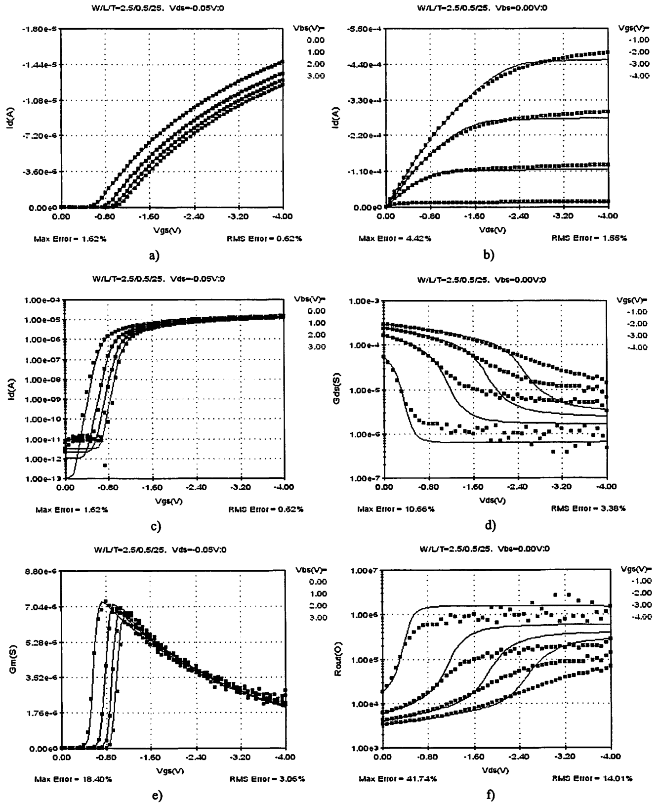
Fig 34 - L=0.5\mu\text{m} W=2.5\mu\text{m} PMOS
