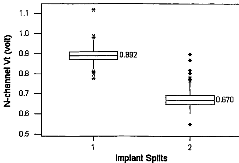
Fig. 19 - Threshold voltages in NMOS split groups: NMOS split group #1: Wafers #4, 5, 6, 7, 8 (NVt implant dose 6E12) NMOS split group #2: Wafers #1, 2, 3, 9, 10 (NVt implant dose 4E12)
