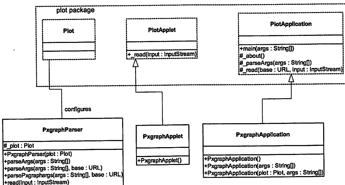
FIGURE 6.10. The compat package provides compatibility with the older pxgraph program.
