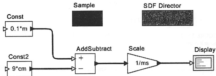
FIGURE 3.7. A model that uses the sample unit system.
