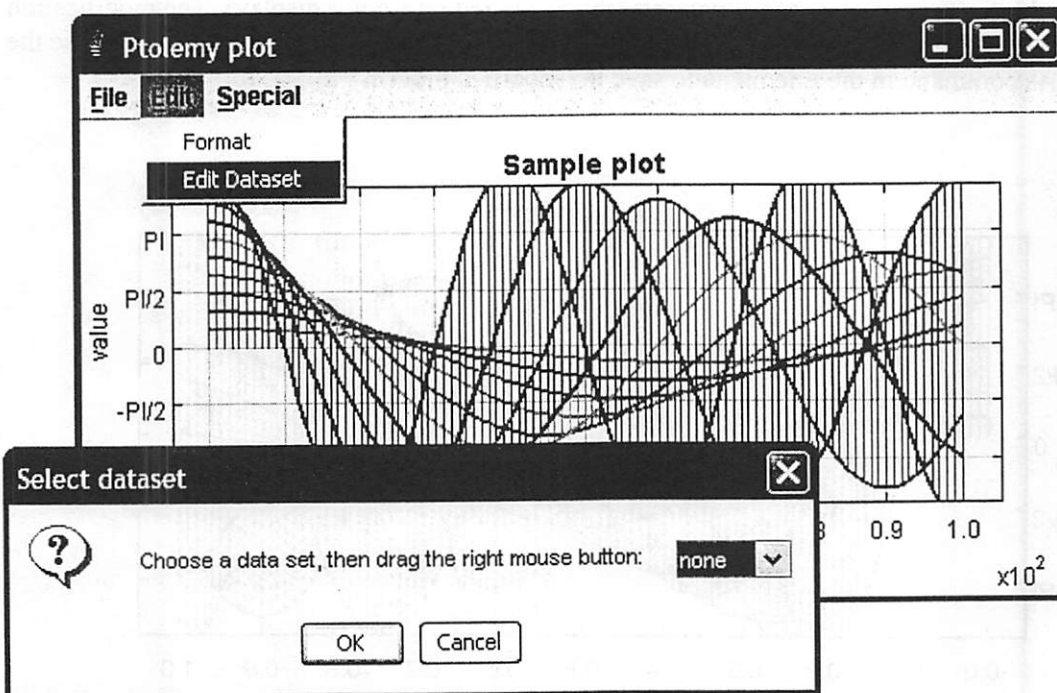
FIGURE 6.4. You can modify the data being plotted by selecting a data set and then dragging the right mouse button. Use the Edit menu to select a data set. Use the Save command in the File menu to save the modified plot (in PlotML format).
