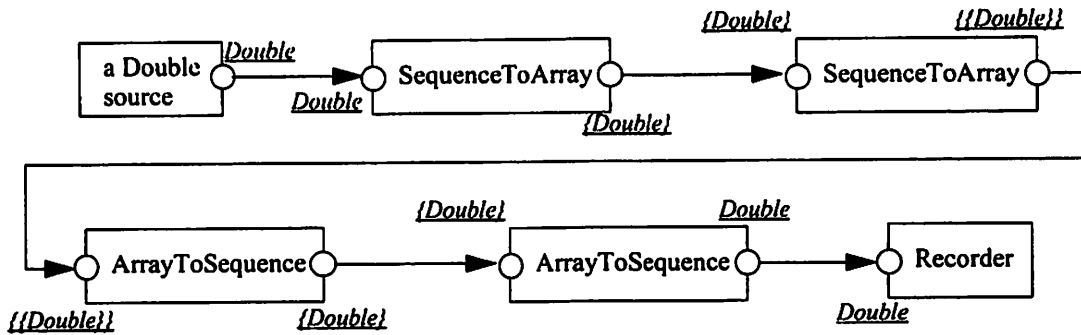
FIGURE 5.7. Conversion between sequence and array.
