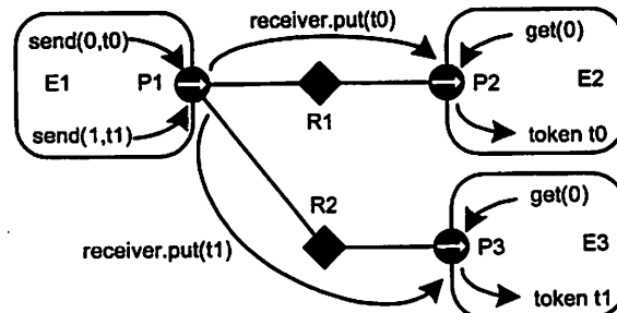
FIGURE 2.3. A port can support more than one channel, permitting an entity to send distinct data to distinct destinations via the same port. This feature is typically used when the number of destinations varies in different instances of the source actor.
