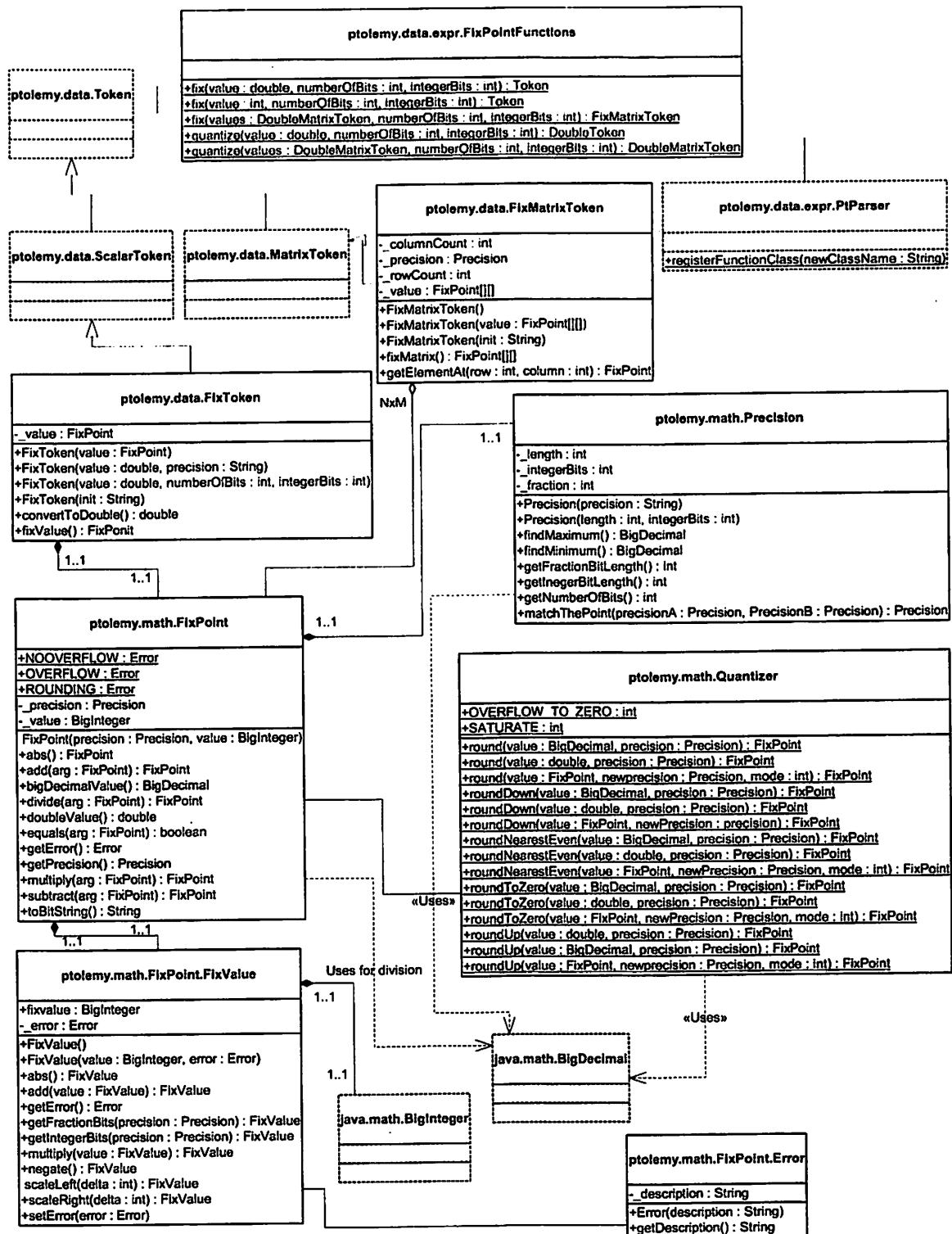
FIGURE 3.2. Organization of the FixPoint Data Type.
