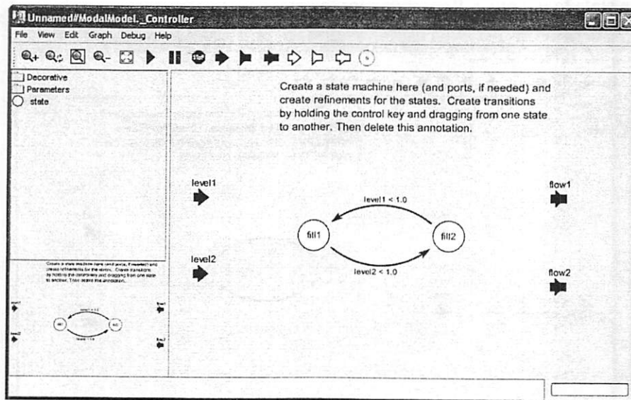
FIGURE 73. State machine with guards on the transitions.
