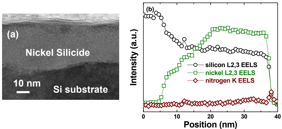
Figure 4.18 (a) Cross-sectional high resolution TEM (HRTEM) micrograph of the sample that received the nitrogen implant. No clear evidence of an interfacial layer is observed, (b) No nitrogen signal is observed in the electron energy loss spectroscopy (EELS) scan at the interface between the Si substrate and the NiSi layer.
