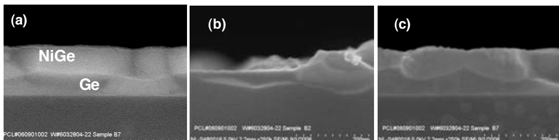
Figure 5.12 Cross-sectional SEM images after NiGe etching in SPM and 20% \text{H}_2\text{SO}_4 : (a) NiGe film after germanidation, (b) after exposure to SPM, (c) after exposure to 20% \text{H}_2\text{SO}_4 . Thus 20% \text{H}_2\text{SO}_4 can be successfully used to remove nickel with high selectivity.
