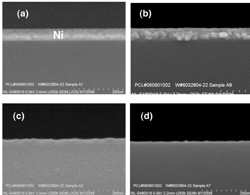
Figure 5.11 Etching characteristics of nickel film in SC1, SPM and 20% \text{H}_2\text{SO}_4 : (a) sputtered nickel film on Si substrate; (b) after exposure to SC1; (c) after exposure to SPM; (d) after exposure to 20% \text{H}_2\text{SO}_4 .
