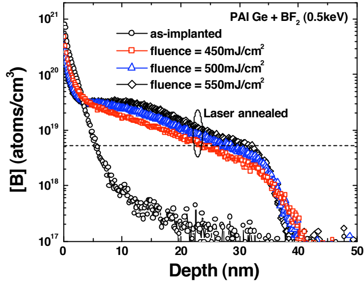
Figure 2.21 SIMS profiles of BF 2 (0.5keV, 5 \times 10^{14} \text{ cm}^{-2} ) implant before and after laser anneal. Laser fluence of 450 mJ/cm 2 , 500mJ/cm 2 , or 550mJ/cm 2 was used to activate dopants.
