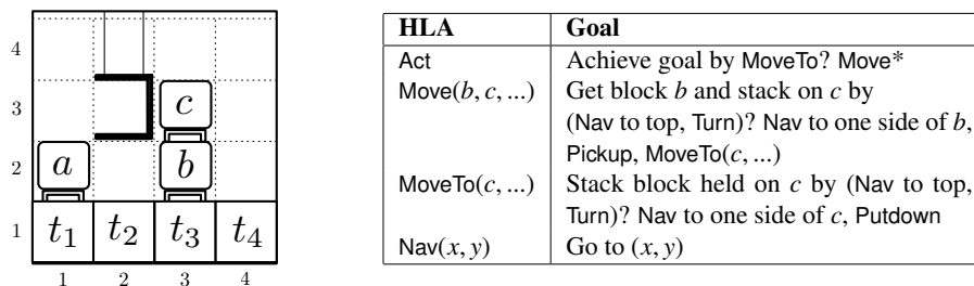
Figure 3: Left: A 4x4 warehouse world problem with goal \text{ON}(c, t_2) \wedge \text{ON}(a, c) . Right: HLAs for warehouse world domain.
