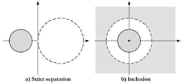
Fig. 1. Two special cases for handling non-convex constraints: (a) by adding a negated RCC a new set is generated that is strictly separated from the previous convex set; (b) the negated RCC generates a set that totally includes the previous convex set.
