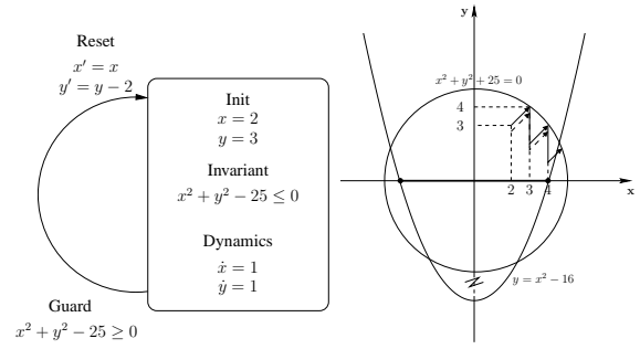
Fig. 5. Simple hybrid automata with convex guards and invariants (left) and representation of the error traces from CalCS (solid) and iSAT (dashed) in the (x, y) plane (right). The safety interval for x is [-4, 4] .
