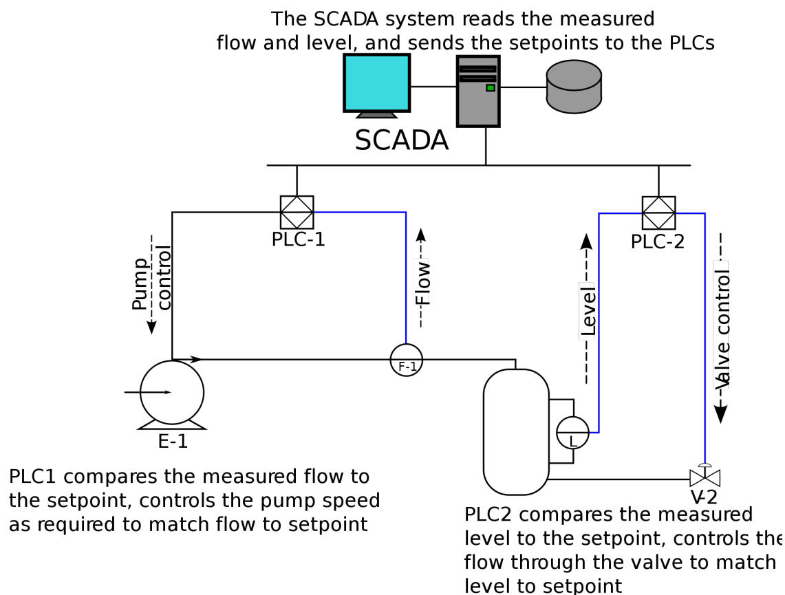
Figure 2.4: SCADA is a supervisory system where a central host controls set-points and remote terminal units (RTUs) perform local decisions. Image source:[82].
