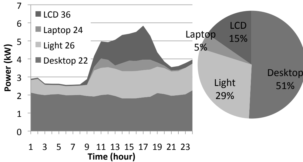
Figure 8.2: Stacked graph of aggregate power consumption grouped by functional class over a day.
