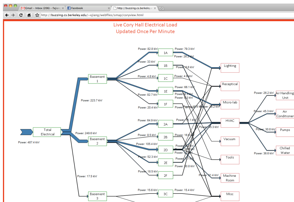
Figure 8.10: A live Sankey diagram showing the energy flows in the building electrical load tree.
