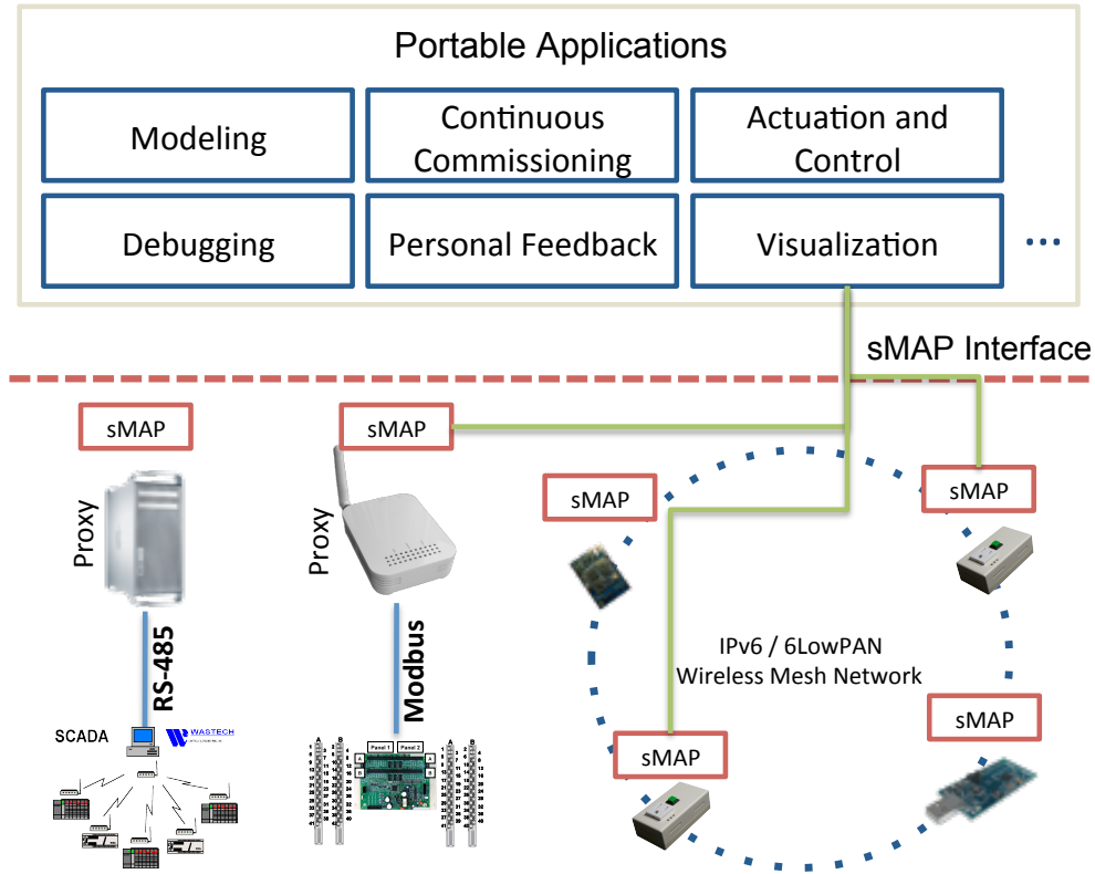
Figure 5.5: IPv6-based sensors such as ACme’s implement sMAP directly while legacy devices such as Modbus based branch meters implement sMAP via proxies. Applications interface with any metering resource uniformly via sMAP. In this example, a visualization application is used to graph real-time energy readings from both ACme’s and from branch meters.
