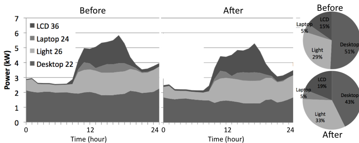
Figure 9.7: Estimated saving of the laboratory energy consumption if all of the desktops incorporated energy management software.
