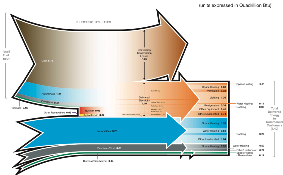
Figure 2.1: Energy end-use flow maps for the commercial buildings. Image source: [29].
