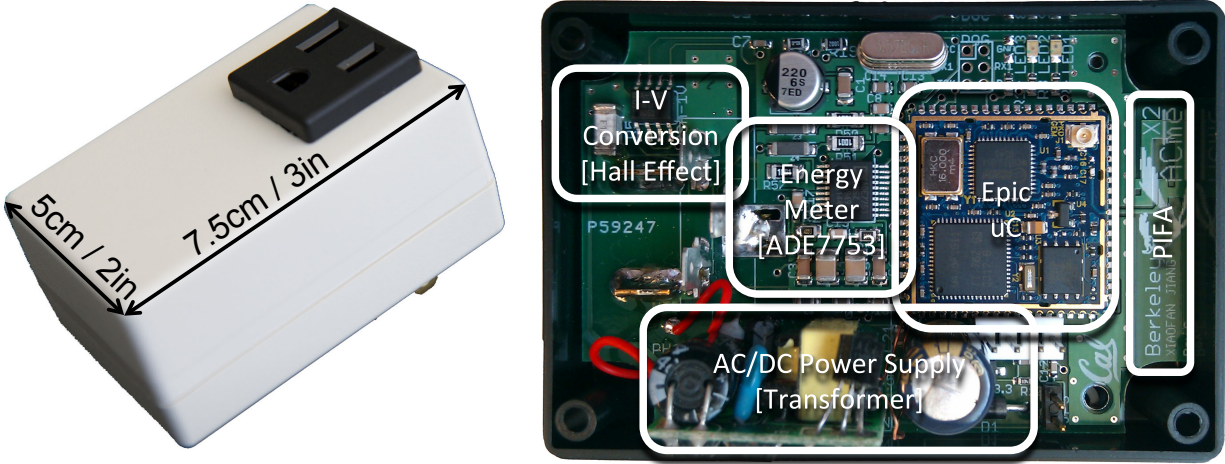
Figure 4.5: ACmeX2 is more compact and efficient but does not include relay.
