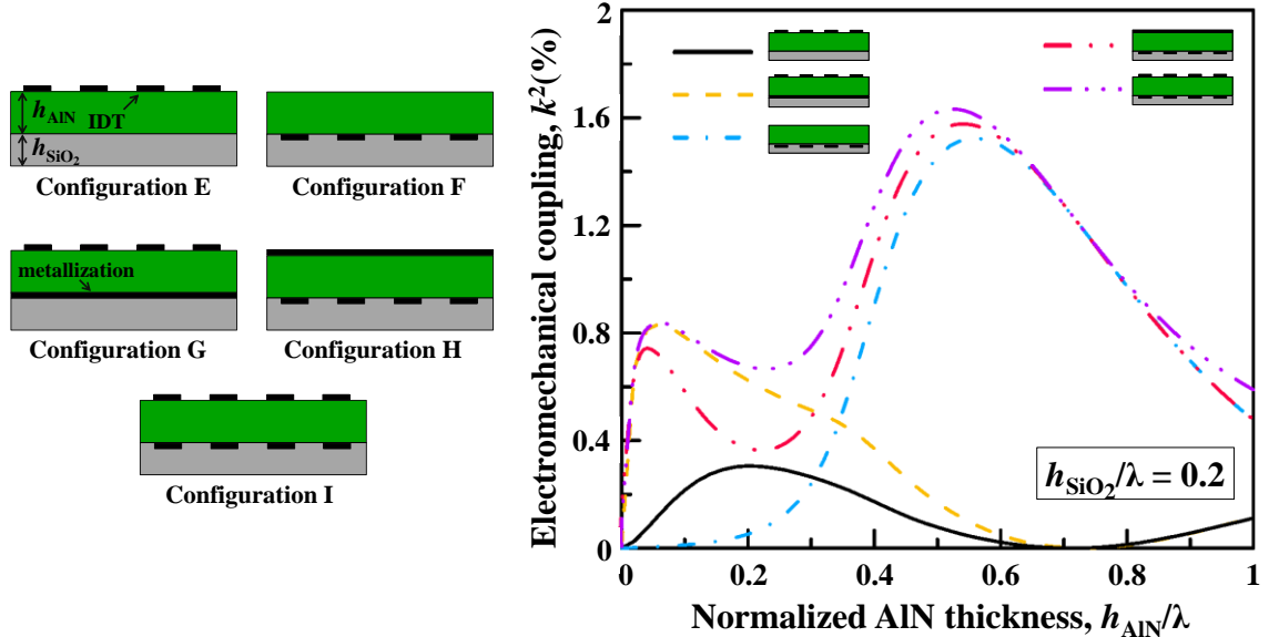
Figure 3-10. Calculated electromechanical coupling coefficients of the QS_0 mode for different electrode configurations listed when h_{\text{SiO}_2}/\lambda=0.2 .
