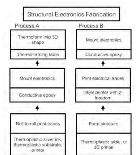
Figure 4.1: Two major fabrication methods used to fabrication structural electronics. Process A starts with the circuit fabricated on a flat thermoplastic sheet first, and the 3D structure is thermoformed with the circuit encapsulated. Process B starts with a 3D printed structure, and relies on a printer with z-axis freedom to print the circuit.
