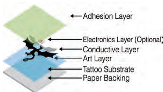
Figure 6.4: An illustration of the different layers of a basic Skintillate device.
