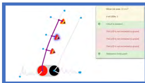
Figure 7.8: Validation tool checks for errors in the electrical design before the user fabricate the circuit. This figure shows
