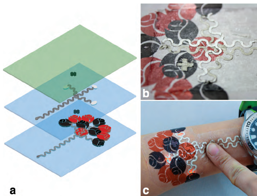
Figure 6.10: Skintillates Display. a) An exploded illustration of the different layers: a bottom layer consists of the basic Skintillates art and conductive layer, while a second conductive layer is connected to the first layer through vias and the adhesive layer. b) a photograph of the two overlaying but insulated conductive layers, c) the multilayer display under operation while being compressed, showing that it maintains functionality while being flexed.
