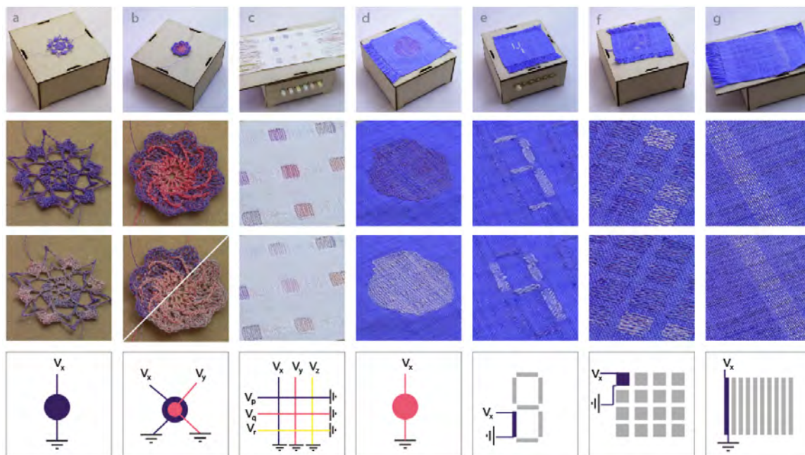
Figure 5.4: Swatches created from Ebb. a) density crochet, b) multicolor crochet, c) woven color-mixing gingham, d) woven graphic element, e) woven seven-segment, f) woven grid, and g) woven stripes. The bottom row shows the wiring diagrams for each swatch. On schematics e-g, grey elements each utilized identical wiring as the featured blue element.
