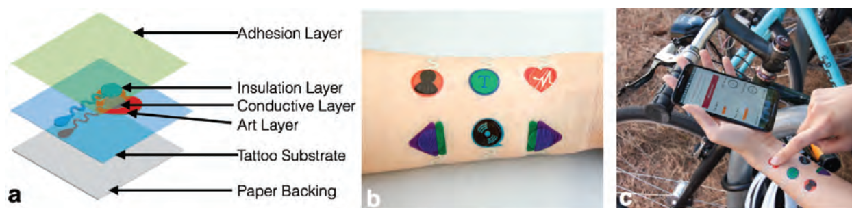
Figure 6.11: Skintillates Capacitive touch sensing. a) an exploded illustration of a Skintillates capacitive sensor showing one additional insulation layer on top of the conductive layer to prevent charges on skin from interfering with the capacitive touch signal, b) capacitive sensors can be applied on body locations convenient to the wearer; in this case, the inner arm, c) the Skintillates capacitive buttons were used to control a mobile device when the user was active and could not directly access the device screen.
