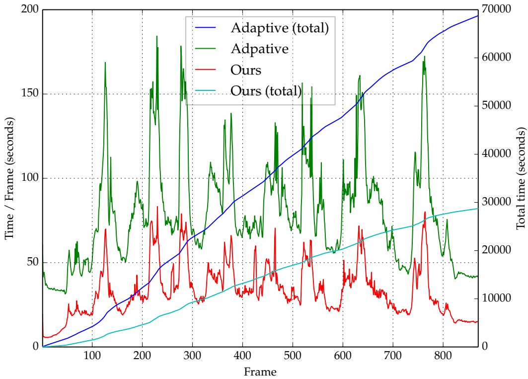
Figure 5: A comparison of view-independent and view-dependent adaptive simulations for the example of Figure 1 in terms of per-frame and cumulative simulation times.
