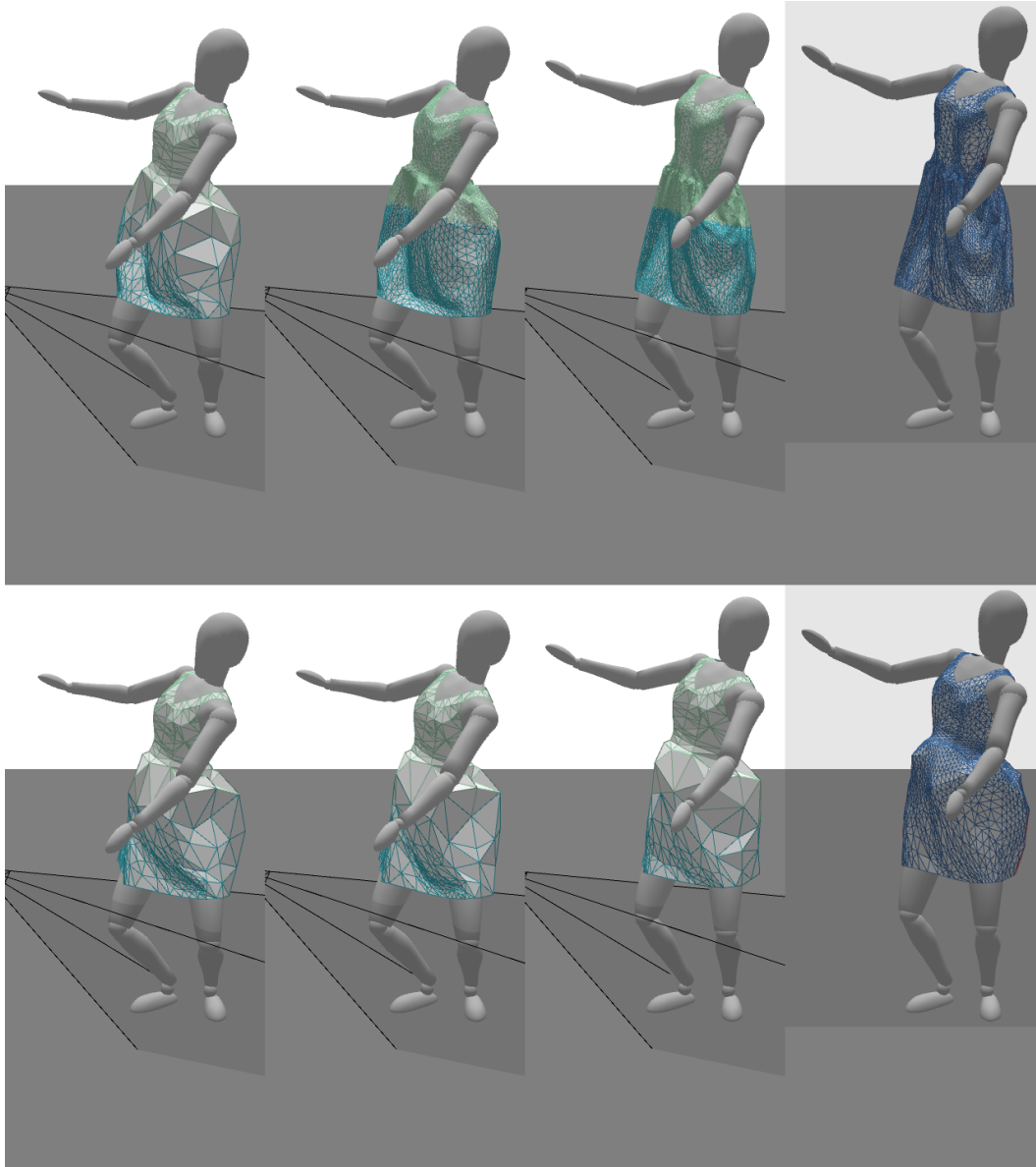
Figure 3: A sequence of frames with a jump cut, showing a dress simulated with temporal anticipation (above), and without (below). Blue edges indicate faces visible in the current view. Temporal anticipation allows the cloth to reach the correct high-resolution state before it becomes visible.
