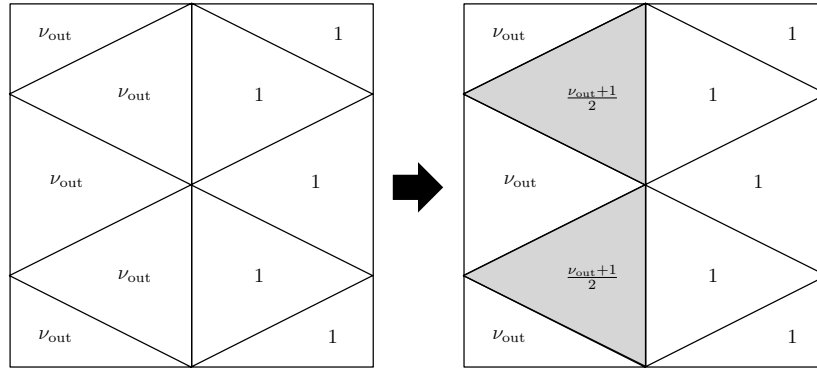
Figure 4: Locally interpolating discontinuous view factors at silhouettes to ensure smooth silhouettes.
