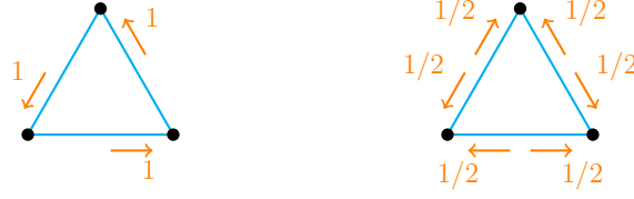
Figure 6.3: A graph with 3 vertices and three edges and two different balanced allocations with zero baseload. Note that the total load at each vertex is the same for the two allocations and is equal to 1 at each vertex.
