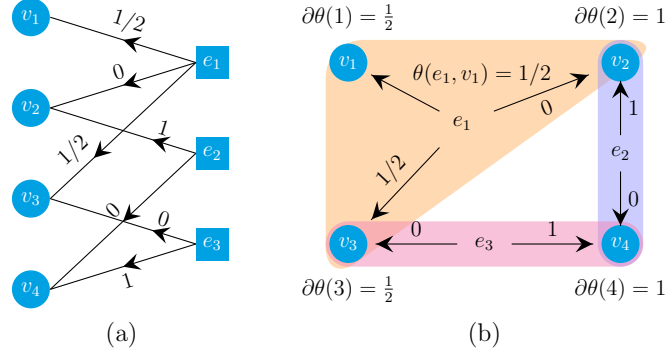
Figure 6.1: Load balancing with 3 tasks and 4 servers. (a) illustrates the bipartite representation together with an allocation. While the load of e_1 could be served by nodes in \{v_1, v_2, v_3\} , half of its load is being assigned to v_1 and the other half to v_3 , i.e. \theta(e_1, v_1) = 1/2 , \theta(e_1, v_2) = 0 and \theta(e_1, v_3) = 1/2 . (b) shows the hypergraph representation. The total load at a node i is denoted by \partial\theta(i) . For instance, \partial\theta(v_3) = \theta(e_1, v_3) + \theta(e_3, v_3) = 1/2 .
