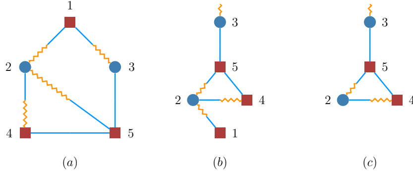
Figure 2.3: (a) A marked graph G on the vertex set \{1, \dots, 5\} with vertex mark set \Theta = \{\bullet, \blacksquare\} and edge mark set \Xi = \{\text{Blue (solid)}, \text{Orange (wavy)}\} . In (b), G(1, 3) is illustrated where the first component \xi_G(1, 3) is depicted as a half edge with the corresponding mark going towards the root 3, and (c) illustrates G(1, 3)_2 . Note that G(1, 3) can be interpreted as cutting the edge between 1 and 3 and leaving the half edge connected to 3 in place. Moreover, note that, in constructing G(u, v) , although we are removing the edge between u and v , it might be the case that u is still reachable from v through another path, as is the case in the above example.
