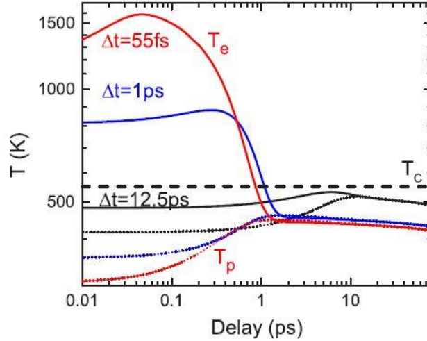
Figure 3.12 Transient electron and lattice temperatures of GdFeCo for different for different pump pulse durations.
