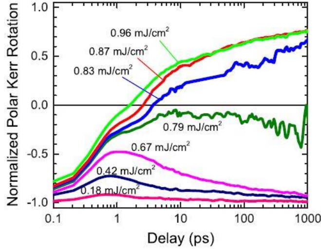
Figure 3.10 Magnetization dynamics of Gd 24 FeCo for different pump fluences.
