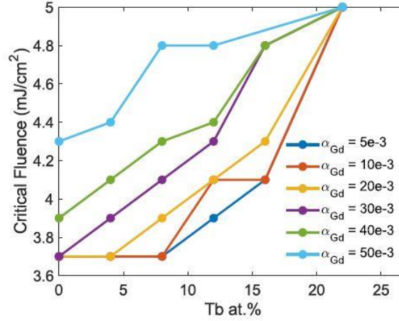
Figure 4.11 Simulated critical fluence for different Tb concentrations.
