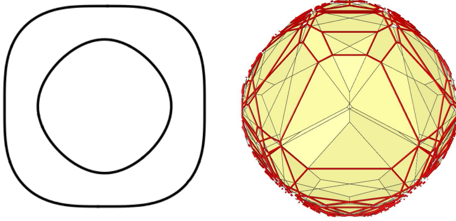
Figure 5.7: A quartic spectrahedron (left) and its second Voronoi decomposition (right). The Schottky locus of that spectrahedron consists of those edges that are highlighted in red.
