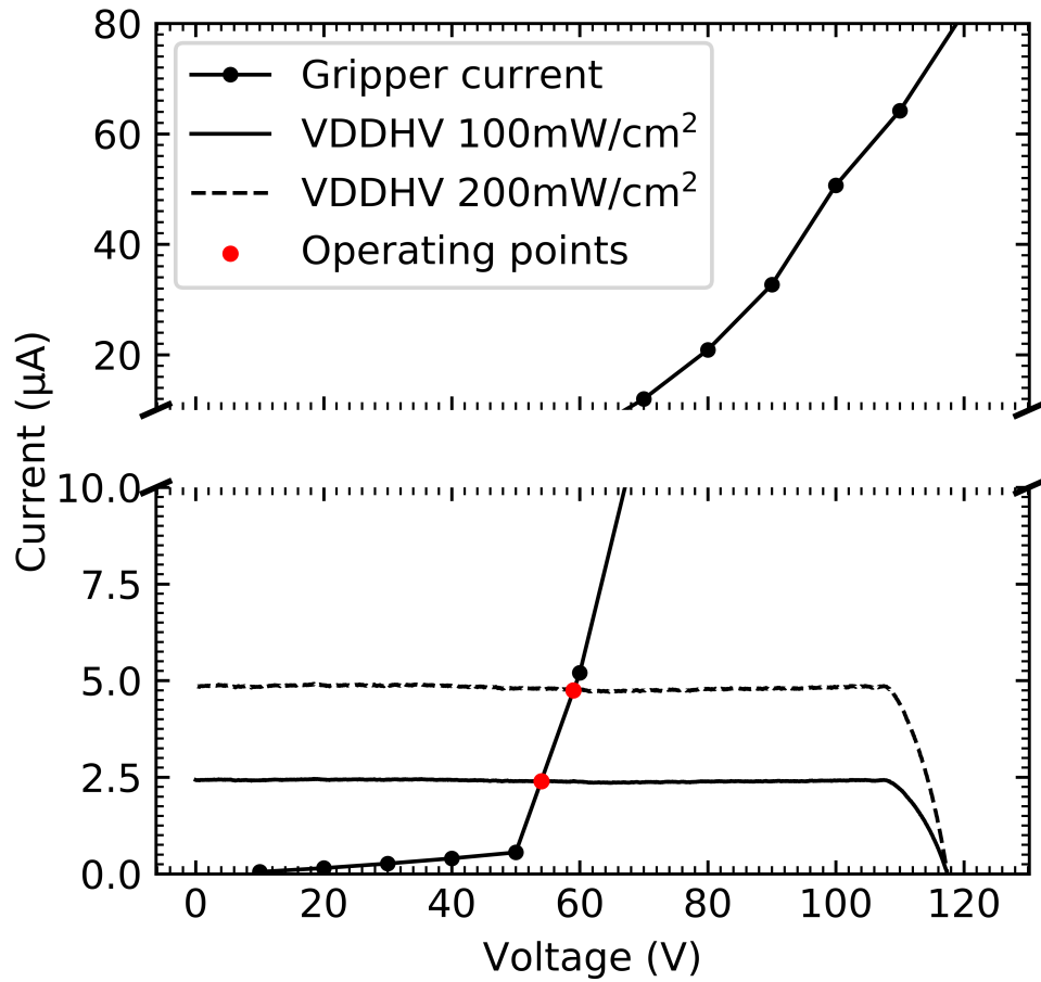
Figure 3.5: Measured gripper leakage current under DC supply vs. HV buffer DC voltage, and Zappy2 VDDHPV supply current vs. VDDHPV voltage under 100 \text{mW}/\text{cm}^2 (measured) and 200 \text{mW}/\text{cm}^2 irradiation (estimated). Red intersections represent operating points of the system at 100 \text{mW}/\text{cm}^2 and 200 \text{mW}/\text{cm}^2 irradiation while closing the gripper at very slow speeds approaching zero and duty cycles approaching 100%.
