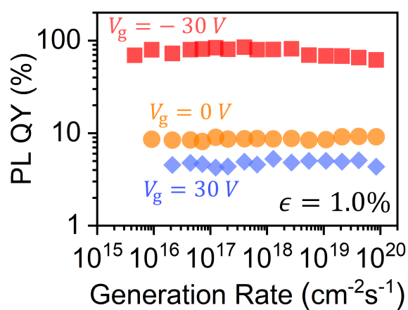
Figure 3.5: Near-unity PL QY in \text{WS}_2 at all generation rates. PL QY of monolayer \text{WS}_2 as a function of gate voltage and generation rate at 1.0% strain.
