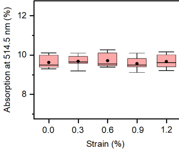
Figure 3.2: Absorption at excitation wavelength under applied strain. Absorption of monolayer \text{WS}_2 as a function of applied strain at pump laser wavelength ( \lambda = 514.5 nm).
