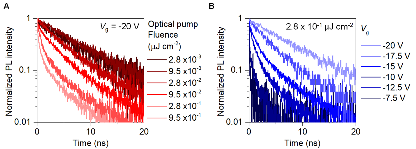
Figure 2.9: Time-Resolved PL of the MoS 2 under different optical pump fluence and V_g . (A) Time-resolved PL emission under different optical pump fluence at V_g = -20 V. (B) Time-resolved PL of the MoS 2 monolayer under different V_g at an optical pump fluence of 2.8 \times 10^{-1} \mu\text{Jcm}^{-2} . Note that the lifetime for V_g greater than -7.5 V is shorter than the instrument response function width.
