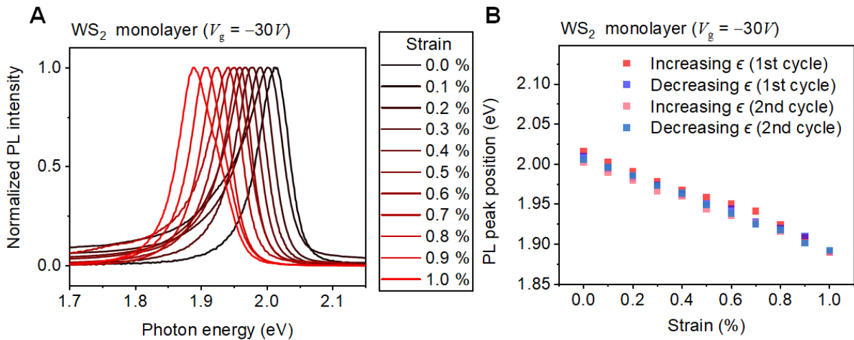
Figure 3.4: PL peak position shift of monolayer WS_2 . (A) Normalized PL intensity of monolayer WS_2 at V_g = -30V as a function of applied strains. (B) PL peak position during multiple bending and release cycles.
