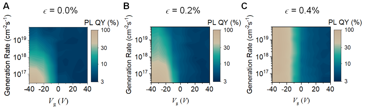
Figure 3.3: PL QY versus G and V_g in WS_2 at different strains. A color plot of PL QY in monolayer WS_2 as a function of gate voltages and generation rate with applied strains.
