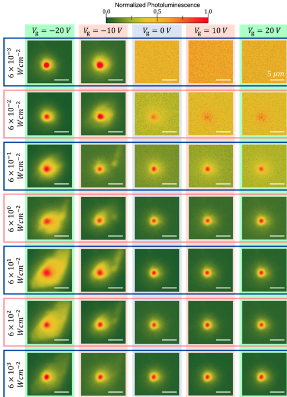
Figure 4.3: PL images at various pump powers and gate voltages. PL excited by a CW laser focused on a diffraction-limited spot for various pump powers and gate voltages. Images in the same row have the same pump power, and in the same column have the same gate voltage. Scale bar is 5 \mu m . Radial anisotropy arises from the finite size of the monolayer.
