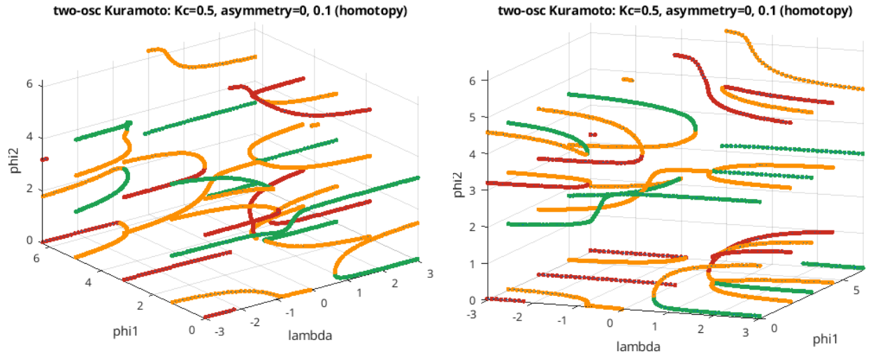
Fig. 21: Homotopy curves for J = \begin{bmatrix} 0 & 0.10 & 3.34 \\ 0.10 & 0 & -2.28 \\ 3.34 & -2.28 & 0 \end{bmatrix} , K_s = \frac{1}{2} , and \tilde{\alpha} = \begin{bmatrix} 0 \\ 0.1 \end{bmatrix} , from two angles.
