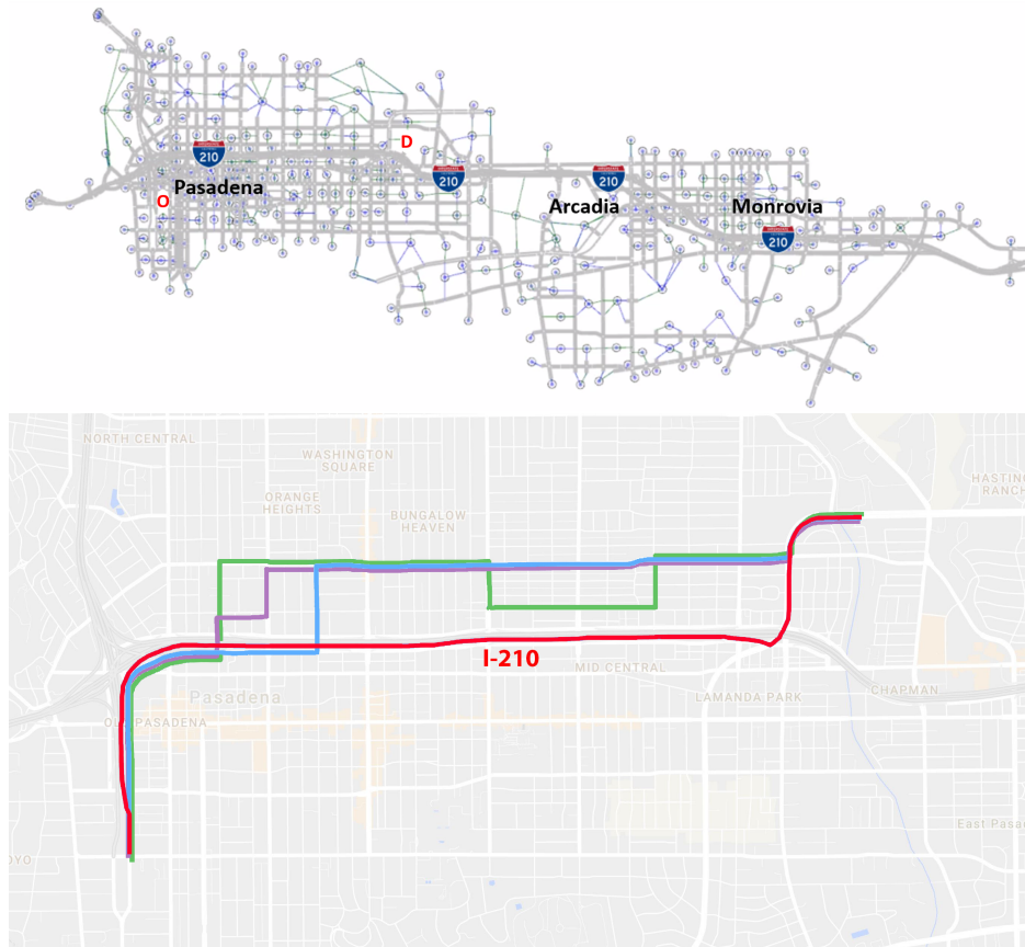
Figure 3.8: (a) The selected od pair for the Aimsun experiments. (b) A selection of alternate paths that app users took instead of the I-210 and the I-210 route (taken by non-app users) shown in red.
