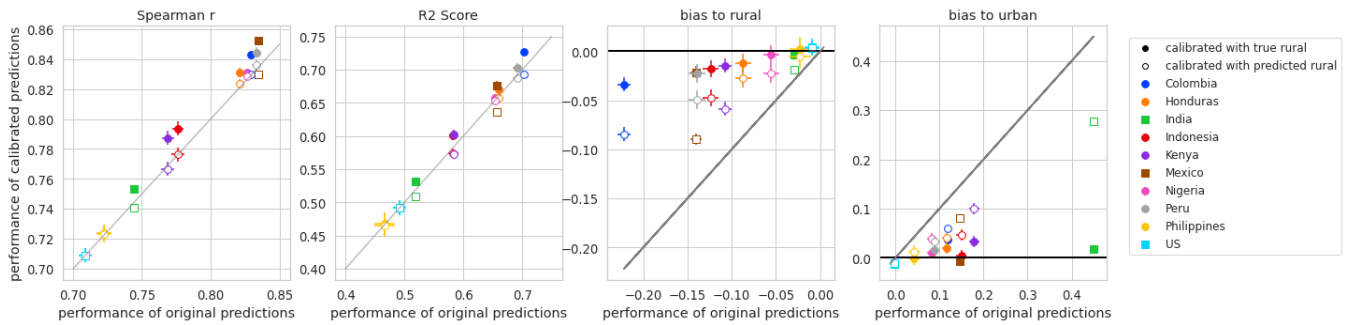
Figure S6: Additive recalibration by group raises the linear fit and rank correlation of overall predictions (leftmost two panels) and reduces statistical bias of predictions per-group (rightmost two panels).
