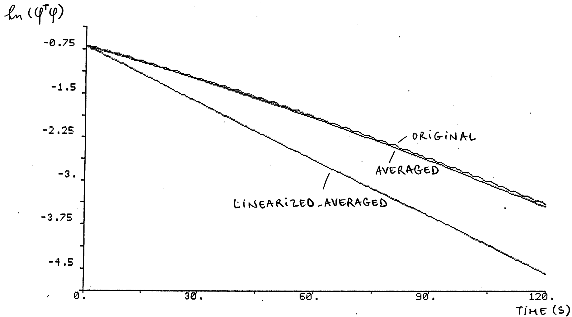
Fig 4 Logarithm of the Lyapunov Function
