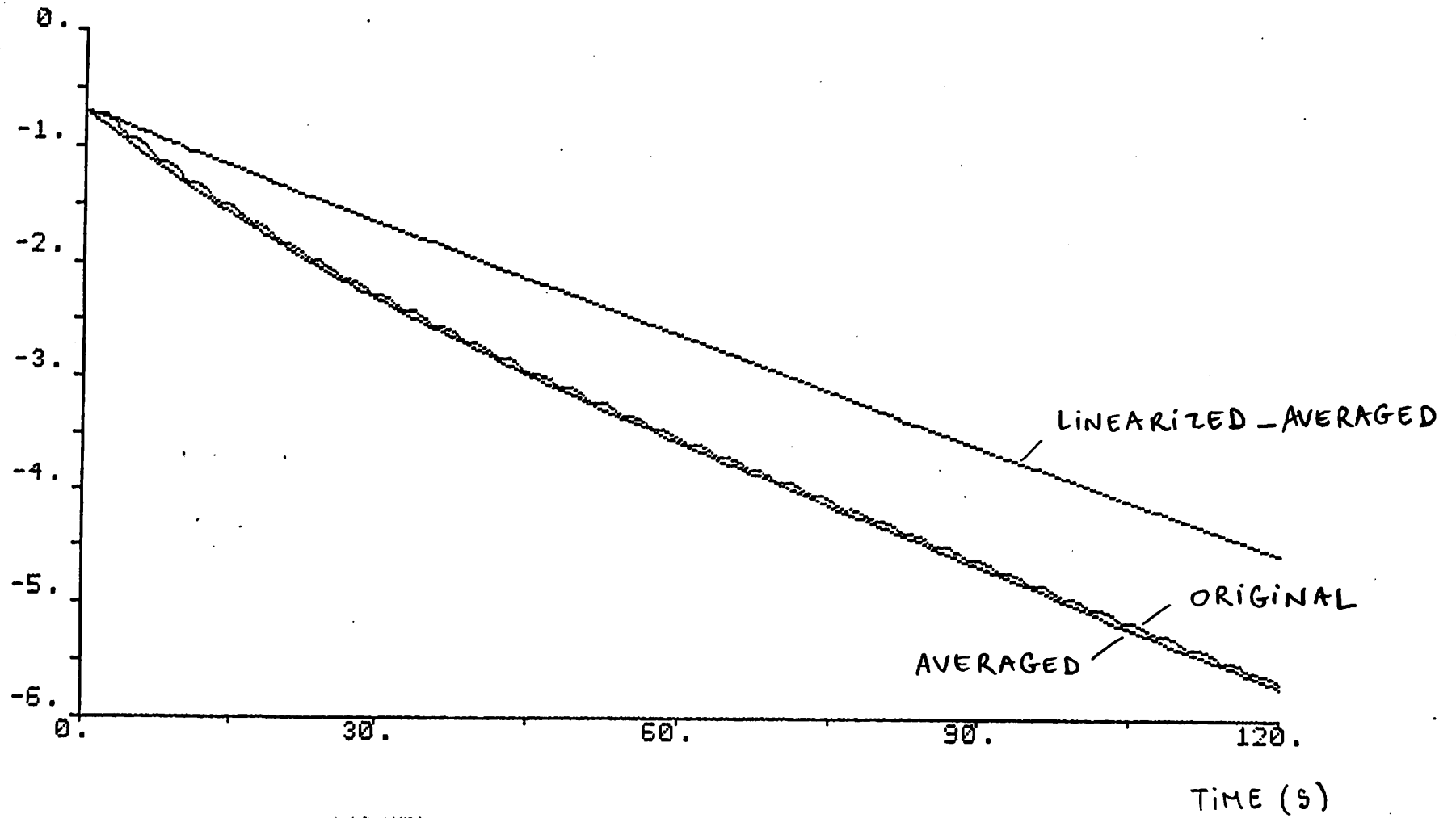
Fig 1 Logarithm of the Lyapunov Function
