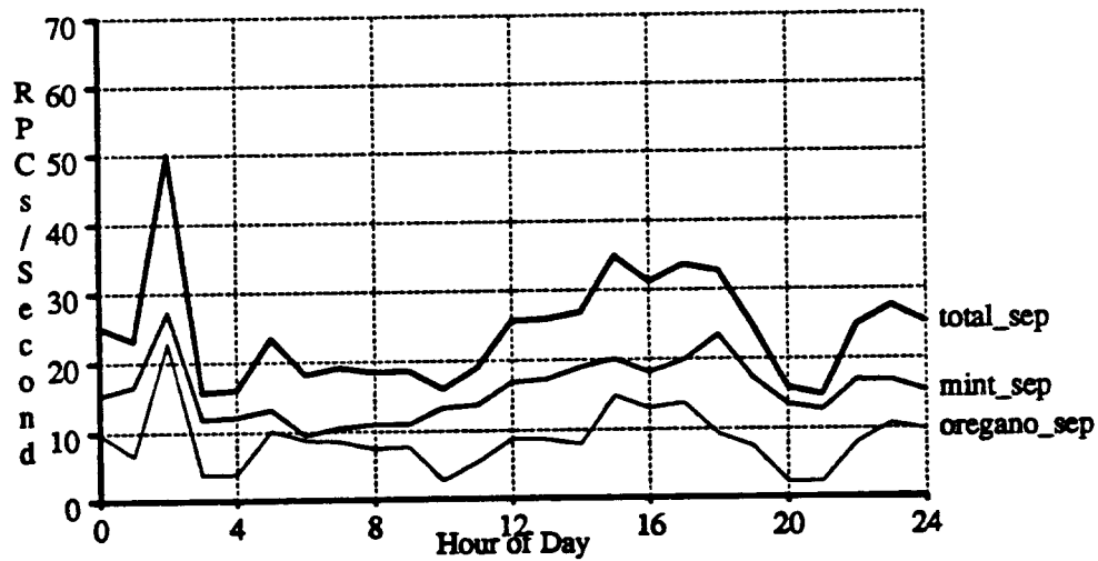
Figure B-8. RPC traffic for September. There were 25-27 clients in September. Assault, which is not shown, began servicing "/user2" September.
