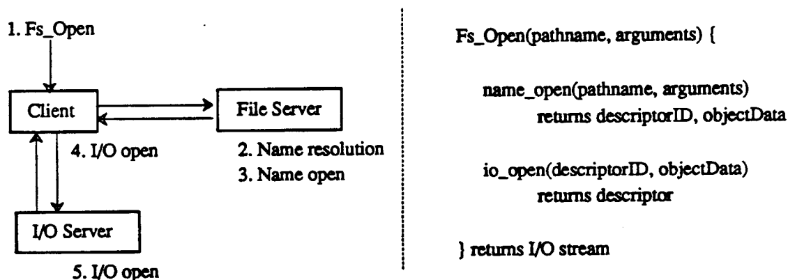
Figure 3-6. The flow of control during an Fs_Open operation. The arrows indicate invocation of the name resolution and the I/O open phases on the file server and the I/O server, respectively. In the most general case these operations are invoked using network RPC.
