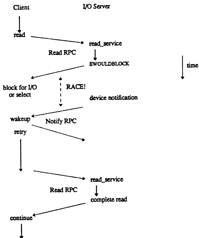
Figure 3-8. Message traffic during a blocking I/O. Control is returned to the client if an I/O operation would block. There is a potential race condition between the EWOULDBLOCK reply message and the notification message from the I/O server.
