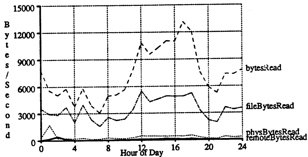
Figure B-12. Read traffic on Mint averaged from July 8 to December 22, 1989.
