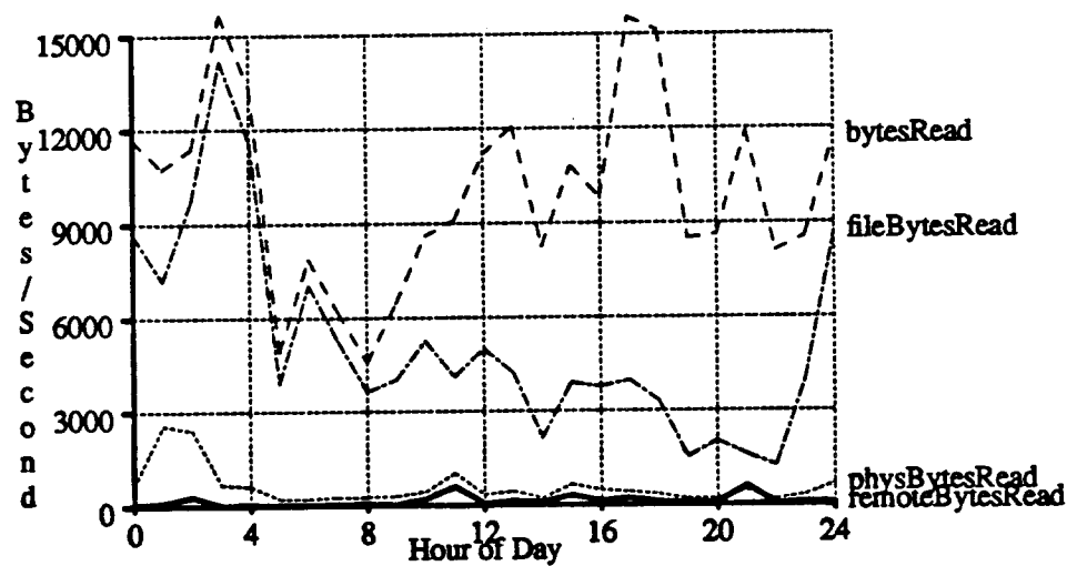
Figure B-13. Read traffic on Allspice averaged from October 5 to December 22, 1989.
