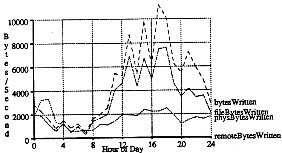
Figure B-17. Write traffic on Allspice averaged from October 5 to December 22, 1989. The sharp peaks reflect the copying of large directory structures from Oregon to Allspice in late October.
