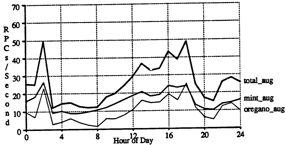
Figure B-7. RPC traffic for August. There were 15-25 clients in August. Allspice, which is not shown, began servicing "/user1" in August.
