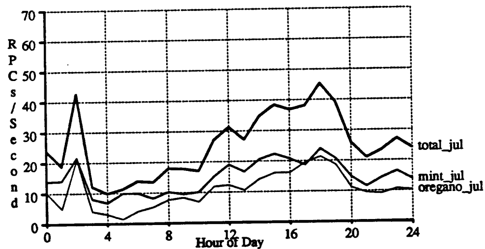
Figure B-6. RPC traffic for July. There were 12-15 clients in July. Allspice, which is not shown, began servicing "/swap" in July.
