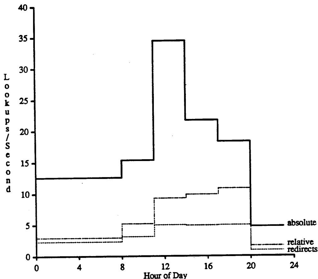
Figure 4-4. Lookup rates for 35 clients combined. The lookups are divided into those on absolute and relative pathnames. The rate of pathname redirections is also shown. These rates were computed from July 8 through Dec 22, 1989. Clients were sampled every three hours from 8:00 AM to 11:00 PM.
