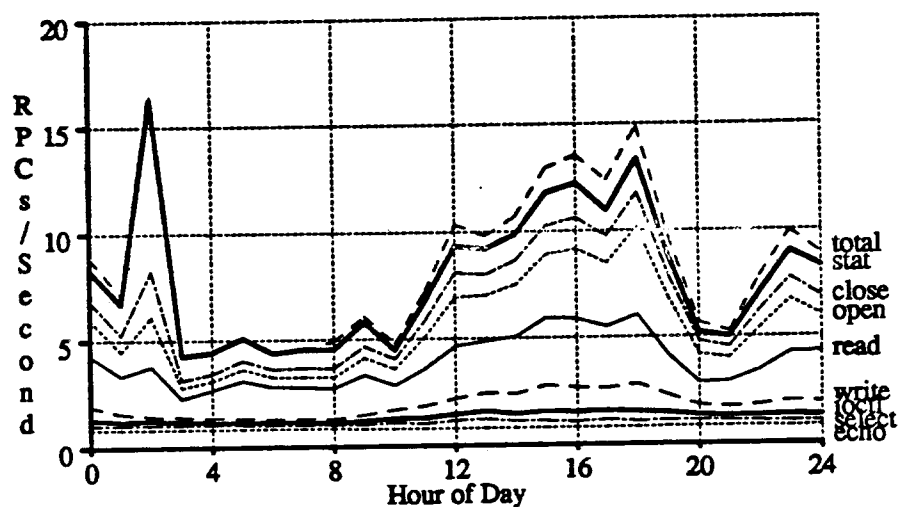
Figure B-3. RPC traffic for Oregon averaged from July 8 to December 22, 1989. Oregon is the server for "/tmp", some source code, and some commands.
