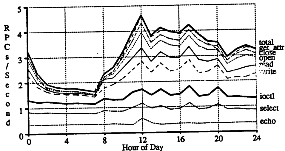
Figure B-5. RPC traffic for Sage averaged from July 8 to December 22, 1989. Sage is a Sun-3/75 client used by a Sprite developer.
