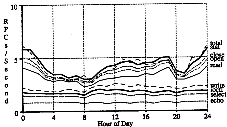
Figure B-4. RPC traffic for Assault averaged from September 13 to December 22, 1989. Assault is the server for some user directories.
