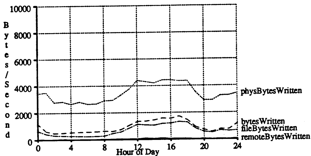
Figure B-16. Write traffic on Mint averaged from July 8 to December 22, 1989. Mint's write traffic is dominated by writes of descriptors for frequently updated files. This graph also highlights a bug that prevented continuously updated files from ever being written out (only their descriptor was written).
