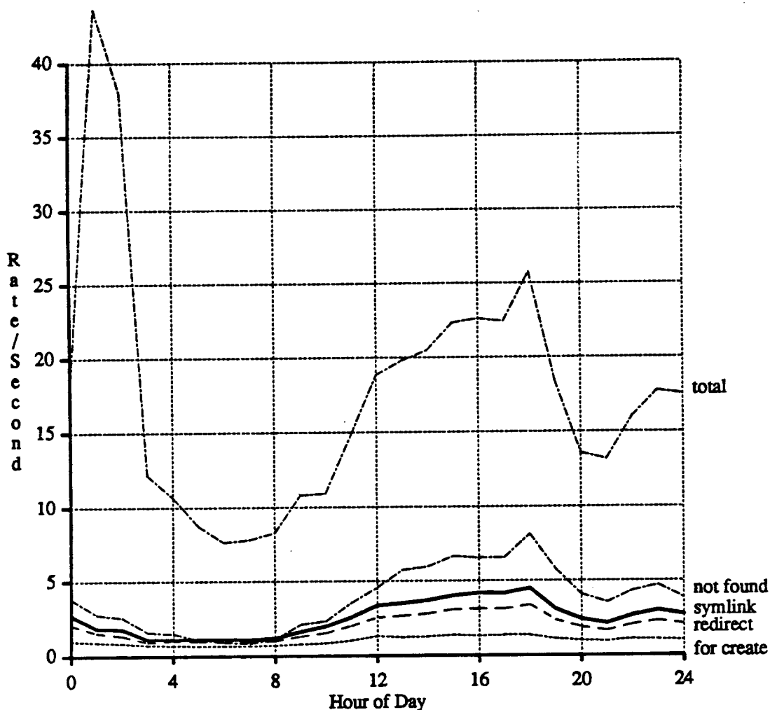
Figure 4-3. Lookup rates for the combination of all four file servers. The servers were measured from July 8 through December 22, 1989. Rates are shown for the total lookups, failed lookups (file-not-found), symbolic links traversed, pathname redirections, and open-for-create.
