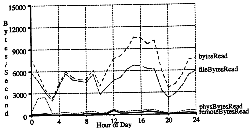
Figure B-14. Read traffic on Oregano averaged from July 8 to December 22, 1989.
