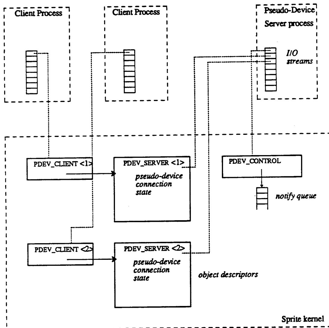
Figure 7-3. I/O streams between clients and a pseudo-device server. There is one pair of kernel object descriptors for each request-response channel between a client and the server. This channel is created each time a client makes an open on the pseudo-device. The PDEV_CLIENT descriptor is a stub that references the corresponding PDEV_SERVER descriptor; it is needed so that client I/O operations invoke different object-specific kernel procedures than the server. There is one PDEV_CONTROL stream for each pseudo-device, and this is used to notify the server about new PDEV_SERVER streams.
