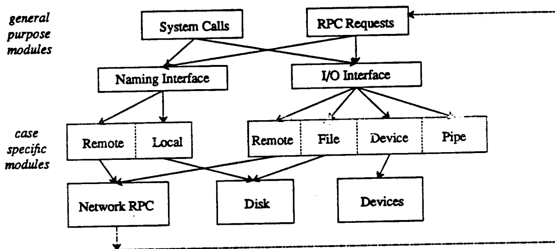
Figure 3-4. The modular organization of the file system architecture. There are two primary internal interfaces, one associated with operations on pathnames, and another associated with operations on I/O streams. General-purpose modules invoke object-specific modules through these interfaces, thus hiding the details associated with each case. Network requests are also dispatched through the internal interfaces in order to completely hide the use of RPC.
