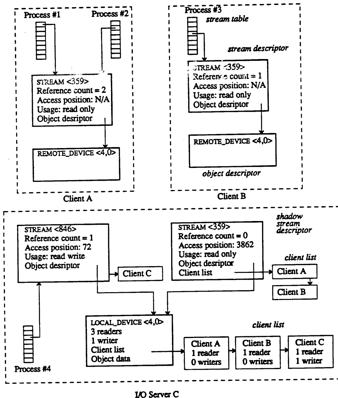
Figure 5-1. Streams and shadow streams. This is similar to Figure 3-6, except that stream #359 is now shared by processes on different hosts, and there is an additional shadow stream descriptor for this stream on the I/O server. The shadow stream descriptor has its own client list that is used to detect when the stream becomes shared by processes on different hosts.
