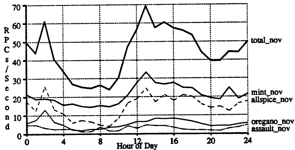
Figure B-10. RPC traffic for November. There were 29-33 clients in November. By this time many of the system source files previously on Oregano had been shifted to Allspice.
