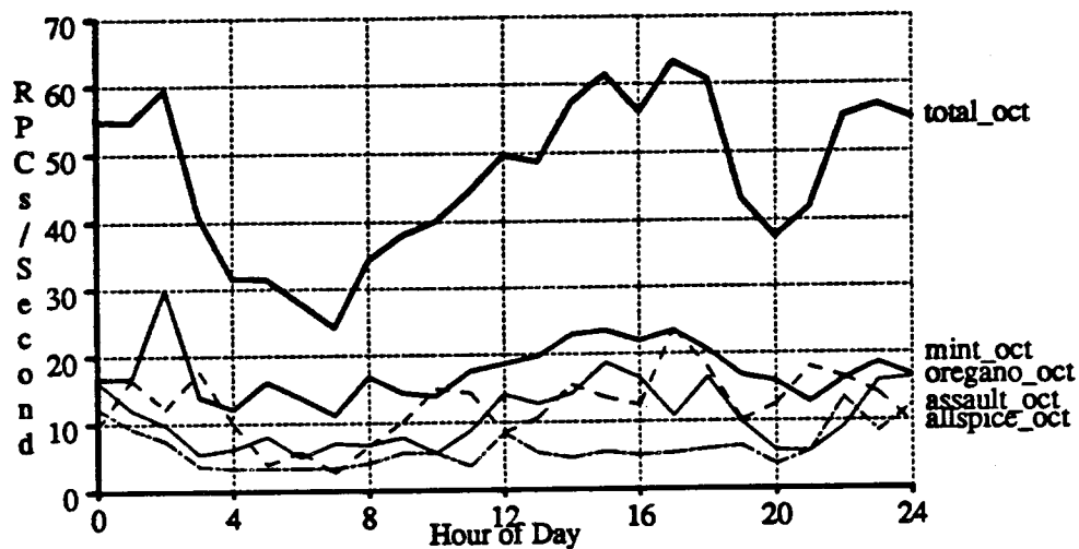
Figure B-9. RPC traffic for October. There were 27-29 clients in October.
