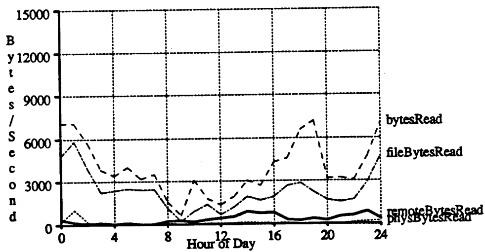
Figure B-15. Read traffic on Assault averaged from September 13 to December 22, 1989.
