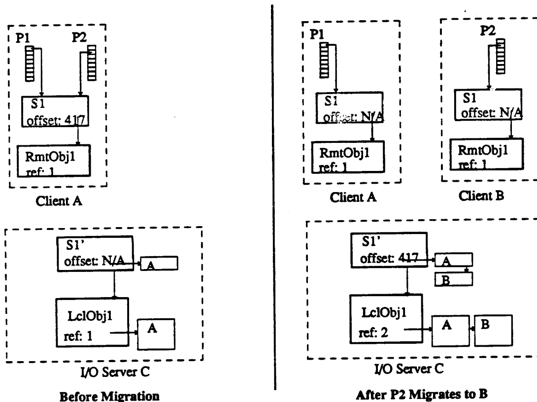
Figure 5-2. A stream may be shared by processes on different hosts after migration. Before the migration the I/O server only knows about the stream on one client, and the fact that the stream is shared by two processes is hidden from it. After migration the stream is in use on different clients and the I/O server has to be informed because it is as if a new stream were being opened at the second client. The I/O server adds a new entry to its client list and increments its summary usage counts to reflect the “new” stream.
