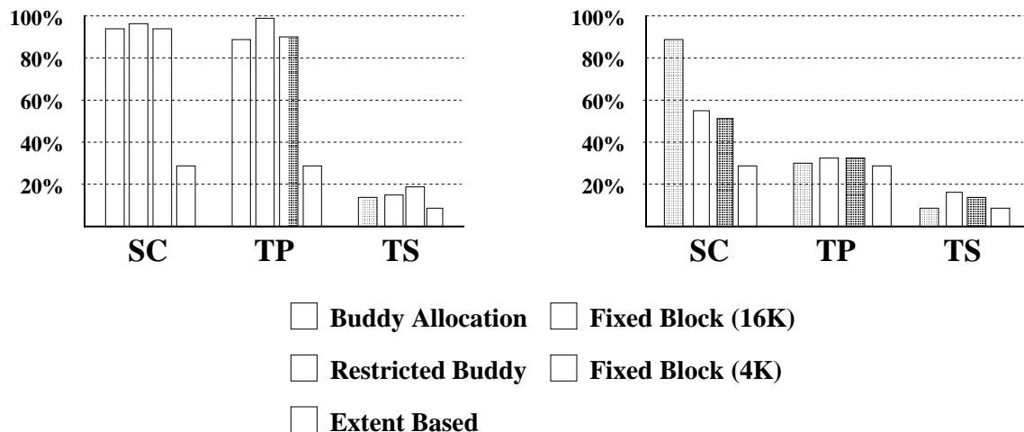
Figure 3-6: Sequential Performance of the Different Allocation Policies.
