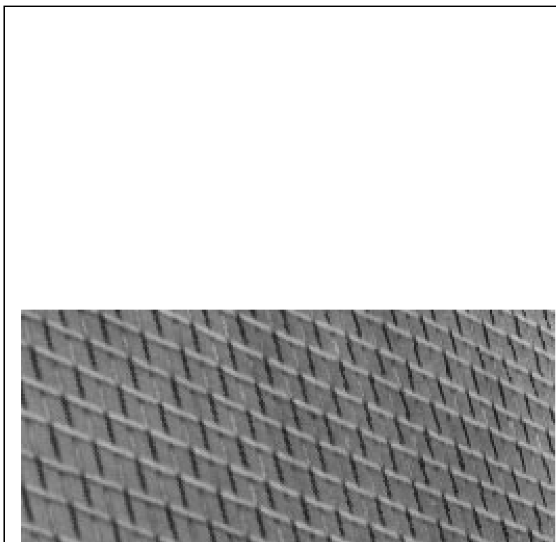
Figure 5: Planar wire texture, \text{slant}=65^\circ , \text{tilt}=-25^\circ , “wire2”.
