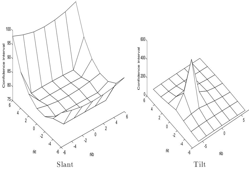
Figure 21: Confidence intervals for slant and tilt as a function of r\kappa_t and r\kappa_b ( r\tau = 0 ).
