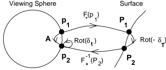
Figure 2: Determining the affine transformation, A , between the texture at point \mathbf{p}_1 and the texture at point \mathbf{p}_2 . F_*(\cdot) is the backprojection map from the viewsphere to the surface. The texture is constant over the image, so the map between \mathbf{P}_1 and \mathbf{P}_2 , the corresponding points on the surface, is just a rotation between the (\mathbf{T}, \mathbf{B}) bases at the two points. \text{Rot}(\delta_t) rotates between the (\mathbf{t}, \mathbf{b}) bases at the points \mathbf{p}_1 and \mathbf{p}_2 . A = \text{Rot}(\delta_t)F_*^{-1}(\mathbf{P}_2)\text{Rot}(-\delta_T)F_*(\mathbf{p}_1) .
