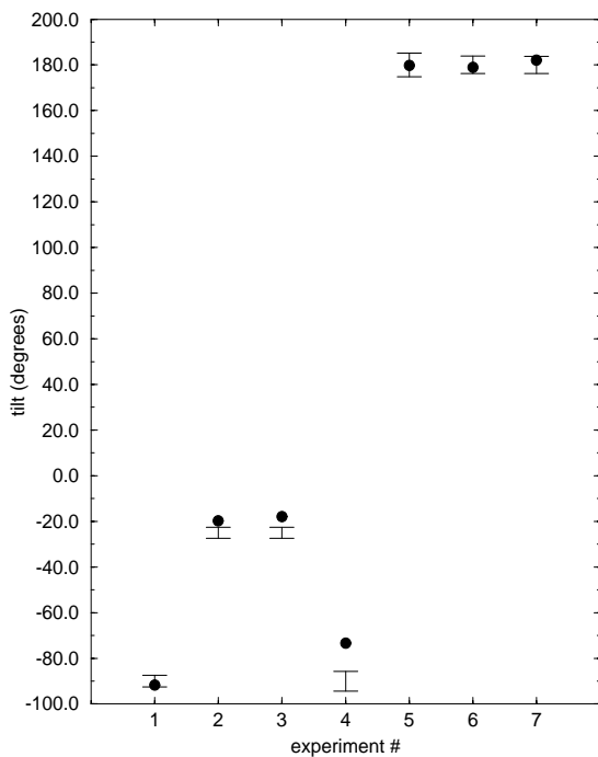
Figure 15: Tilt estimates with confidence intervals.
