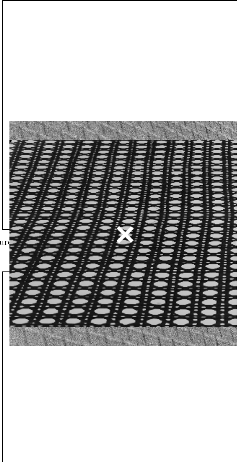
Figure 7: Planar cane texture , \text{slant}=65^\circ , \text{tilt}=-90^\circ , “cane”.
