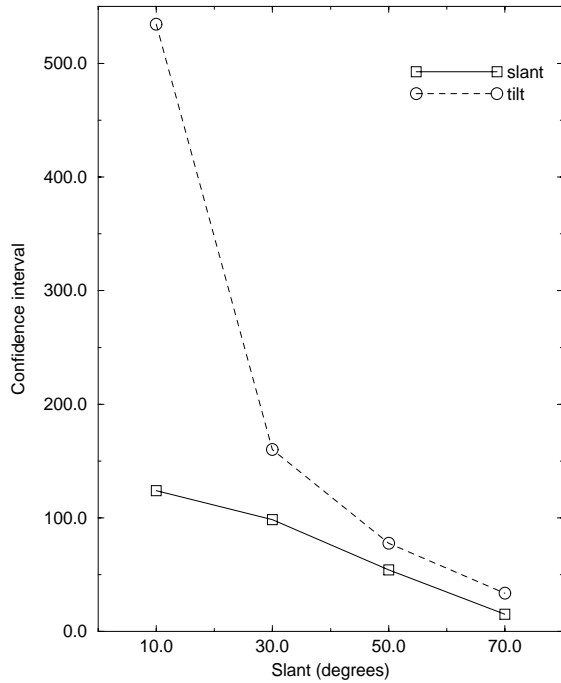
Figure 19: Confidence intervals for slant and tilt as a function of slant for a planar surface.
