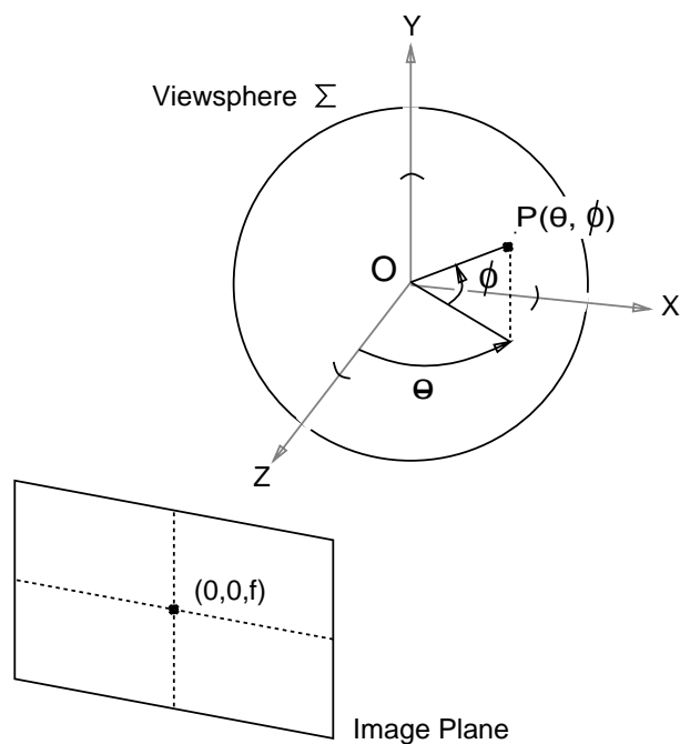
Figure 24: Transforming image plane coordinates into longitude/lattitude spherical coordinates. The optical center is at the origin, O , of the coordinate system. The Z -axis intersects the image plane Z = f at the point (0, 0, f) . Point P = P(\theta, \phi) lies on the surface of the unit viewsphere \Sigma . Point P corresponds to a point Q = (X, Y, f) (not shown) in the image plane, i.e. point P is the intersection of ray \overline{OQ} with the surface of the unit viewsphere. The projection of P onto the Z - X plane makes a counterclockwise angle of \theta with respect to the Z -axis.
