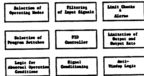
Block diagram of an industrial PID regulator with heuristics (after Astrom, et al)
