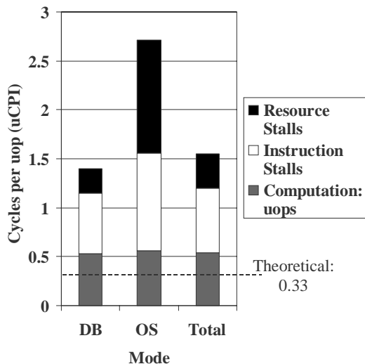
FIGURE 2. Breakdown of cycles per micro-operation ( \mu\text{CPI} ) for base system.
