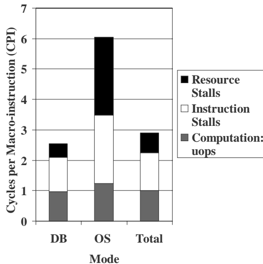
FIGURE 3. Breakdown of cycles per macro-instruction (CPI) for base system.
