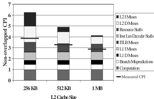
FIGURE 8. Non-overlapped and measured CPI as a function of L2 cache size. Latency from each of the components above is shown as a portion of the bar graph. L1 and L2 hit times are as described in the caption for Table 12, and branch misprediction penalties are as described in the caption for Table 5. L2 cache miss penalties are computed from counter values that measure the number of cycles where data read transactions are outstanding on the bus, and the number of data read transactions.
