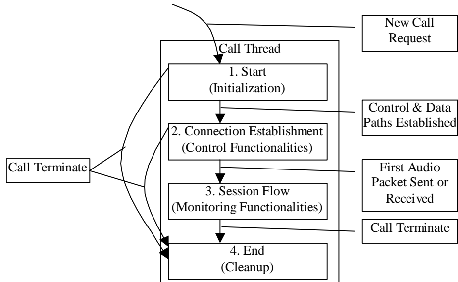
Figure 4.5: A four-state FSM model of a H.323 call.
