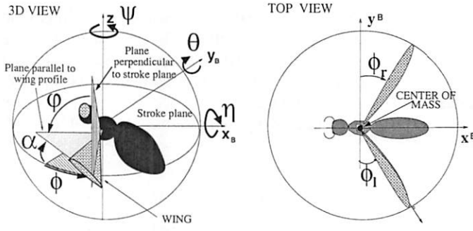
Fig. 3. Definition of wing kinematic parameters: (left) 3D view of insect body and left wing, (right) top view of insect stroke plane.
