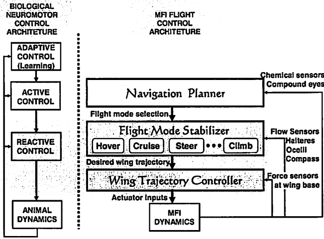
Fig. 2. Design architecture for the control unit of the MFI compared to the neuromotor control architecture present in most animals.
