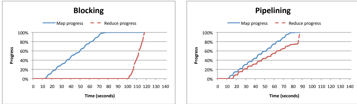
Figure 8: Multi-job Top-100 query over 5.5GB of Wikipedia article text.
