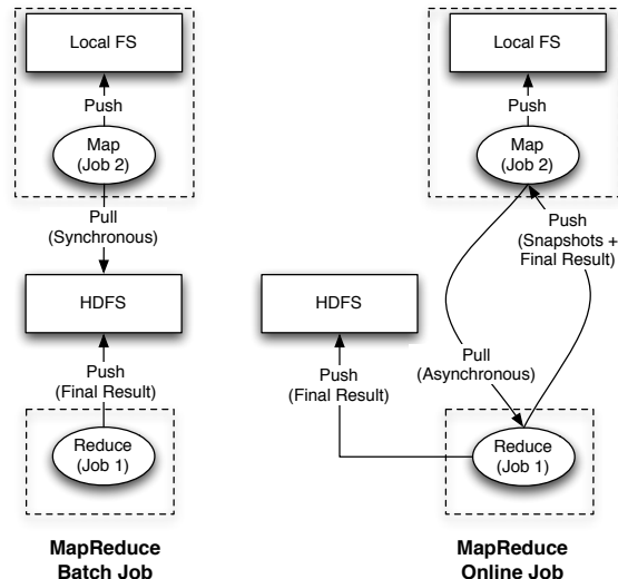
Figure 7: Hadoop dataflow for batch (left) and snapshot (right) processing of MapReduce jobs.
