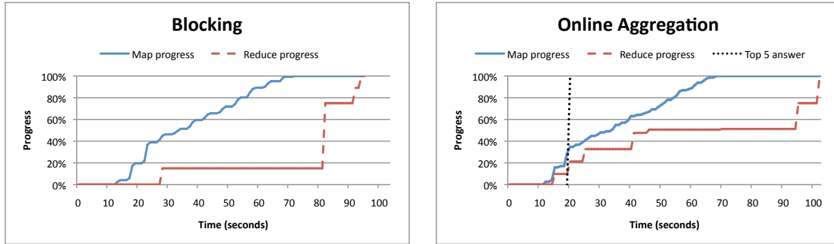
Figure 6: Single job that finds the top 5 words in the 550MB Gutenberg data set. In the graph on the right, the vertical dashed line indicates when online aggregation produces an accurate result.
