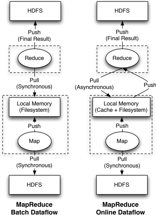
Figure 4: Hadoop dataflow for batch (left) and pipelined (right) processing of MapReduce computations.
