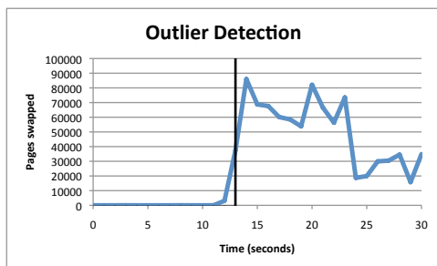
Figure 10: Pages swapped in and out over time on the thrashing host. The vertical line indicates the time at which the alert was sent by the monitoring system.
