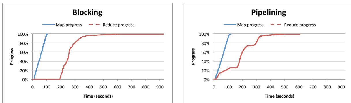
Figure 5: CDF of map and reduce task completion times for a sort job on 5.5GB of text extracted from Wikipedia. The total job runtimes were 927 seconds for blocking, and 610 seconds for pipelining.
