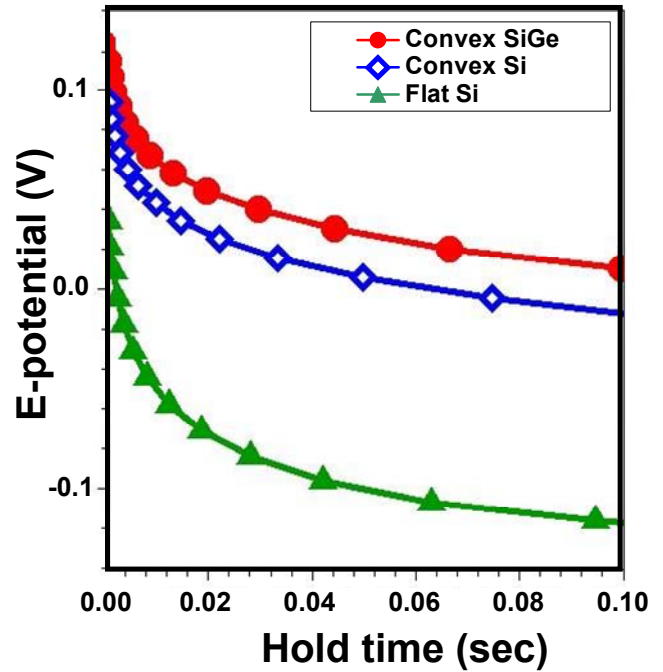
Figure 8. Electrostatic potential at the location in the cell indicated by the black dots in Figure 5 (60 nm below the source/drain surface) vs. Hold time, for cells after a Write “1” operation.
