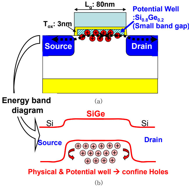
Figure 3. Convex \text{Si}_{1-x}\text{Ge}_x cell design: (a) schematic cross-section. (b) energy band diagram from source to drain region. A deeper potential well for holes is formed, due to the valence band offset between \text{Si}_{1-x}\text{Ge}_x and Si.
