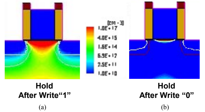
Figure 4. Hole density contour maps for a Flat Si cell. (a) Hold state after Write “1”: many holes are stored underneath the gate. (b) Hold state after Write “0”: holes have been swept away.
