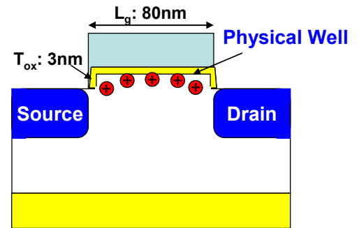
Figure 2. Proposed new convex channel (physical well) design. The increased volume of the charge-storage region enhances retention time.
