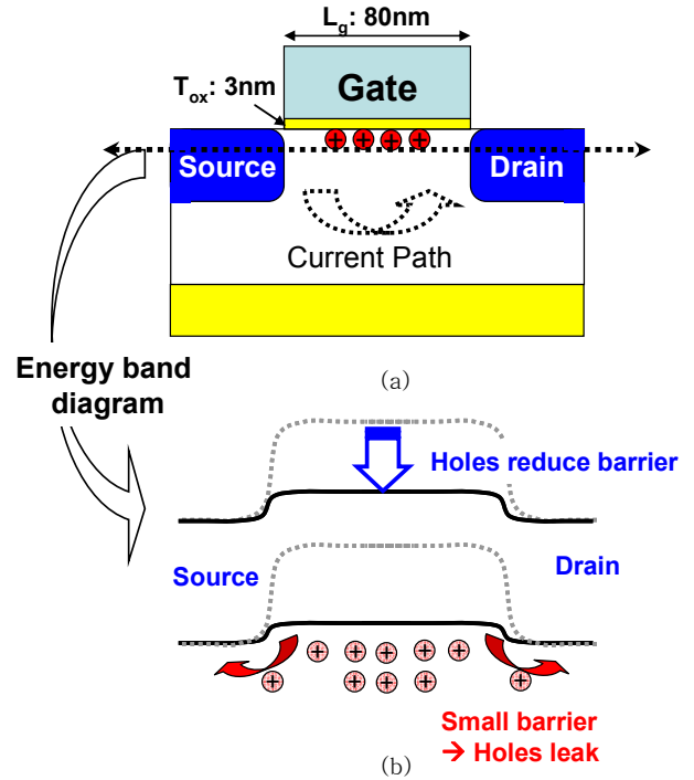
Figure 1. Capacitorless DRAM Generation 2 cell: (a) schematic cross-section. (b) energy band diagram along the channel surface. The dotted lines are for the “0” state in which no holes are stored. The solid lines are for the “1” state in which holes (generated by impact ionization during a Write “1” operation) are stored and hence the potential barrier between the source and body is reduced.
