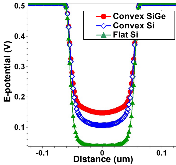
Figure 6. Potential profiles along the x-axis (ref. dotted lines in Figure 5), for cells in the Hold state after a Write “1” operation. The hole potential barrier from the body to the source/drain regions is lowest for the Convex SiGe structure, due to more effective hole storage.
