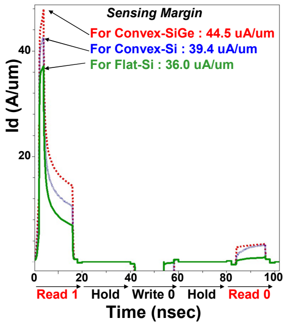
Figure 7. Cell current vs. time for the sequence of operations described in Table I. The sensing margin is defined to be the difference between Read “1” current and Read “0” current.
