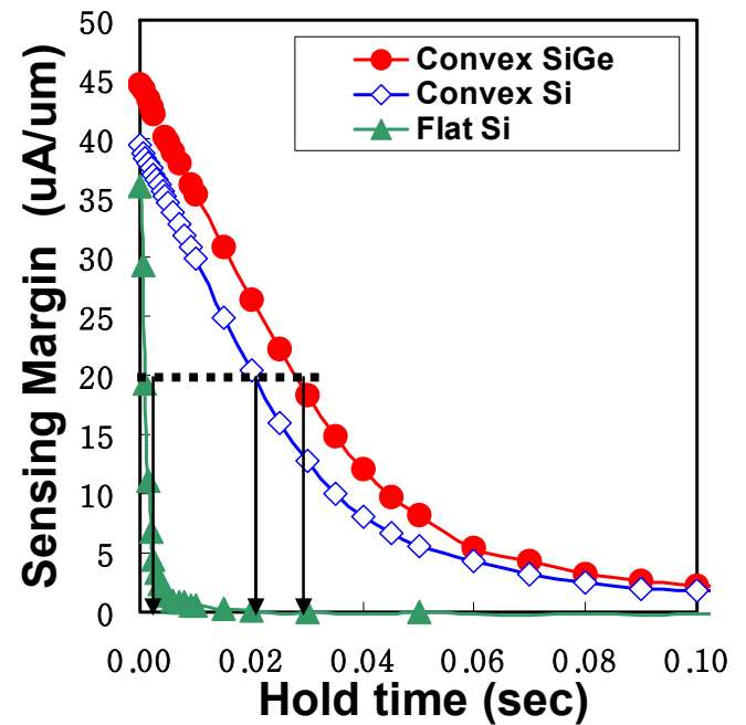
Figure 9. Sensing margin vs. Hold time. The Flat Si cell design shows very short (1ms) retention time. Retention time at 20uA/um is improved to >21ms for the convex cell designs.
