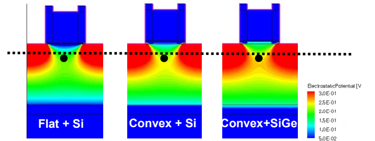
Figure 5. Contour maps of electrostatic potential in the Hold state after a Write “1” operation. The dotted line is shown as a reference for Figure 6, and the large black dots are shown as a reference for Figure 8.
