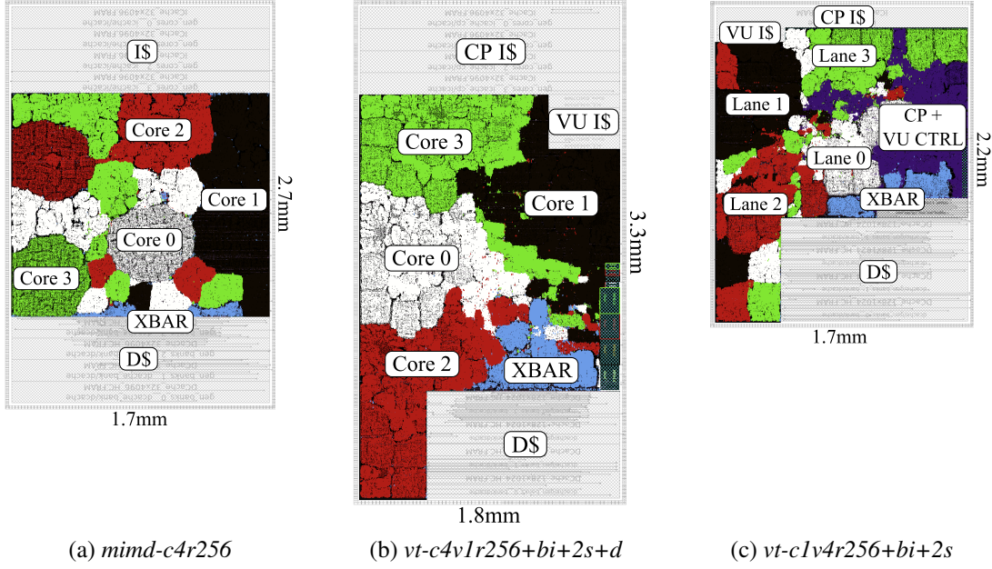
Figure 15: Example VLSI Layouts – ASIC layout designs for mimd-c4 , vt-c4v1r256+bi+2s+d , and vt-clv4r256+bi+2s with individual cores/lanes and the memory crossbar highlighted.
