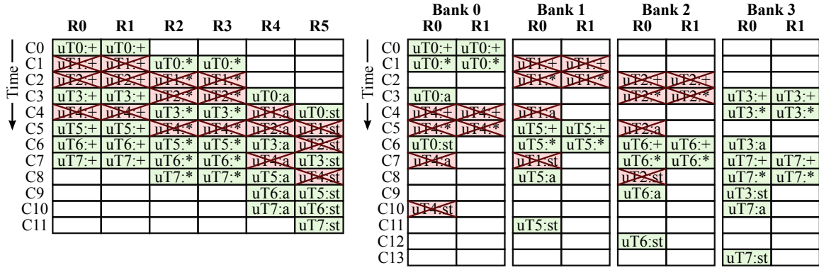
(a) Monolithic 6r3w Vector Register File
