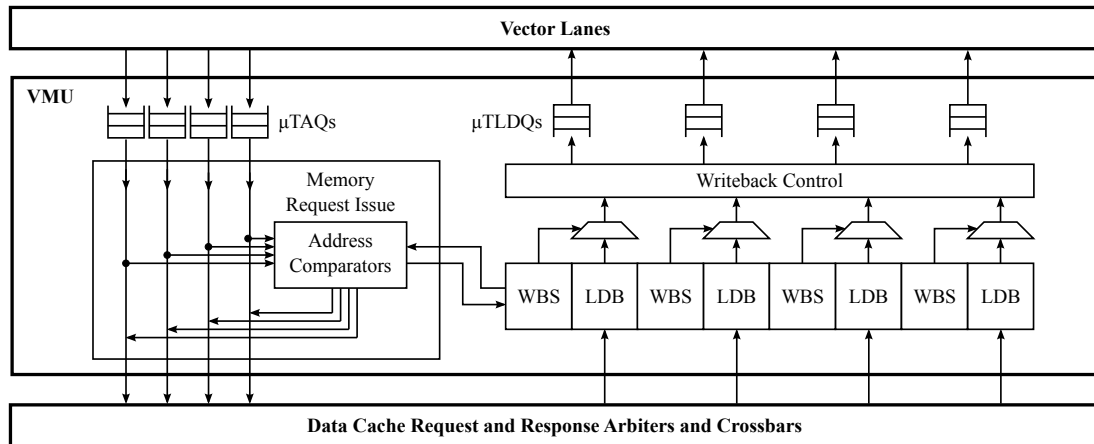
Figure 10: Memory Coalescer Microarchitecture – A memory coalescer for multi-lane VT tiles with four lanes. VMU = vector memory unit, \mu TAQ = \mu T address queue, \mu TLQ = \mu T load data queue, WBS = word/byte select buffer, LDB = load data buffer.
