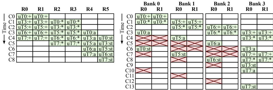
(c) Monolithic VRF with Density-Time Execution
