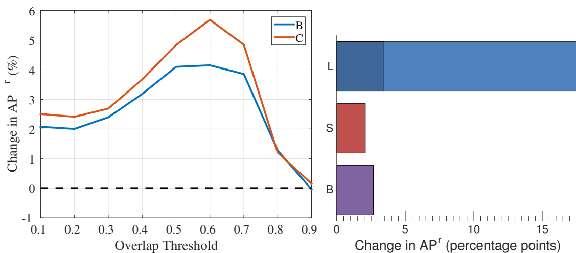
Figure 2.3: Left: The improvement offered by B and C over a range of overlap thresholds. Right: The impact on AP^r of mislocalization, confusion with similar categories and confusion with background.
